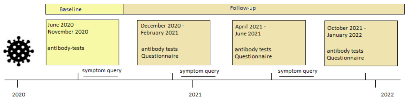
Figure 2. Timeline of data collection. Each participant was invited for four antibody tests: An initial blood test (start June 2020, light yellow) and three follow-up blood tests (dark yellow). In each follow-up blood collection, a questionnaire was completed by the participants.
