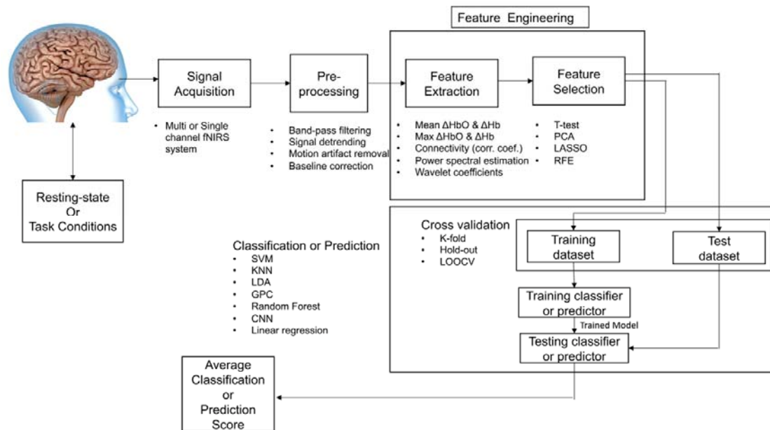
Figure 1. A framework for Classification or Prediction of Clinical Populations or Clinical Conditions using fNIRS
