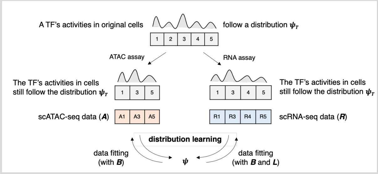
Figure S1. Distribution learning of the hidden TF activity. Within each cell type, the distribution of the hidden variable, TF activity, is identical across cells profiled by ATAC assay and RNA assay from the same sample. MAGICAL iteratively learns the distribution of TF activity and fits both chromatin accessibility and gene expression data together with other model parameters.
