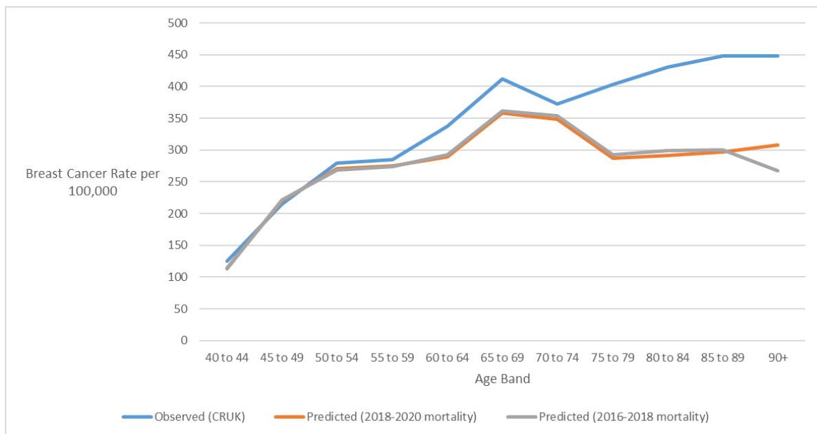
Figure 1: Predicted and Observed Age-specific incidence rate
