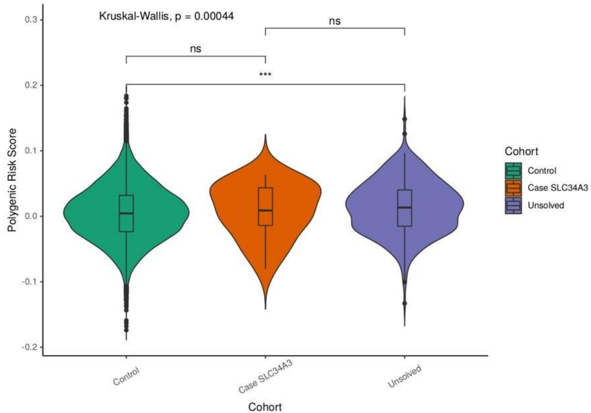
Supplementary figure 3 - Violin and boxplot showing the polygenic risk score (PRS) distributions between controls (those with qualifying SLC34A3 variants removed), cases with qualifying SLC34A3 variants and unsolved patients who have neither a reportable variant or a qualifying SLC34A3. The means of the three PRS were compared with a Kruskal-Wallis test ( p=4.4 \times 10^{-04} ) with the signal being driven by the difference between unsolved cases and controls (paired Willcox =3.1 \times 10^{-04} ). *** = statistical significance, ns = no significant difference
