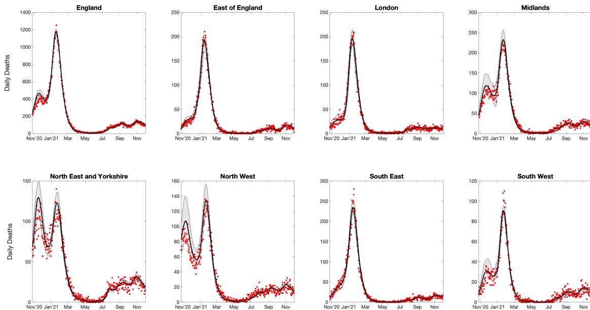
Fig. S6: Comparison between models and data for regional deaths. We depict the data as solid black dots and results from the model simulations in red- no attempt is made to add the appropriate noise to these raw deterministic simulations. The solid lines corresponds to mean values and the shaded area shows the 95% prediction interval (i.e. it contains 95% of all predictions at each point in time).
