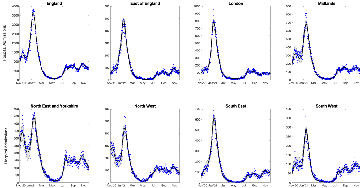
Fig. S5: Comparison between models and data for regional hospital admissions. We depict the data as solid black dots and results from the model simulations in blue - no attempt is made to add the appropriate noise to these raw deterministic simulations. The solid lines corresponds to mean values and the shaded area shows the 95% prediction interval (i.e. it contains 95% of all predictions at each point in time).
