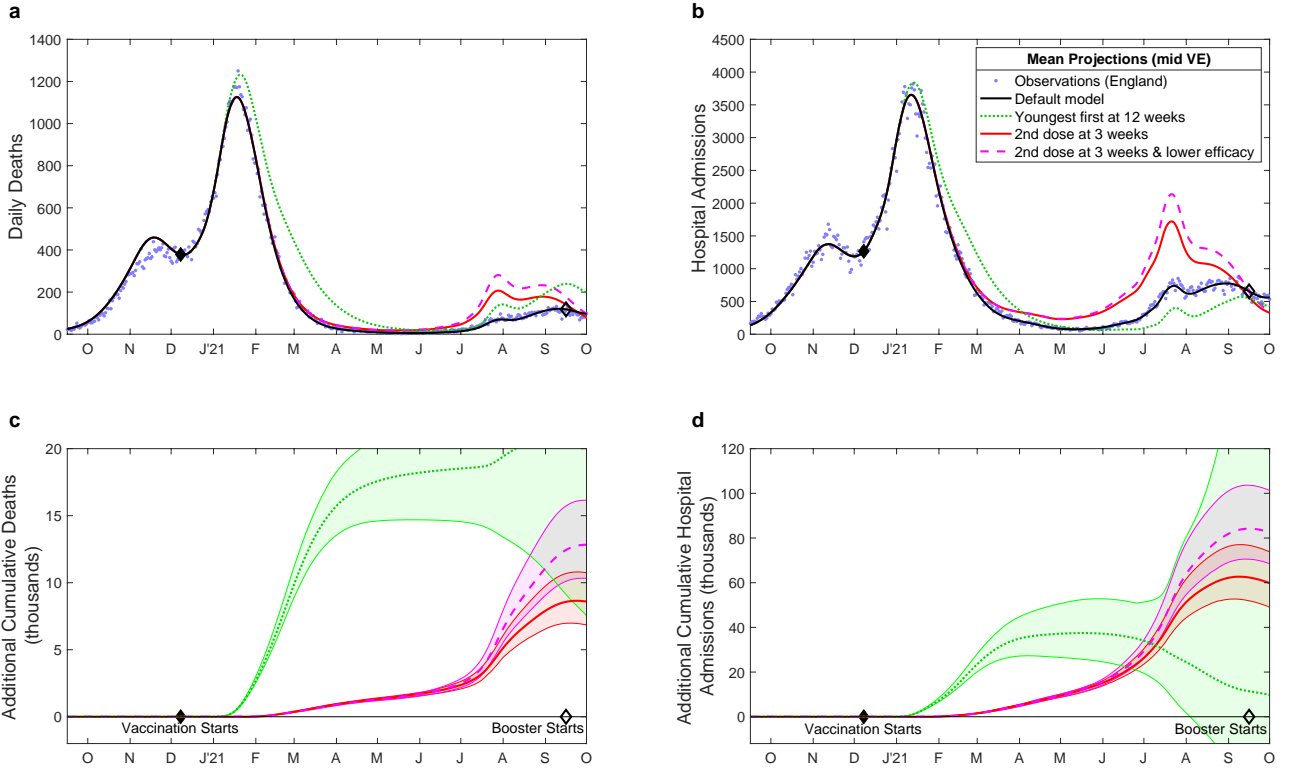
Fig. S7: Projected changes in daily deaths (a, c) and hospital admissions (b, d) with differing vaccination patterns. This is the equivalent of Fig. 1 in the main text, but uses the mid-point estimates of vaccine efficacy from the SAGE Vaccine Effectiveness Expert Panel subgroup [9].
