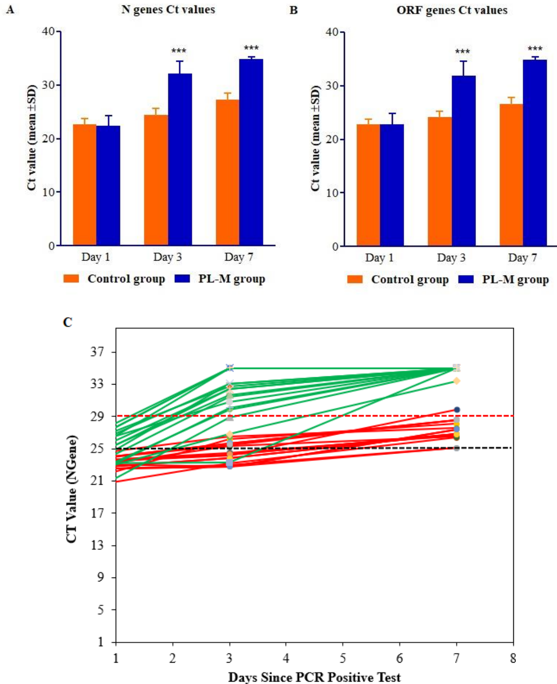
Figure 1. RT-PCR profiles of (A) the N gene, (B) the ORF gene, and (C) change in Ct value of individual subject in the placebo group (n=17) and PL-M group (n=17). RT-PCR profiles of N and ORF genes detected SARS-CoV-2 in COVID-19 patients on days 1, 3 and 7. On day 3, 82.35% of participants in the PL-M group had cycle counts for the N gene above the cut-off value of 29, while on day 7 all participants had cycle counts above the cut-off value. The majority of participants (94.12%) in the placebo group had cycle counts for the N gene below
