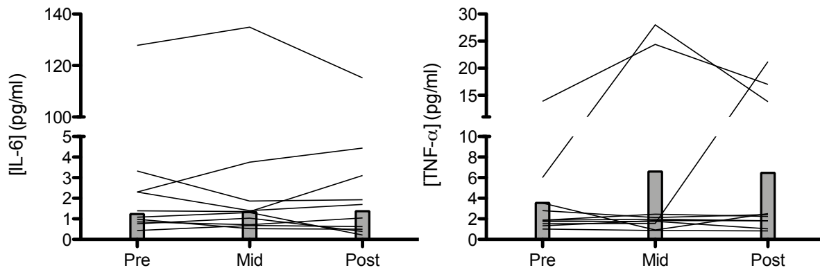
Supplementary Figure 2. Circulating cytokine levels. The grey lines denote data for individual participants at each time point. The grey bars demonstrate the group median at each time point. A single participant, IBDM-09, had abnormally high levels of IL-6 (>110 pg/mL) for all three assessment points; however, Friedman test results were unchanged when this participant was excluded.
