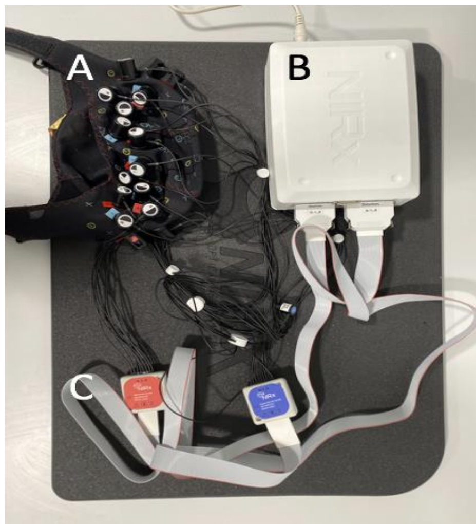
Figure 2: fNIRS acquisition system. A. fNIRS cap. B. NIRSport2 system. C, Optodes
