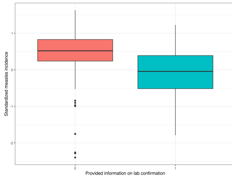
Supplementary Figure 9. Distribution measles incidence values used for covariates of country-years for studies providing information on laboratory confirmation of cases (1) versus not providing information on laboratory confirmation of cases (0).
