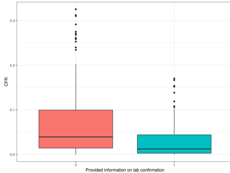
Supplementary Figure 8. Distribution of CFR values for studies providing information on laboratory confirmation of cases (1) versus not providing information on laboratory confirmation of cases (0).
