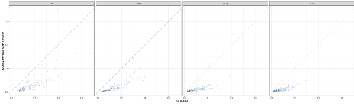
Supplementary Figure 12. CFR estimates from framework using all studies versus only studies providing definition of death attributable to measles, for select years.
