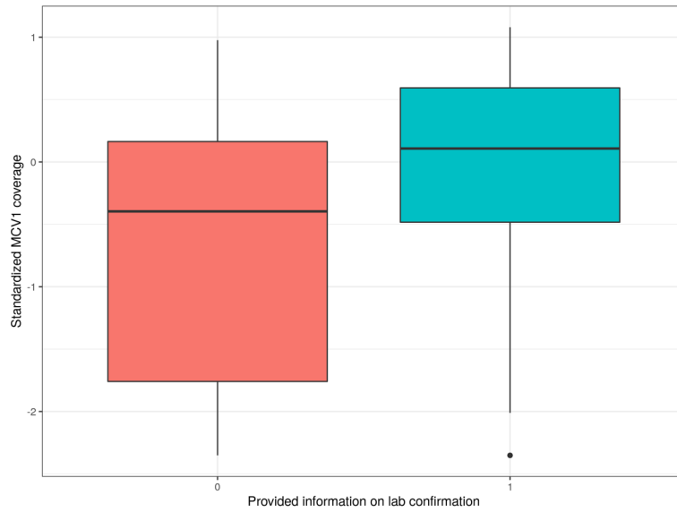
Supplementary Figure 10. Distribution MCV1 coverage values used for covariates of country-years for studies providing information on laboratory confirmation of cases(1) versus not providing information on laboratory confirmation of cases (0).
