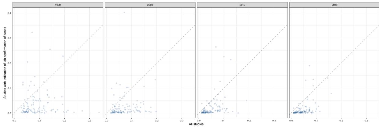
Supplementary Figure 11. CFR estimates from framework using all studies versus only studies providing information on laboratory confirmation of cases, for select years.
