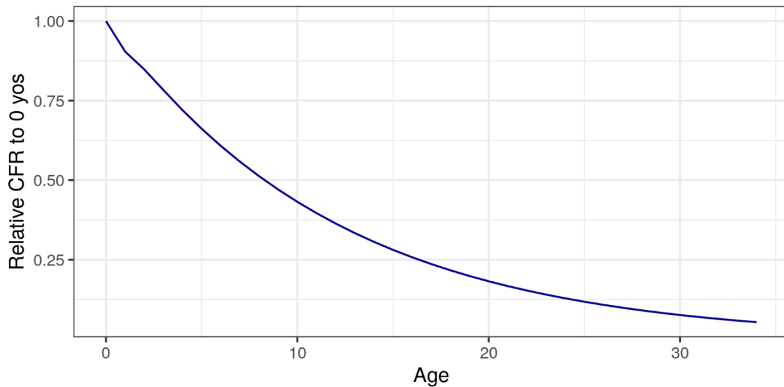
Supplementary Figure 2. Relative age pattern from first-stage model with 2 internal knots.
