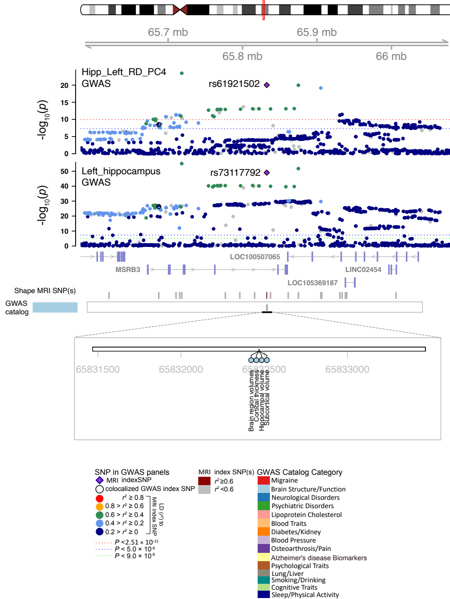
Fig. S16 Selected genetic locus that were associated with both shape features and other complex traits.
