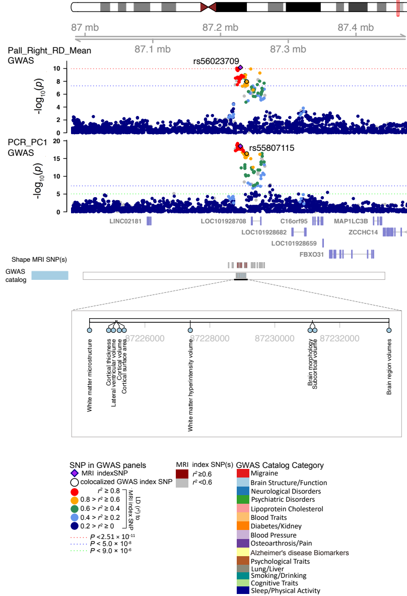
Fig. S29 Selected genetic locus that were associated with both shape features and other complex traits.
