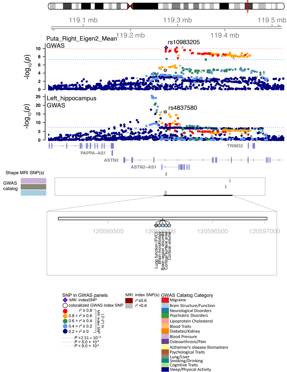
Fig. S12 Selected genetic locus that were associated with both shape features and other complex traits.
