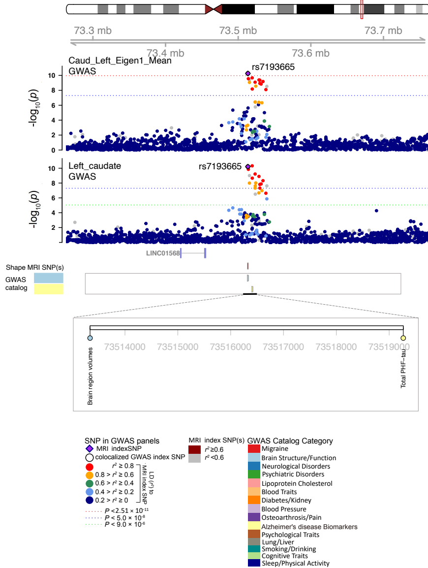
Fig. S20 Selected genetic locus that were associated with both shape features and other complex traits.
