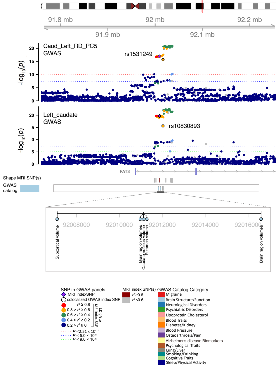
Fig. S13 Selected genetic locus that were associated with both shape features and other complex traits.
