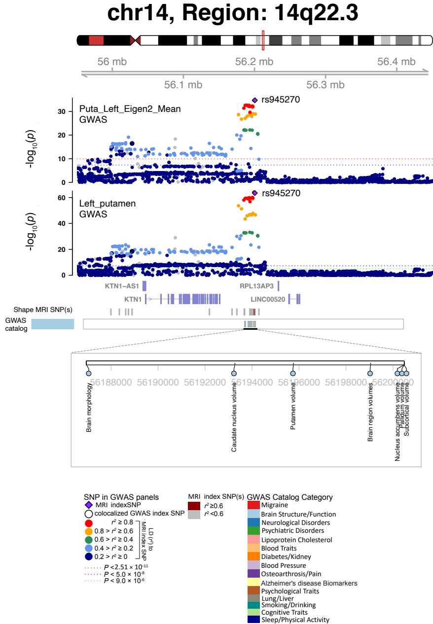
Fig. S19 Selected genetic locus that were associated with both shape features and other complex traits.
