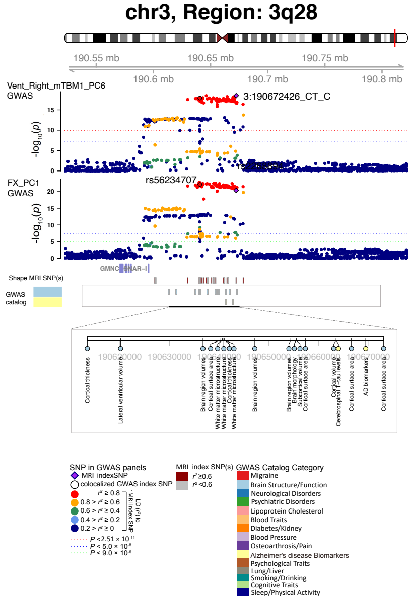
Fig. S23 Selected genetic locus that were associated with both shape features and other complex traits.
