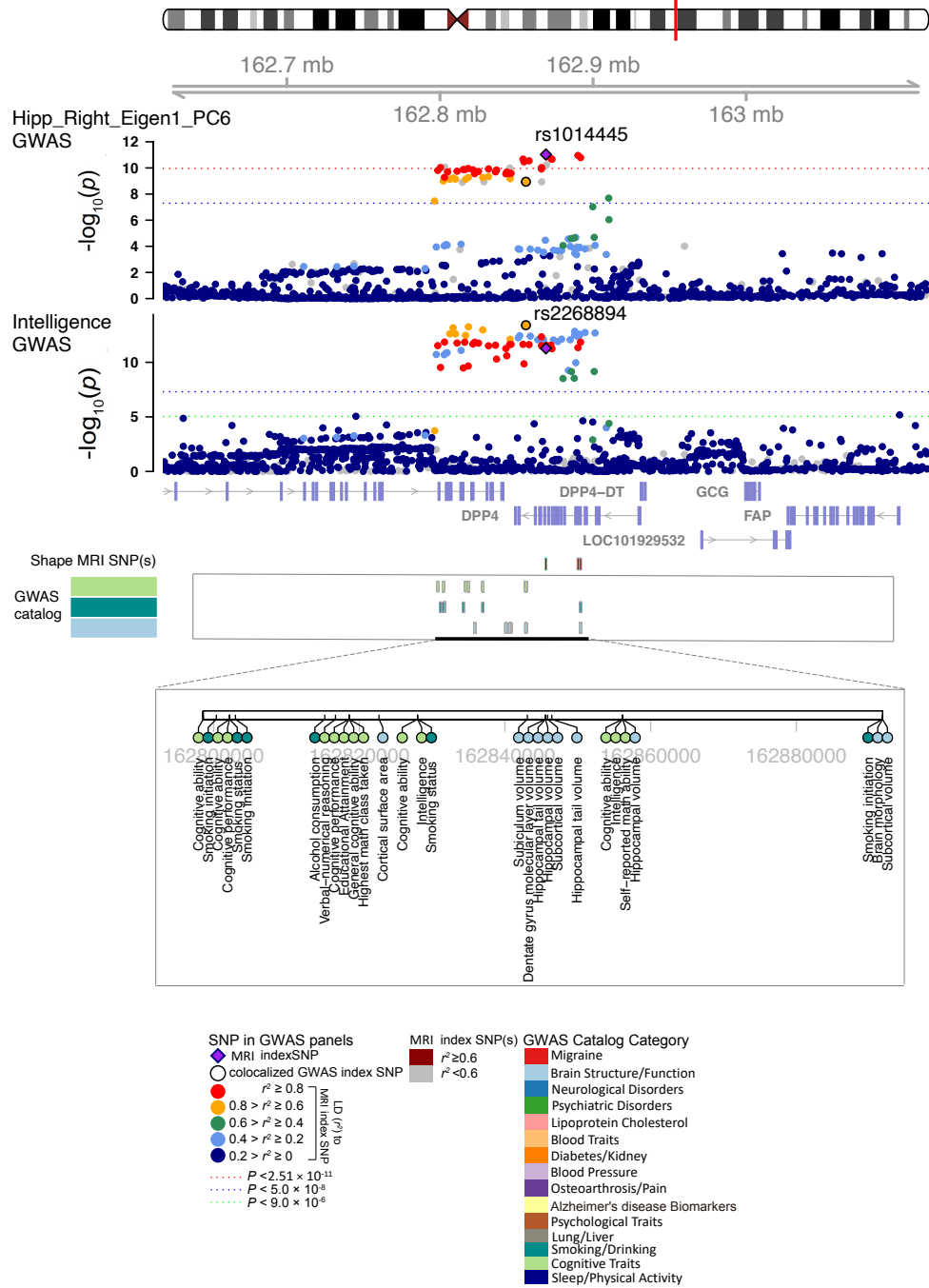
Fig. S34 Selected genetic locus that were associated with both shape features and other complex traits.
