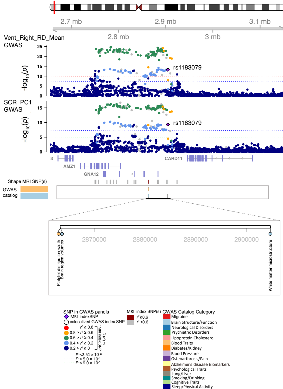
Fig. S26 Selected genetic locus that were associated with both shape features and other complex traits.
