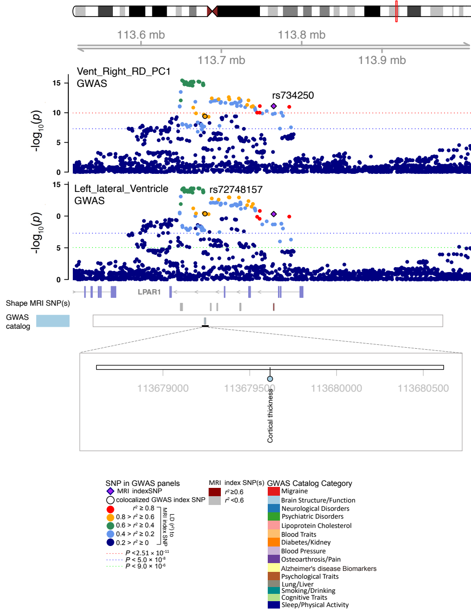
Fig. S11 Selected genetic locus that were associated with both shape features and other complex traits.
