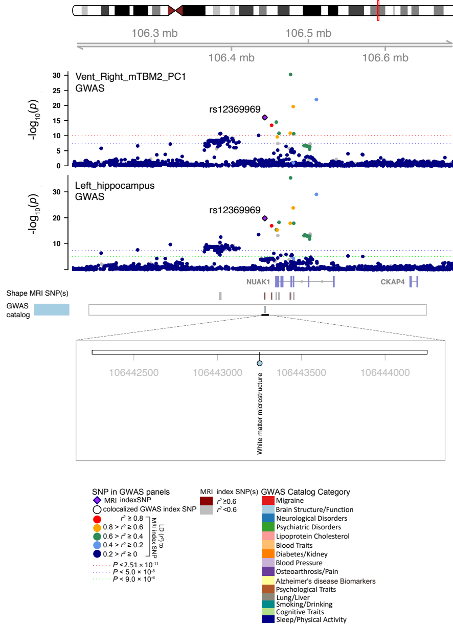
Fig. S17 Selected genetic locus that were associated with both shape features and other complex traits.
