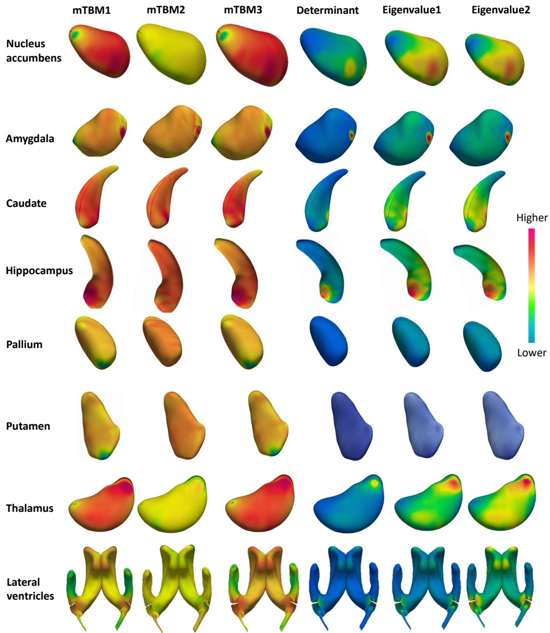
Fig. S2 Illustration of the structures and shape features. We illustrate the spatial pattern of 6 shape statistics (mTBM1, mTBM2, mTBM3, determinant, eigenvalue1, and eigenvalue2) in the vertex-wise maps of 8 ventricular and subcortical structures. These maps were generated by averaging the data from 500 randomly selected UKB subjects.
