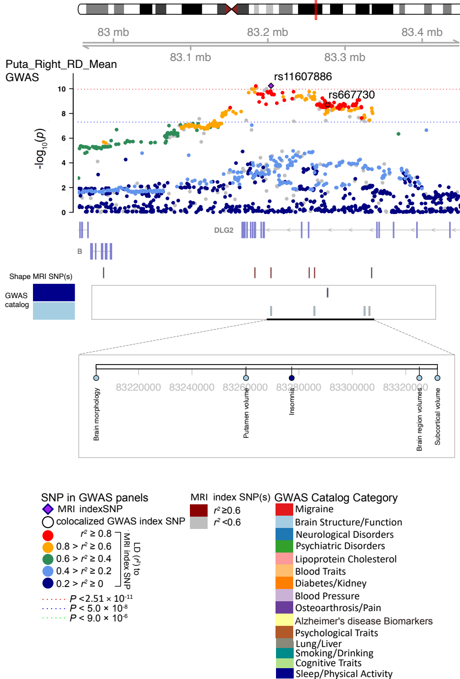
Fig. S38 Selected genetic locus that were associated with both shape features and other complex traits.
