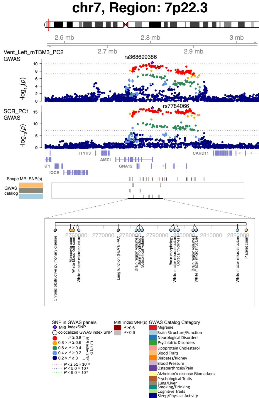
Fig. S27 Selected genetic locus that were associated with both shape features and other complex traits.
