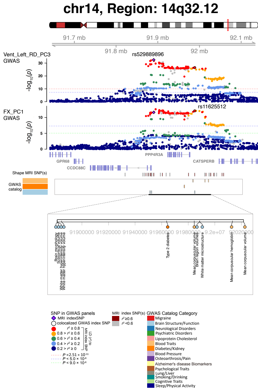
5 Fig. S28 Selected genetic locus that were associated with both shape features and other complex traits.
