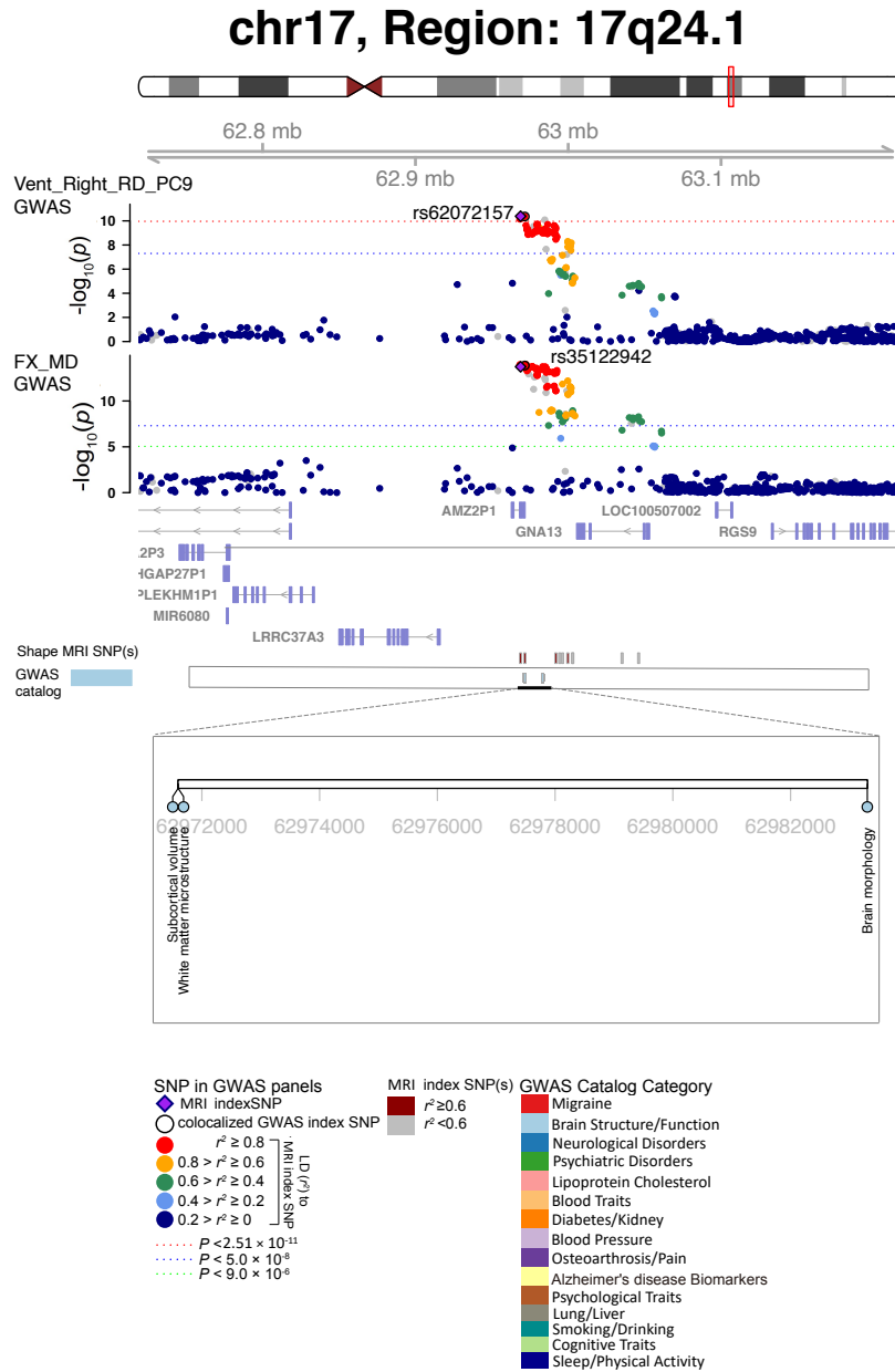
Fig. S21 Selected genetic locus that were associated with both shape features and other complex traits.
