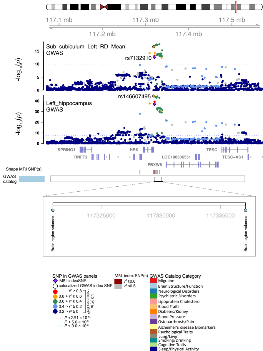
Fig. S18 Selected genetic locus that were associated with both shape features and other complex traits.
