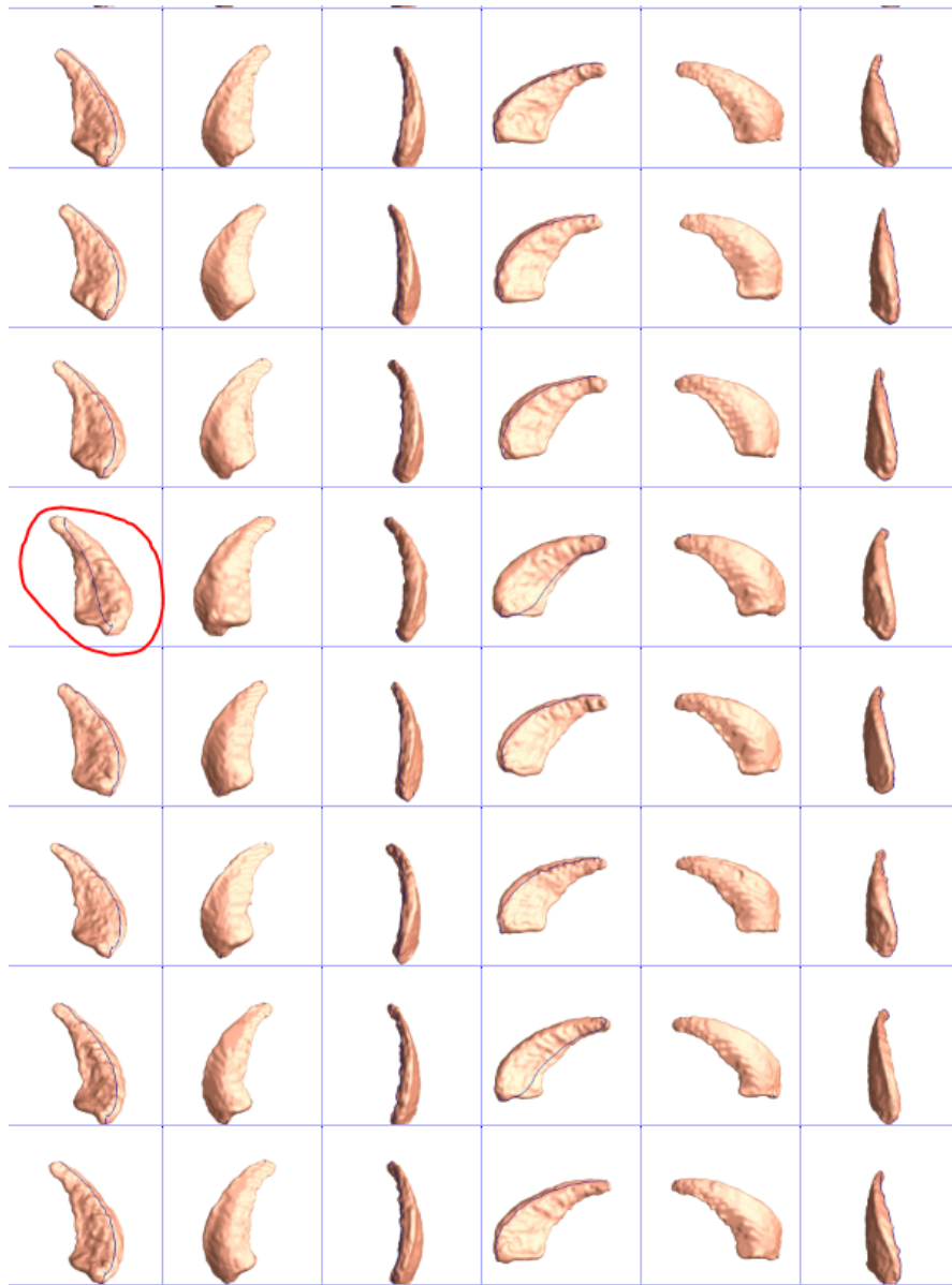
Fig. S42 Example of surface registration quality check.
