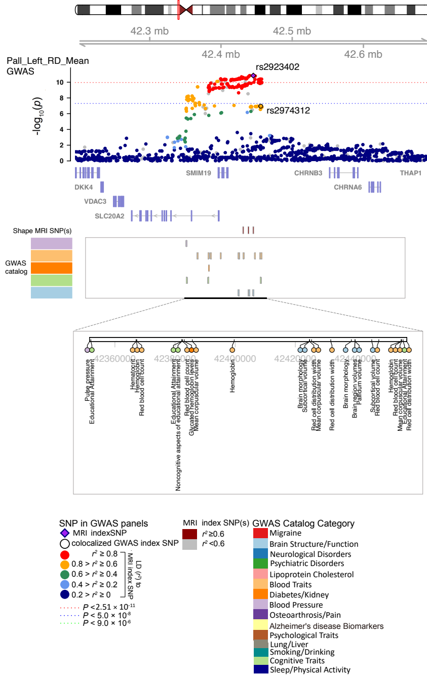
Fig. S36 Selected genetic locus that were associated with both shape features and other complex traits.
