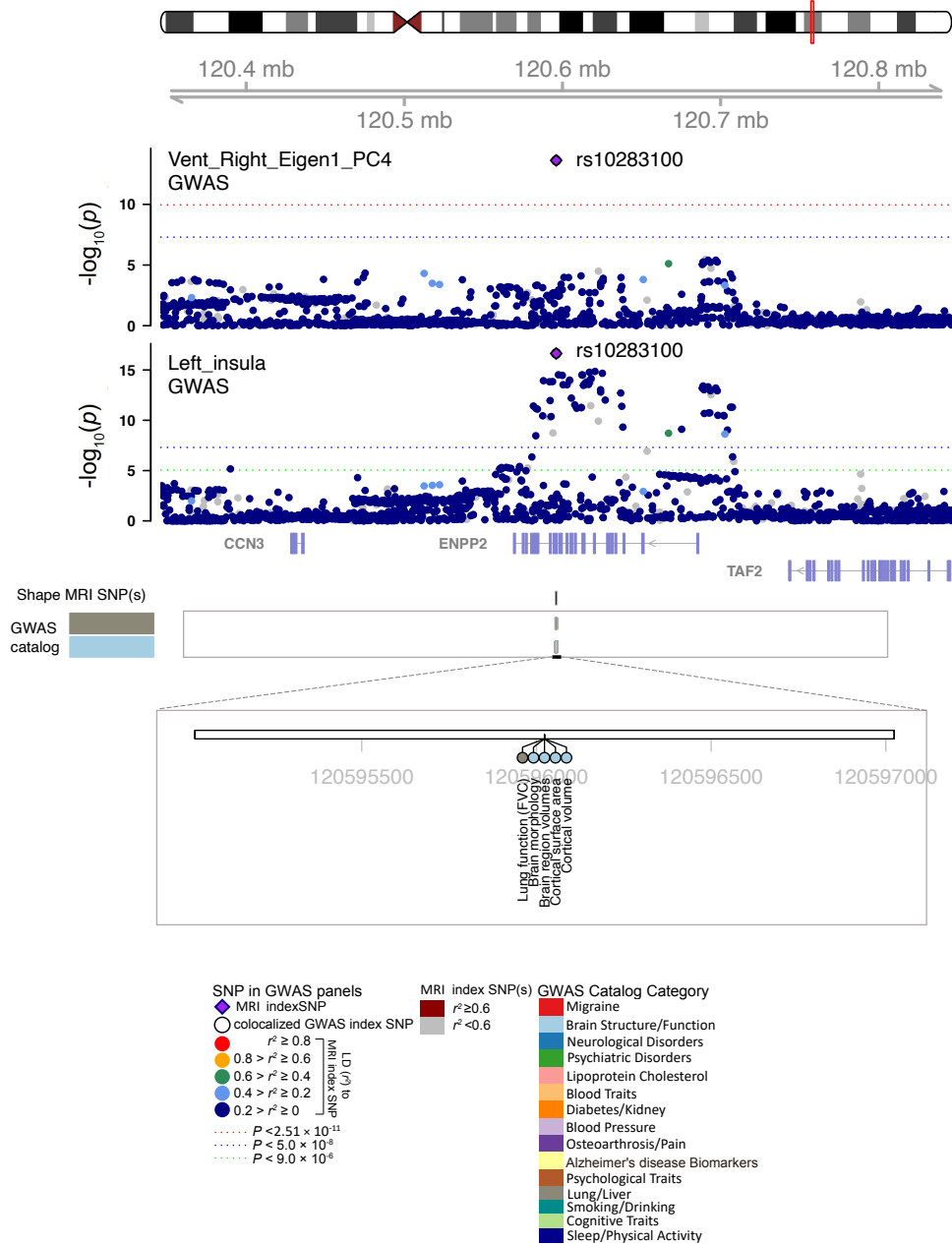
Fig. S10 Selected genetic locus that were associated with both shape features and other complex traits.
