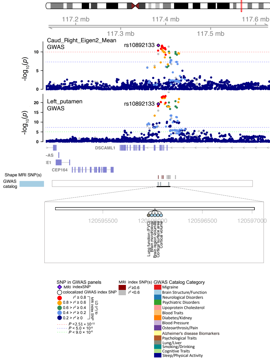
Fig. S15 Selected genetic locus that were associated with both shape features and other complex traits.
