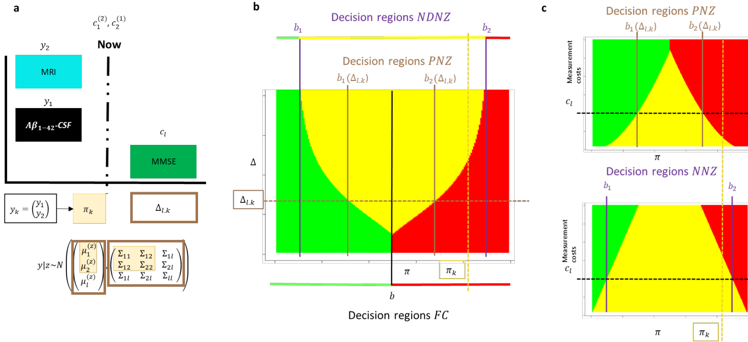
Fig. S1: Visualization of the prospective neutral zone classifier (a) Situation in which already a MRI ( y_1 ) and A\beta_{1-42} -CSF ( y_2 ) measure were assessed ( y_k vector containing both measures) and the classification task consist of either choosing one of the possible classes (MCI-stable or MCI converter) in case there is enough evidence or postpone the decision and stay neutral ( NZ ) to additionally assess the MMSE ( y_l ) and then decide for one of the classes. The classification outcome depends on the misclassification costs c_1^{(2)}, c_2^{(1)} and the measurement cost c_l for y_l , the current evidence \pi_k and the prospective discriminability \Delta_{l,k} (given by the conditional distributions y_l|z, y_k ). (b) Visualizations of decision regions for constant decision costs. In contrast to the forced-choice (FC, black line) and the non-prospective neutral zone classifier (NPNZ, purple lines) for the prospective neutral zone classifier (PNZ) the amount of leftover diagnosis-relevant information in y_l (quantified by \Delta_{l,k} ) determines the amount of evidence given by the assessment y_k (quantified by \pi_k ) that is needed to make a finite decision without assessing y_l ( \pi_k < b_1(\Delta_{l,k}) or \pi_k > b_2(\Delta_{l,k}) ). For the prospective neutral zone classifier, the prediction outcome for a given value of \Delta_{l,k} is displayed by the coloured areas, the boundaries between the green and yellow area is b_1(\Delta_{l,k}) and the one between the yellow and red area is b_2(\Delta_{l,k}) (c) For fixed misclassification costs c_1^{(2)}, c_2^{(1)} and prospective discriminability \Delta_{l,k} the decision boundaries for the PNZ- and DNZ classifiers are displayed as a function of the measurement costs
