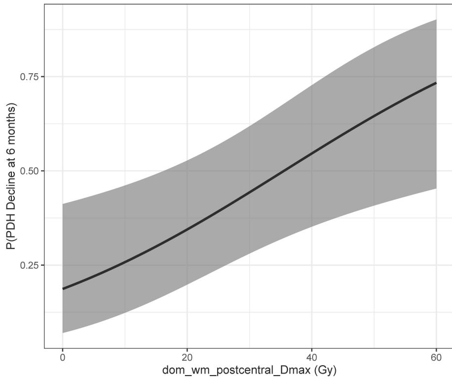
Fig S3: Logistic NTCP curve for the single term model produced using automated bootstrapped regression
