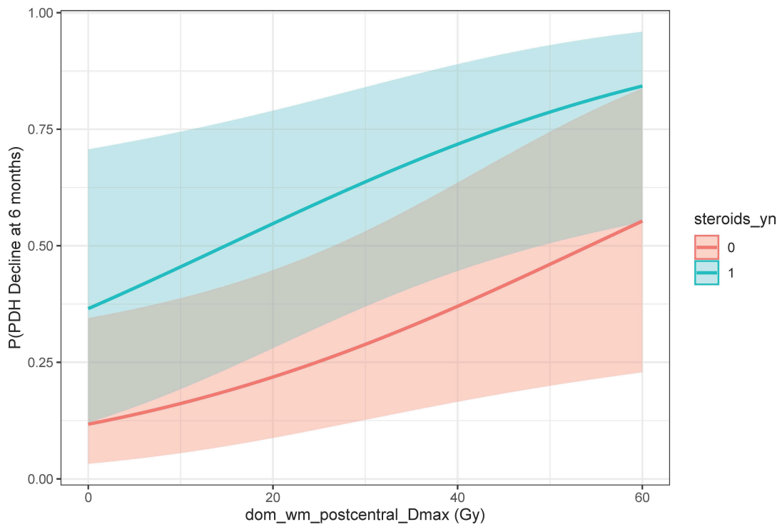
Fig S4: Logistic NTCP curve for the two term model produced using LASSO (coefficients here are unregularized)
