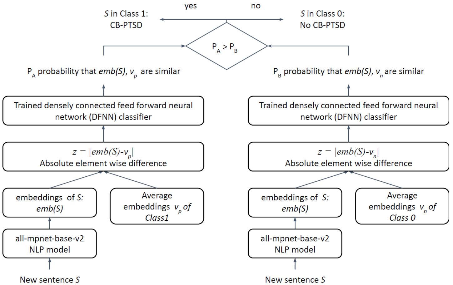
Supplemental Figure 2. Identification of childbirth-related post-traumatic stress disorder (CB-PTSD) using the developed model by classification of a new narrative sentence ( S ) that was not used for model training.
