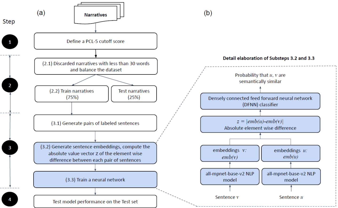
Supplemental Figure 1. Steps of the machine learning classifier model development for the identification of maternal childbirth-related post-traumatic stress disorder (CB-PTSD). (a) Left panel: An illustration summary of the four steps of the model. (b) Right panel: Training a neural network to identify pairwise sentence similarity.
