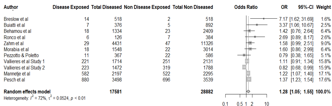
Figure 2: Forest Plot showing the pooled association between exposure to welding fumes and lung cancer
