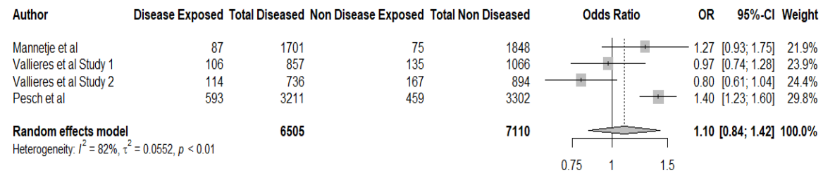
Figure 4: Forest Plot showing the pooled association between arc fume exposure and lung cancer
