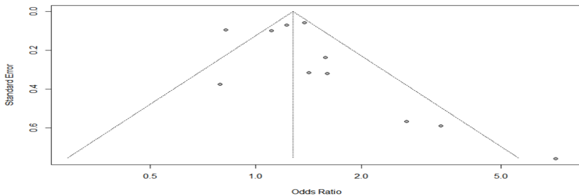
Figure 10: Contour-Enhance Funnel Plot
