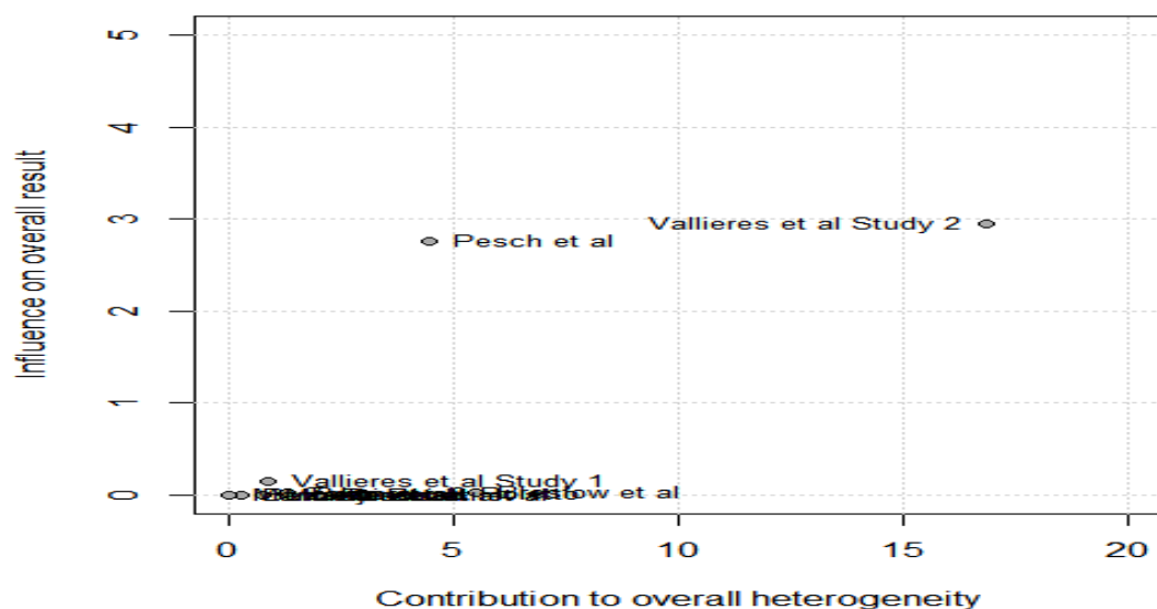
Figure 6: Baujat plat showing outliers among the studies included
