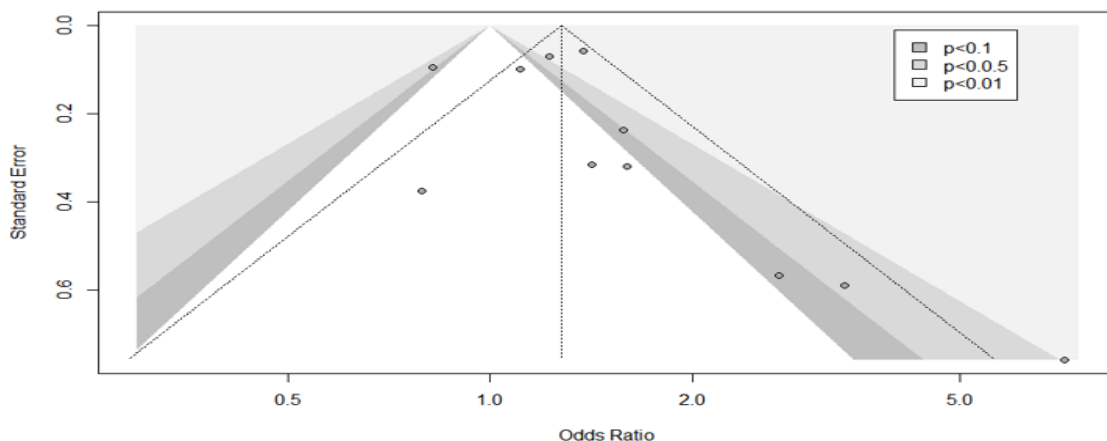
Figure 10: Contour-Enhance Funnel Plot
