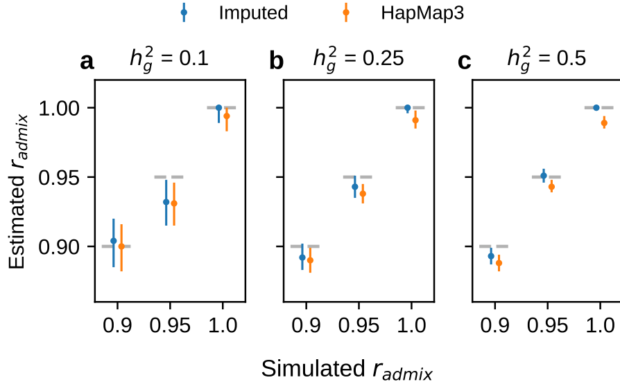
Figure 2: Results of genetic correlation r_{\text{admix}} estimation in genome-wide simulations. Simulations were based on 17K PAGE individuals and 6.9M genome-wide variants with MAF > 0.5% in both ancestries. We fixed the proportion of causal variants p_{\text{causal}} as 0.1%, varied genome-wide heritability h_g^2 = 0.1, 0.25, 0.5 , genetic correlation r_{\text{admix}} = 0.90, 0.95, 1.0 . For each simulated genetic architecture, we plot the mode and 95% credible interval based on the meta analysis across 100 simulations (Methods). Numerical results are reported in Table S1. Numerical results for other p_{\text{causal}} are reported in Table S2.
