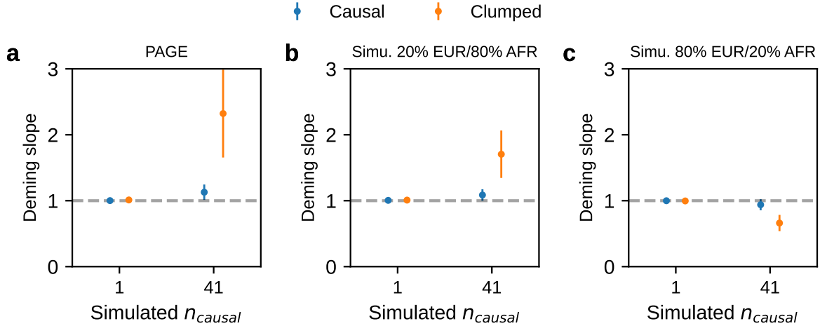
Figure S8: Simulation results in PAGE data set and simulated genotype data sets with varying ancestry proportion. We evaluated the bias of Deming slope ( \beta_{\text{eur}}^{(m)} \sim \beta_{\text{afr}}^{(m)} ) observed in Figure 6 by performing simulations on 3 genotype data sets: (a) PAGE data set of 17,299 individuals with \sim 20\% European and \sim 80\% African ancestry proportions. (b) simulated genotype data set of 20,000 individuals with 20\% European and 80\% African ancestry proportions. (c) simulated genotype data set of 20,000 individuals with 80\% European and 20\% African ancestry proportions. Simulated genotype data was generated as follows: first, we simulated the local ancestries for each SNP and individual using a Poisson process parametrized by the recombination rate and genetic distance; second, we used the phased genotype segment from a random individual in 1,000 Genomes with the corresponding ancestry (European / African) as the genotype for each simulated local ancestry segment. Such simulation method preserves the realistic local ancestry segment length distribution, MAF and LD structure for the generated genotypes. To simulate the phenotype, we randomly selected 100 regions each spanning 20 Mb on chromosome 1. For each region, we either simulated n_{\text{causal}} = 1 causal variant at the middle of the region, or simulated n_{\text{causal}} = 41 equally spaced across 20 Mb (on average 2 causal variant per Mb); these causal variants had same causal effects across local ancestries and each causal variant was expected to explain a fixed amount of heritability ( 0.6\% ) (we simulated a large heritability to better simulate the bias due to different ancestry proportions). 95% confidence intervals were based on 100 random sub-samplings with each sample consisted of 500 SNPs. We determined that biases from PAGE and simulated genotype data with 20\% European / 80\% African ancestries were both upward and biases from simulated genotype data with 80\% European / 20\% African ancestries were downward. Therefore, we determined the biases were due to imbalanced ancestry proportions ( \sim 20\% European and \sim 80\% African ancestries) in PAGE data. Numerical results are reported in Table S13.
