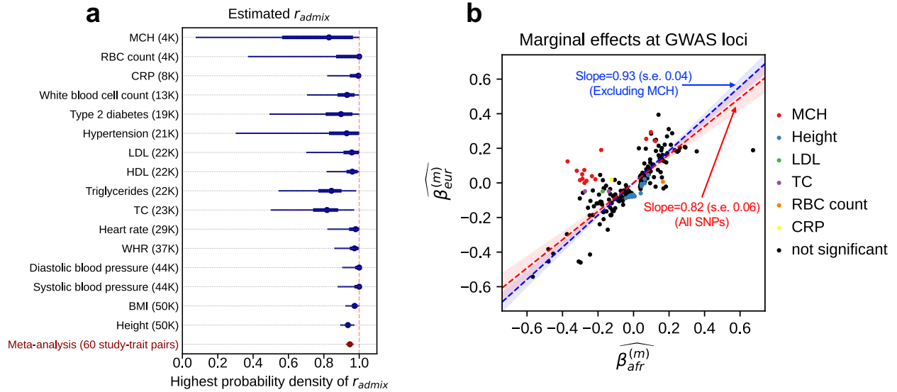
Figure 3: Similarity of causal effects and marginal effects across local ancestries meta-analyzed across PAGE, UKBB, AoU. (a) We plot the trait-specific estimated r_{admix} for 16 traits. For each trait, dots denote the estimation modes; bold lines and thin lines denote 50% / 95% highest density credible intervals, respectively. Traits are ordered according to total number of individuals included in the estimation (shown in parentheses). These traits are selected to be displayed either because they have the largest total sample sizes, or because the associated SNPs of these traits exhibit heterogeneity in marginal effects (see the panel on the right). We also display the meta-analysis results across all 38 traits (60 study-trait pairs). (b) We plot the ancestry-specific marginal effects for 217 GWAS significant clumped trait-SNP pairs across 60 study-trait pairs. Trait-SNP pairs with significant heterogeneity in marginal effects by ancestry ( p_{HET} < 0.05/217 via HET test) are denoted in color (non-significant trait-SNP pairs denoted as black dots). Numerical results are reported in Table S7. Deming regression slopes of \widehat{\beta}_{eur}^{(m)} \sim \widehat{\beta}_{afr}^{(m)} are provided either for all 217 SNPs, or for 193 SNPs after excluding 24 MCH-associated SNPs. MCH, mean corpuscular hemoglobin. RBC, red blood cell. CRP, C-reactive protein. LDL, low density lipoprotein cholesterol. HDL, high density lipoprotein cholesterol. TC, total cholesterol. BMI, body mass index. WHR, waist to hip ratio. Numerical results are provided in Tables 1 and S7.
