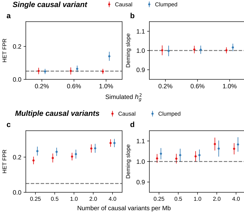
Figure 6: Mis-calibration of HET test and Deming regression slope in simulations with r_{\text{admix}} = 1 . (a-b) Simulations with single causal variant. Each causal variant had the same causal effects across local ancestries and each causal variant explained a fixed amount of heritability (0.2%, 0.6%, 1.0%). (a) False positive rate (FPR) of HET test. (b) Deming regression slope of \widehat{\beta}_{\text{eur}}^{(m)} \sim \widehat{\beta}_{\text{afr}}^{(m)} . Numerical results are reported in Table S9. (c-d) Simulation with multiple causal variants. We simulated different level of polygenicity, such that on average there were approximately 0.25, 0.5, 1.0, 2.0, 4.0 causal variants per Mb. Causal variants had same causal effects across local ancestries. The heritability explained by all causal variants was fixed at h_g^2 = 10\% . (c) FPR of HET test. (d) Deming regression slope of \widehat{\beta}_{\text{eur}}^{(m)} \sim \widehat{\beta}_{\text{afr}}^{(m)} . 95% confidence intervals were based on 100 random sub-samplings with each sample consists of 1,000 SNPs (Methods). Results for other number of SNPs used for sub-sampling are shown in Figure S7. Numerical results are reported in Table S10.
