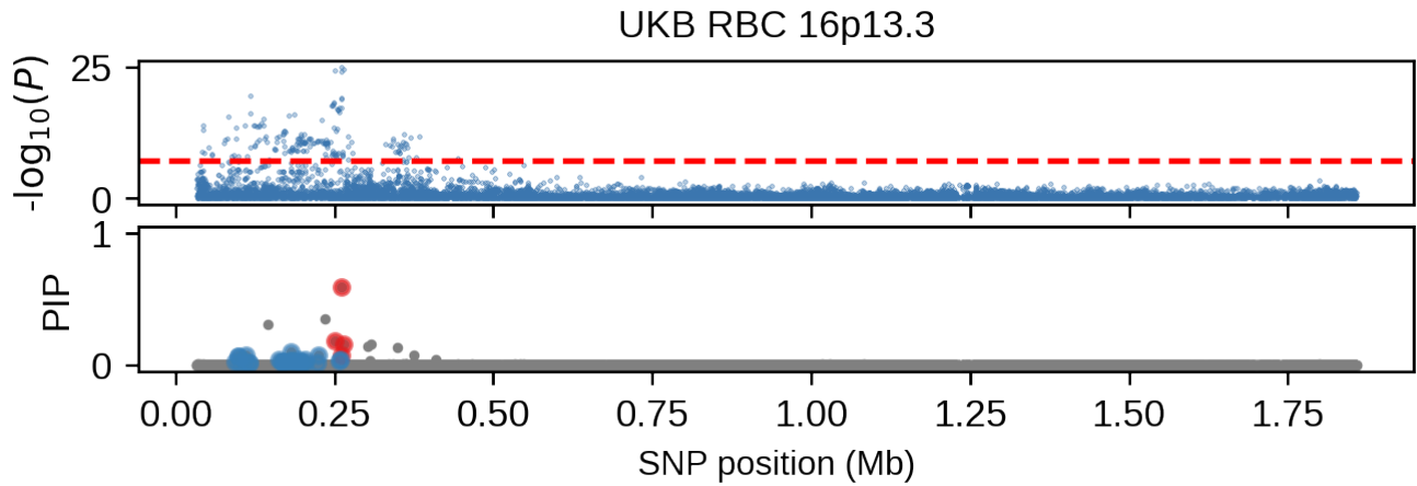
Figure S4: Association p -values and fine-mapping PIP of RBC at 16p13.3 for UK Biobank European-African admixed individuals. Upper panel corresponds to the association p -values and lower panel corresponds to the fine-mapping PIP. Different colors in the PIP plot corresponds to different credible sets.
