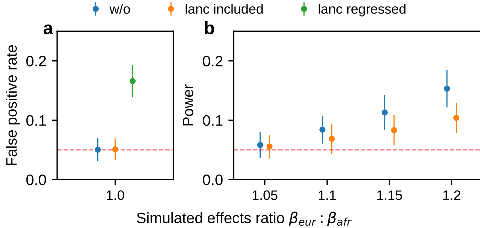
Figure 5: Pitfalls of including local ancestry in estimating heterogeneity. In each simulation, we selected a single causal variant and simulated quantitative phenotypes where these causal variants explain heritability h_g^2 = 0.6\% ; we also varied ratios of effects across ancestries \beta_{\text{eur}} : \beta_{\text{afr}} . (a) False positive rate in null simulation \beta_{\text{eur}} : \beta_{\text{afr}} = 1.0 . (b) Power to detect \beta_{\text{eur}} \neq \beta_{\text{afr}} in power simulations with \beta_{\text{eur}} : \beta_{\text{afr}} > 1 . 95% confidence intervals are calculated based on 100 random sub-samplings with each sample consisting of 500 SNPs (Methods). Numerical results are reported in Table S8.
