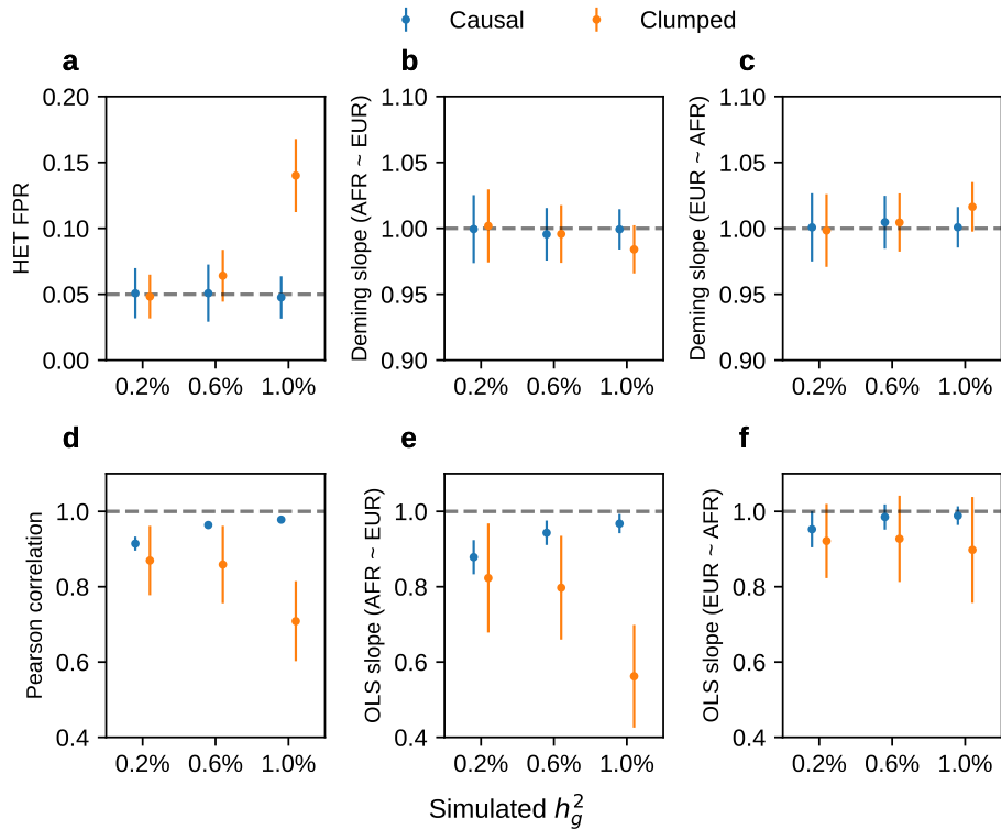
Figure S6: Simulations with single causal variant. Simulation were based on 100 regions each spanning 20 Mb on chromosome 1 and 17,299 PAGE individuals. In each simulation, we randomly selected single causal variant and simulated quantitative phenotypes where these causal variants had same causal effects across ancestries and each causal variant was expected to explain a fixed amount of heritability (0.2%, 0.6%, 1.0%). Each panel corresponds to one metric for both causal and clumped variants. (a) False positive rate (FPR) of HET test. (b) Deming regression slope with \beta_{\text{afr}} \sim \beta_{\text{eur}} . (c) Deming regression slope with \beta_{\text{eur}} \sim \beta_{\text{afr}} . (d) Pearson correlation. (e) OLS regression slope with \beta_{\text{afr}} \sim \beta_{\text{eur}} . (f) OLS regression slope with \beta_{\text{eur}} \sim \beta_{\text{afr}} . 95% confidence intervals were based on 100 random sub-samplings with each sample consisted of 500 SNPs (Methods). Numerical results are reported in Table S9.
