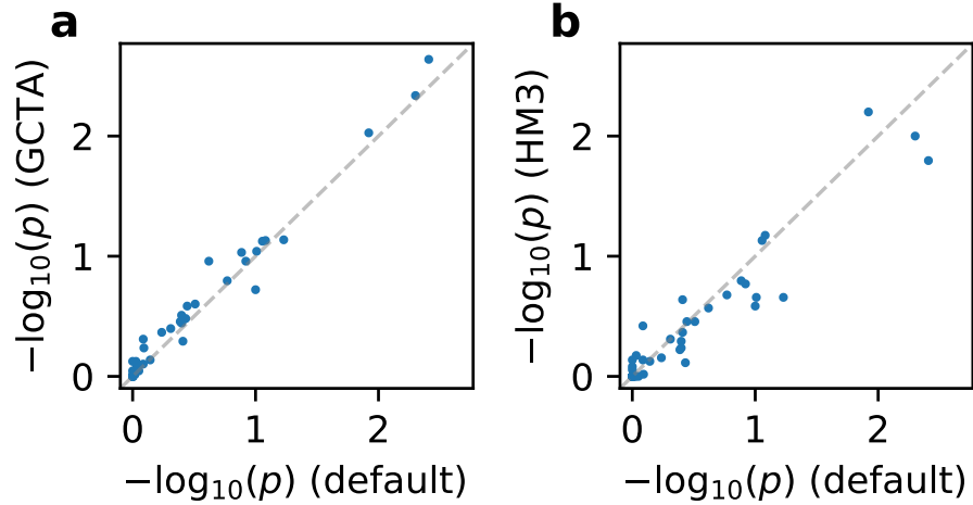
Figure S2: Genetic correlation estimation are robust to genetic architecture and SNP set. We performed r_{\text{admix}} estimation under the assumption of alternative genetic architecture and SNP set on real trait analysis across PAGE and UKBB. We compared p -values (for testing genetic correlation H_0 : r_{\text{admix}} = 1 ) of our default setting (using frequency-dependent genetic architecture and imputed SNPs; Table 1) to those obtained using GCTA genetic architecture and imputed SNPs (a), and to those obtained using frequency-dependent genetic architecture and HM3 SNPs (b). Numerical results are reported in Table S6.
