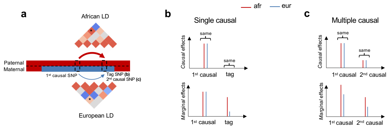
Figure 4: Induced heterogeneities in marginal effects across local ancestries. (a) Illustrations that different LD patterns across local ancestries can induce differential tagging between a causal SNP and a tag SNP in (b) or another causal SNP in (c). LD strengths between the two SNPs are indicated both in the thickness of arrows and in the color shades of ‘*’ elements in LD matrices. (b) Example of single causal SNP with no heterogeneity. Causal effects are the same across local ancestries, and the estimated marginal effects at causal SNP will be also very similar with sufficient sample size. However, because of differential tagging across local ancestries, the estimated marginal effects evaluated at the tag SNP are different. (c) Example of multiple causal SNPs with no heterogeneity. Causal effects for both SNPs are the same across local ancestries. In this example, the correlation between the 2 causal variants is higher for genotypes in African local ancestries than those in European local ancestries. Therefore, African ancestry-specific genotypes tag more effects, creating different marginal ancestry-specific effects at each causal SNP.
