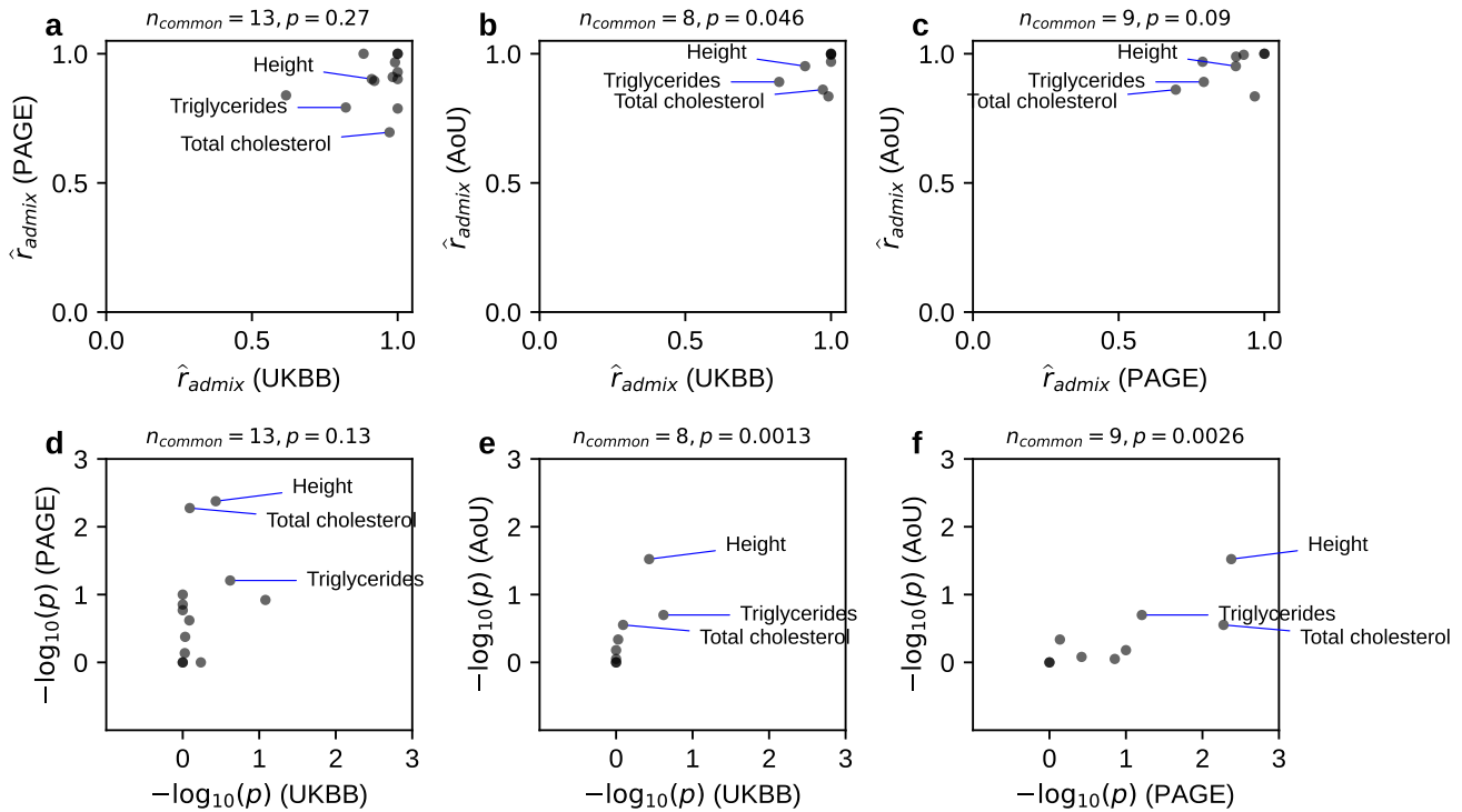
Figure S1: Consistency of r_{\text{admix}} across shared traits across studies. We compared estimated r_{\text{admix}} for shared traits across studies. We compared both \hat{r}_{\text{admix}} and -\log_{10}(p) (for testing genetic correlation H_0 : r_{\text{admix}} = 1 ). Three traits (Height, Triglycerides, Total cholesterol) with the most significant p -values for H_0 : r_{\text{admix}} = 1 were annotated. Number of common traits shared across studies ( n_{\text{common}} ) and Spearman correlation p -value were shown in the title for each panel. Overall, there were weak consistency of estimated \hat{r}_{\text{admix}} for shared traits across studies (although p -values for H_0 : r_{\text{admix}} = 1 were consistent significantly). Numerical results are reported in Table S5.
