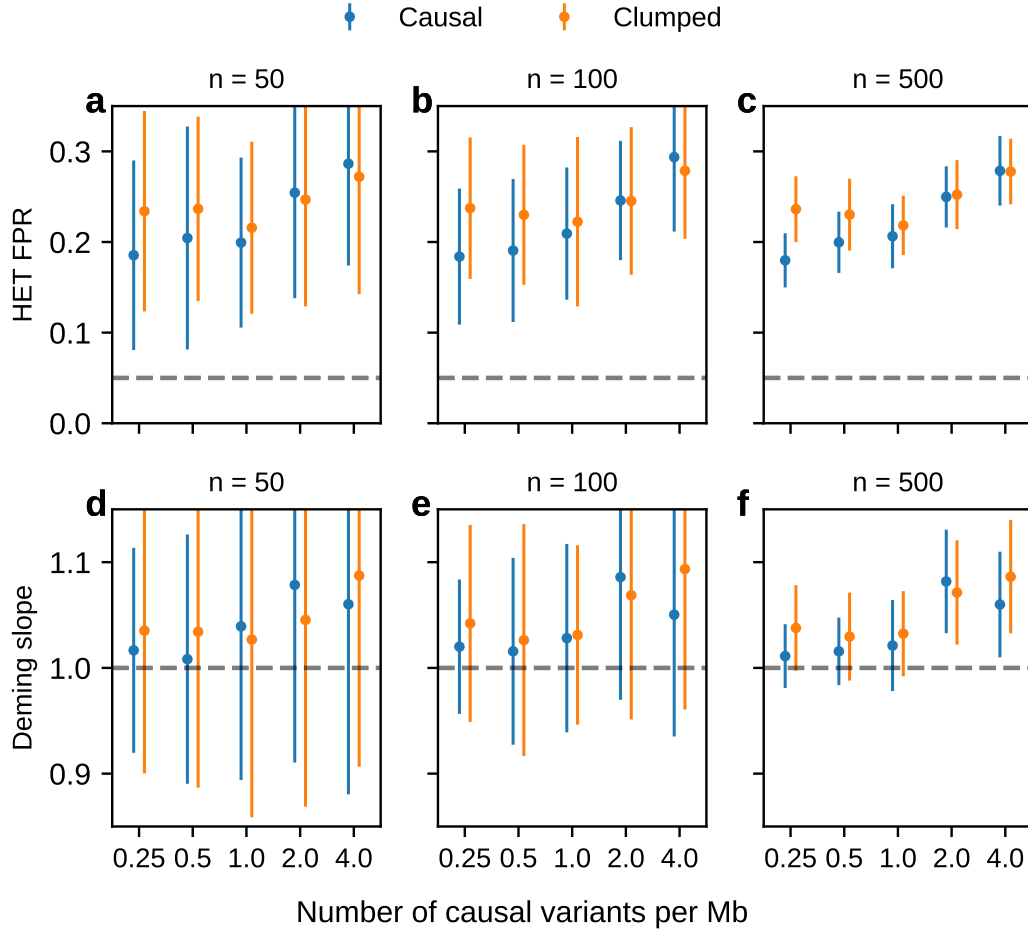
Figure S7: Simulation with multiple causal variants at other sample sizes (Figure 6cd) . Simulation were based on chromosome 1 (515,087 SNPs) and 17,299 PAGE individuals. We drew 62, 125, 250, 500, 1000 causal variants to simulate different level of polygenicity, such that on average there were approximately 0.25, 0.5, 1.0, 2.0, 4.0 causal variants per Mb. The heritability explained by all causal variants was fixed at h_g^2 = 10\% . (a-c) False positive rate of HET test for the causal variants and clumped variants. (d-f) Deming regression slope of estimated ancestry-specific effects ( \beta_{\text{eur}}^{(m)} \sim \beta_{\text{afr}}^{(m)} ) for the causal variants and clumped variants. 95% confidence intervals were based on 100 random sub-samplings with each sub-sample consisted of n = 50, 100, 500 SNPs (instead of n = 1,000 SNPs in Figure 6cd) (Methods).
