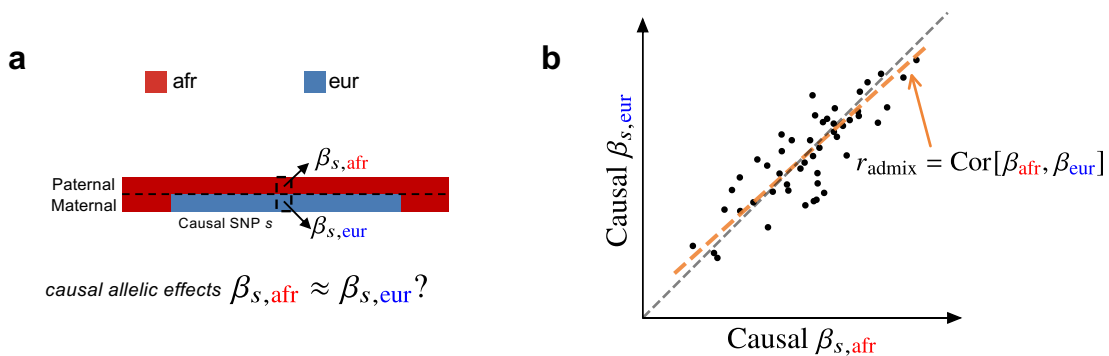
Figure 1: Concepts of estimating similarity in the causal effects across local ancestries. (a) For a given trait, with phased genotype (paternal haplotype at the top and maternal haplotype at the bottom) and inferred local ancestry (denoted by color), we investigate whether \beta_{s,\text{afr}} \approx \beta_{s,\text{eur}} across each causal SNP s . (b) We focus on estimating the genome-wide correlation of genetic effects across ancestries r_{\text{admix}} = \text{Cor}[\beta_{\text{afr}}, \beta_{\text{eur}}] , which is the regression slope (orange line) of ancestry-specific causal effects. For reference, the grey dashed line corresponds \beta_{\text{afr}} = \beta_{\text{eur}} .
