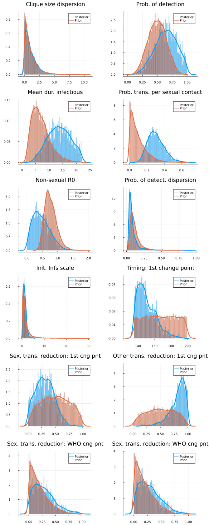
Figure S2. Empirical distributions of the target parameters for inference (blue and orange colours, posterior and prior distributions, respectively).
