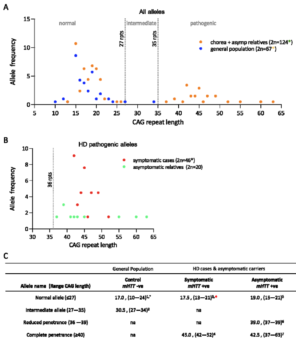
Figure 2: Allele Frequency distribution
