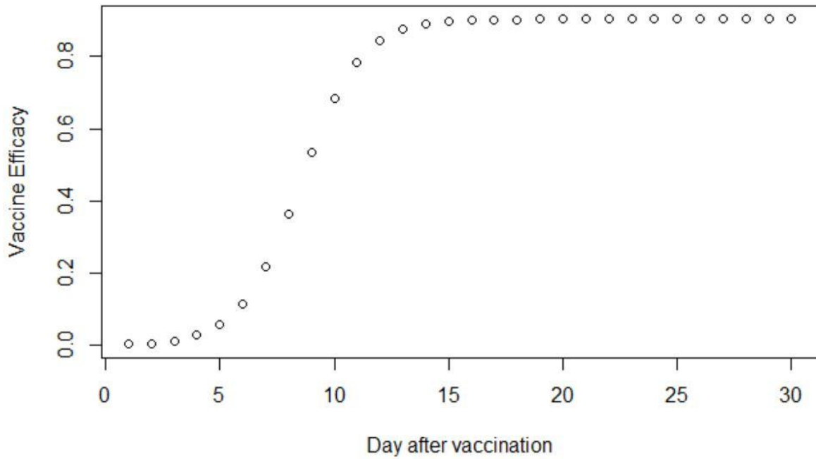
Figure A1: Curve showing vaccine efficacy as a logistic function of days after vaccination
