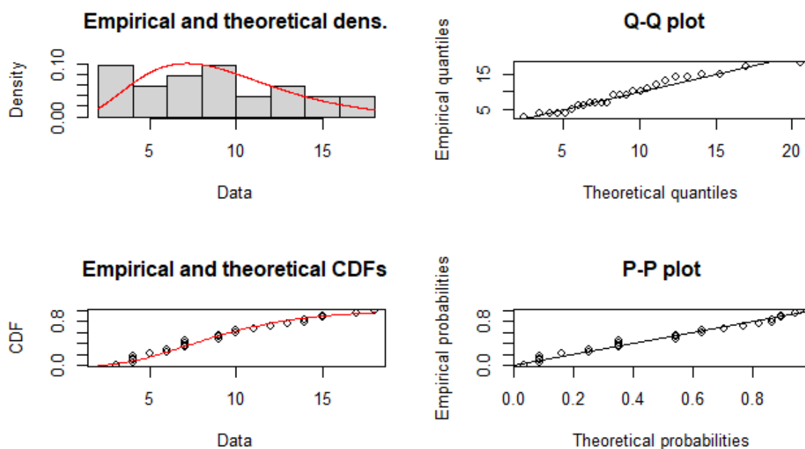
Figure A2: Plot of fitted and observed values of the serial interval for marburgvirus disease.
