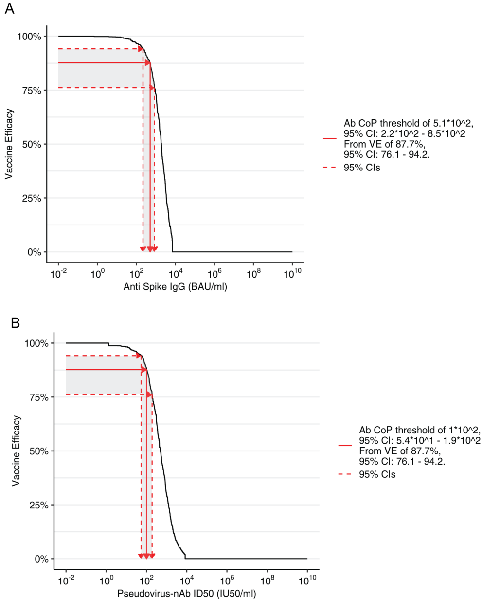
Supplementary Figure 3. Inverse probability sampling (IPS)-weighted empirical reverse cumulative distribution function curves for each Day 35 marker (spike IgG, nAb ID50) and application of the Siber (2007) method 2 for estimating a threshold of perfect vs. no protection.
