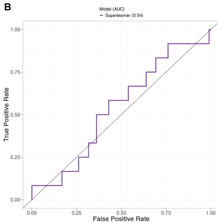
Supplementary Figure 5. Performance of the baseline risk score built from ensemble machine learning. (A) Receiver operating characteristic (ROC) curves based on cross-validated (CV)-estimated predicted probabilities for the top two learners, Superlearner and Discrete Superlearner. CV-estimated predicted probabilities were computed using only data from the placebo arm in the US. (B) ROC curve based on Superlearner predicted probabilities in vaccine recipients.
