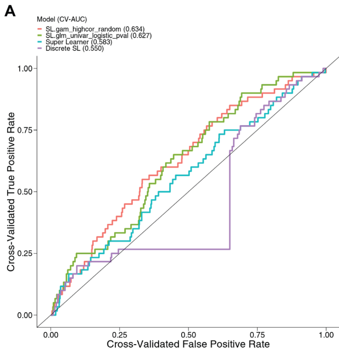
Supplementary Figure 5. Performance of the baseline risk score built from ensemble machine learning. (A) Receiver operating characteristic (ROC) curves based on cross-validated (CV)-estimated predicted probabilities for the top two learners, Superlearner and Discrete Superlearner. CV-estimated predicted probabilities were computed using only data from the placebo arm in the US. (B) ROC curve based on Superlearner predicted probabilities in vaccine recipients.
