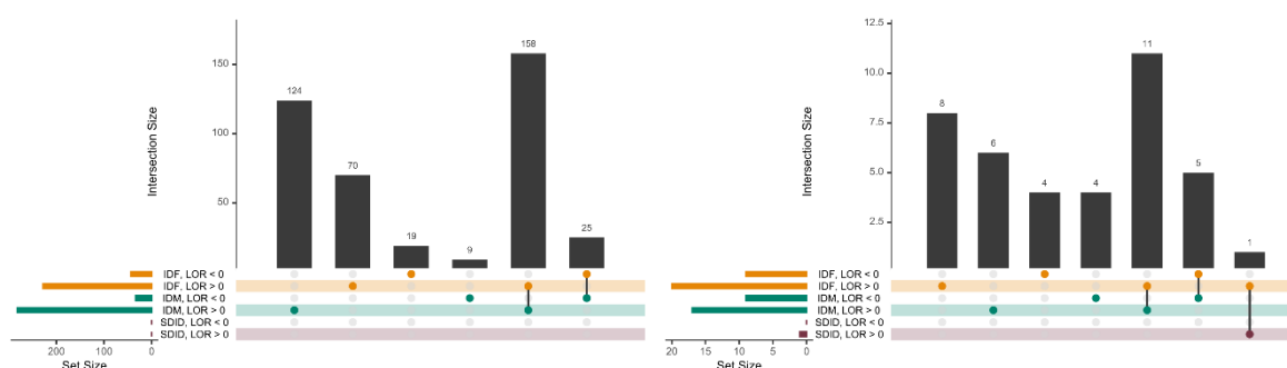
Figure 7. Upset plot of the functional enrichment results in nervous tissue for BP GO terms. Horizontal bars indicate the number of significant BP GO terms in each comparison (a specific color for each comparison). Results are exhibited separately for significantly upregulated (LOR > 0) and downregulated (LOR < 0) BP GO terms. The vertical bars indicate the genes included in the intersection of the groups denoted with a colored dot
