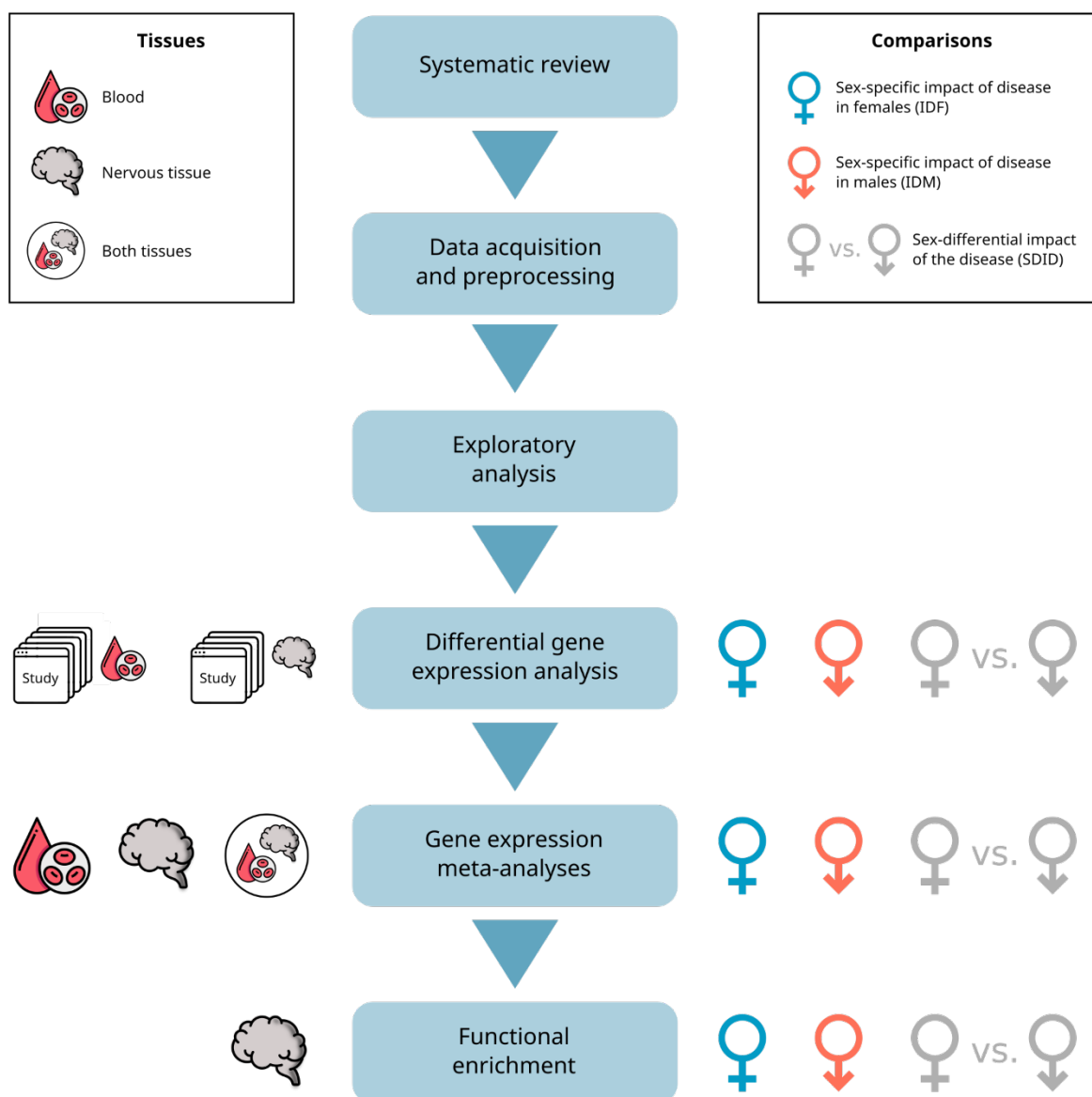
Figure 1. Flowchart describing the work performed, indicating tissues analyzed and comparisons performed in each step.
