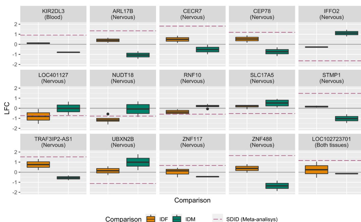
Figure 3. Boxplot of LFC values for the DGE in the SDID comparison. Each boxplot indicates the log fold-change (LFC) values of a gene in the individual DGEs. The dashed purple line indicates the LFC value of the meta-analysis for the SDID comparison. The gray line (at a value of 0) indicates the absence of change. The tissue in which the gene is significant is indicated in parentheses under the gene name.
