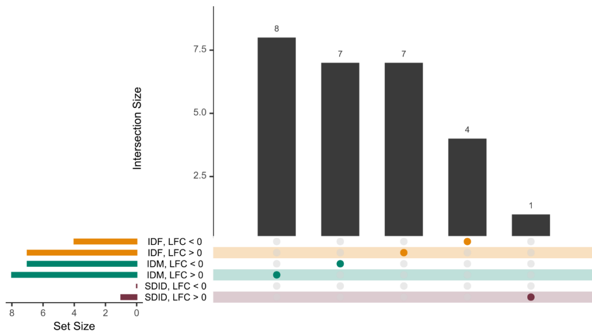
Figure 6. Upset plot of the two-tissue meta-analysis results. The results of each comparison are separated according to the LFC sign. Horizontal bars indicate the number of significant elements in each comparison (one specific color for each comparison). The vertical bars indicate the genes included in the intersection of the groups denoted with a colored dot underneath. A colored dot under a bar indicates that the genes are specific to this group.
