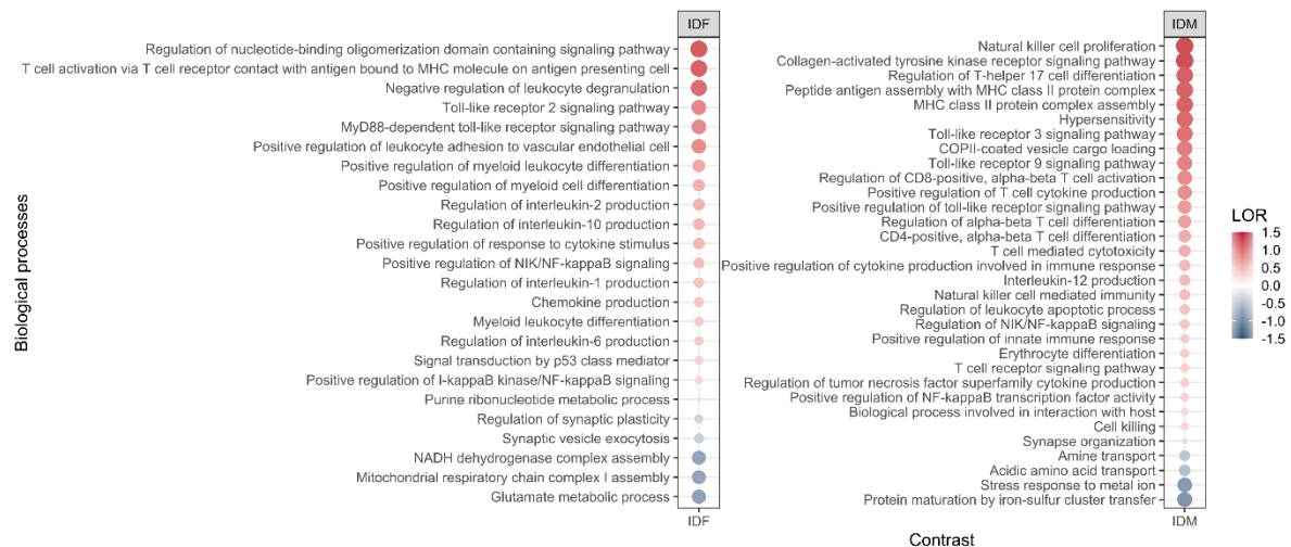
Figure 9. Dotplot of a representative selection of the specific significant BP GO terms in IDF and IDM. GO terms affected exclusively in IDF (left) or IDM (right). The color and size of the dots represent the sign and magnitude of the change (LOR).
