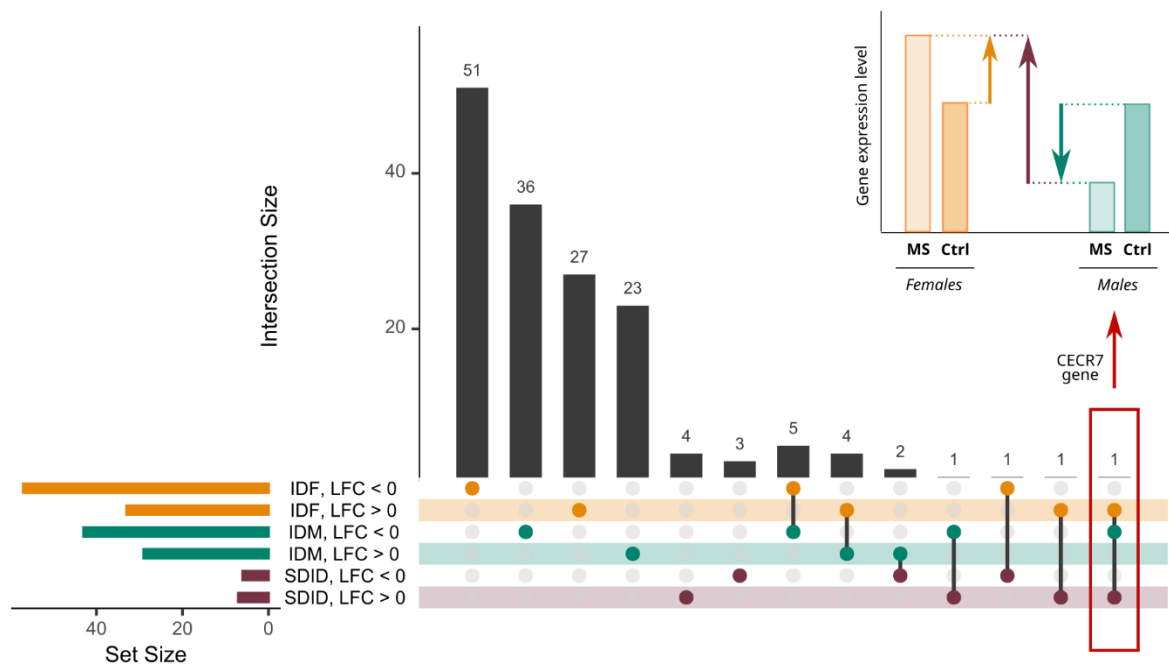
Figure 5. Upset plot of the meta-analysis results in nervous tissue samples. The results of each comparison are separated according to the LFC sign. Horizontal bars indicate the number of significant genes in each comparison (a specific color for each comparison). The vertical bars indicate the genes included in the intersection of the groups denoted with a colored dot underneath. A colored dot under a bar indicates that the genes are specific to this group. The red box indicates the case of the CECR7 gene, which is significant in all comparisons in the manner represented by the bar plot in the upper right corner.
