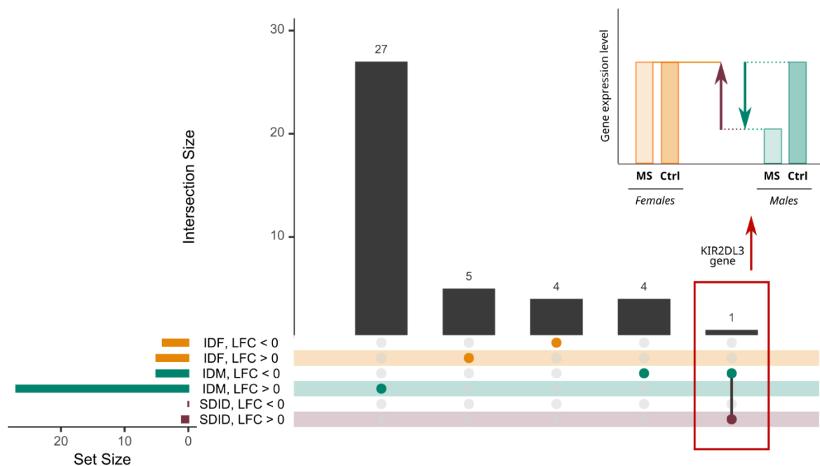
Figure 4. Upset plot of meta-analysis results in blood studies. The results of each comparison are separated according to the LFC sign. Horizontal bars indicate the number of significant genes in each comparison (1 specific color for each comparison). The vertical bars indicate the genes included in the intersection of the groups denoted with a colored dot underneath. A colored dot under a bar indicates that the genes are specific to this group. The red box indicates the case of the KIR2DL3 gene, which is significant SDID and IDM comparisons in the manner represented by the bar plot in the upper right corner.
