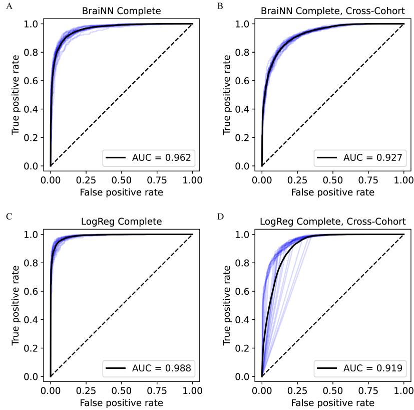
Supplementary Figure 2: Receiver operation characteristic (ROC) curves for BraiNN (CNN) and LogReg on the complete SHIP data set. The ROC curves of each single training run are shown in blue, the black curves are the respective averaged ROC curves. The mean area under the curve (AUC) is shown in the bottom right of the plots. A) ROC and AUC for BraiNN, trained on the complete SHIP data set when predicting the SHIP test data. B) ROC and AUC for BraiNN, trained on the complete SHIP data set when predicting the HCP data set. C) ROC and AUC for LogReg, trained on the complete SHIP data set when predicting the SHIP test data. D) ROC and AUC for LogReg, trained on the complete SHIP data set when predicting the HCP data set. The LogReg in this setting has a tendency to predict values close to 1, even for male images (data not shown), thus the shape of the blue curves here.
