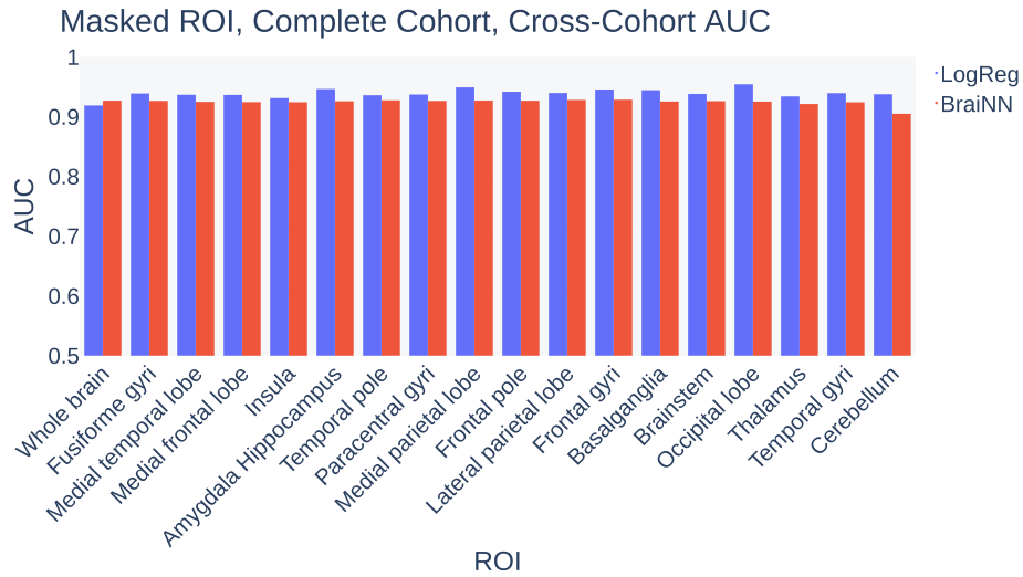
Supplementary Figure 6: AUC of LogReg and BraiNN (CNN) for “whole brain” images and images missing certain brain regions. Top: Performance on the test data (see Section 2.3). Bottom: Performance on the HCP data set. In all cases, the complete SHIP data set was used for training. See Table 3 for the exact values.
