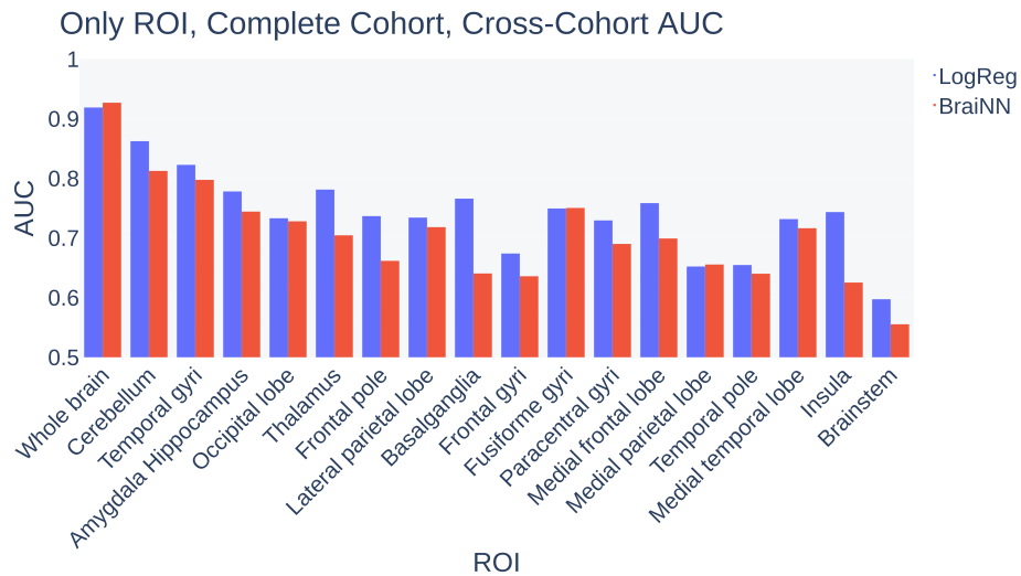
Supplementary Figure 5: AUC of LogReg and BraiNN (CNN) for “whole brain” images and images containing only certain brain regions. Top: Performance on the test data (see Section 2.3). Bottom: Performance on the HCP data set. In all cases, the complete SHIP data set was used for training. See Table 1 for the exact values.
