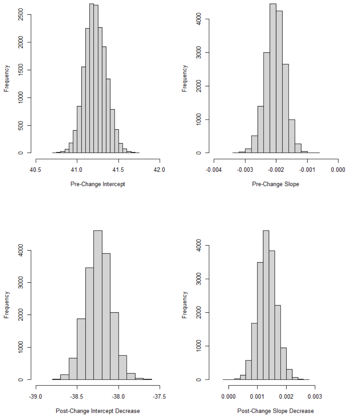
Figure 2. Tertiary hospital posterior estimates; x-axes represent hours related to receiving methicillin-resistant Staphylococcus aureus (MRSA) results with the pre-change period being before the testing switch from culture to polymerase chain reaction in the adult Intensive Care Unit.
