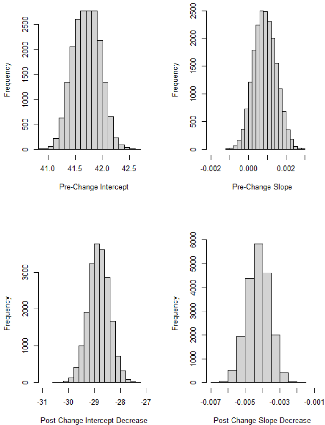
Figure 3. Community hospital posterior estimates; x-axes represent hours related to receiving methicillin-resistant Staphylococcus aureus (MRSA) results with the pre-change period being before the testing switch from culture to polymerase chain reaction in the adult Intensive Care Unit.
