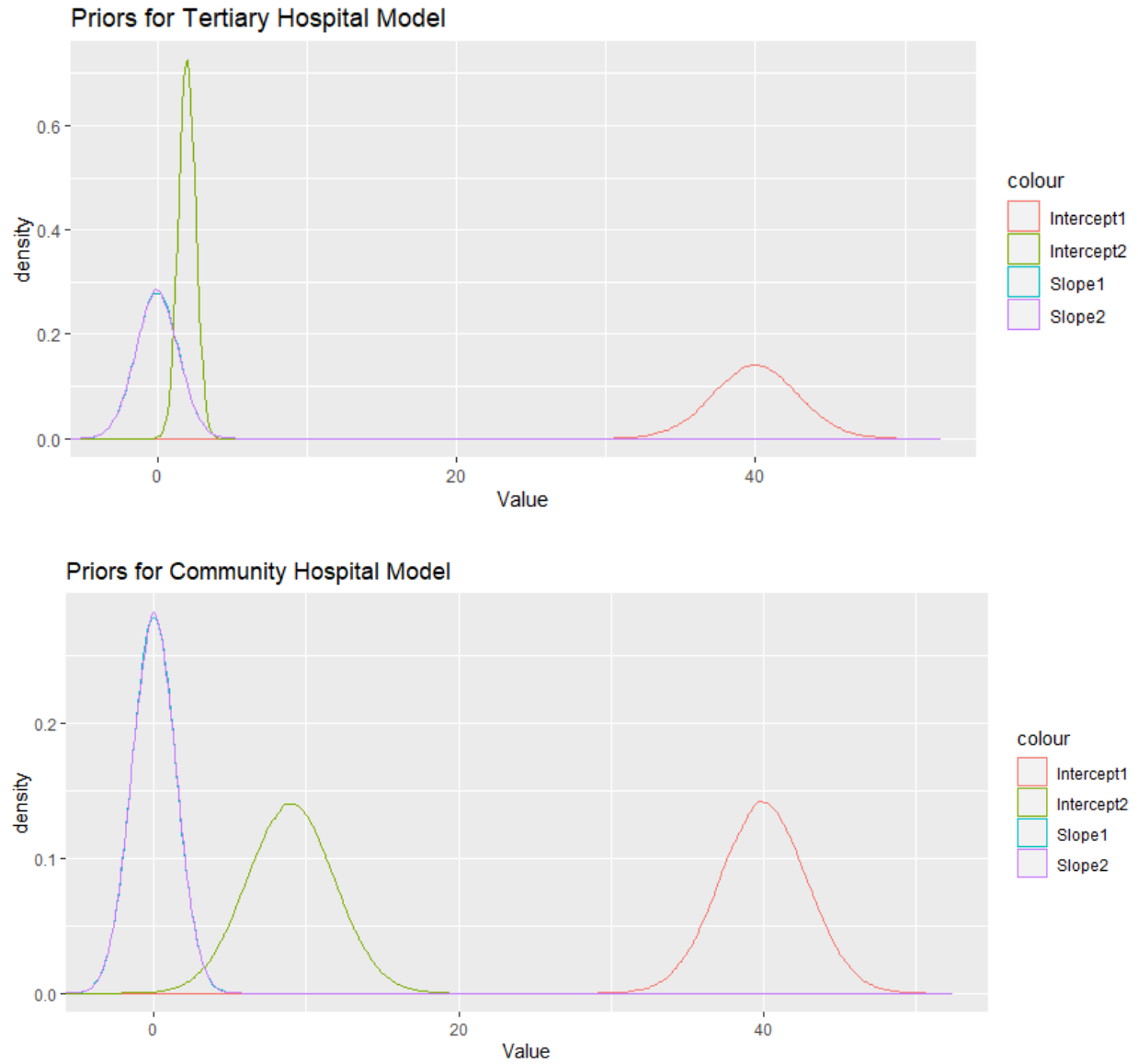
Figure 1. Top panel presents the priors used in the tertiary hospital model and the bottom panel presents the priors used in the community hospital model. Priors for slope values for the two-line segments were the same and mostly overlap in the above figures.
