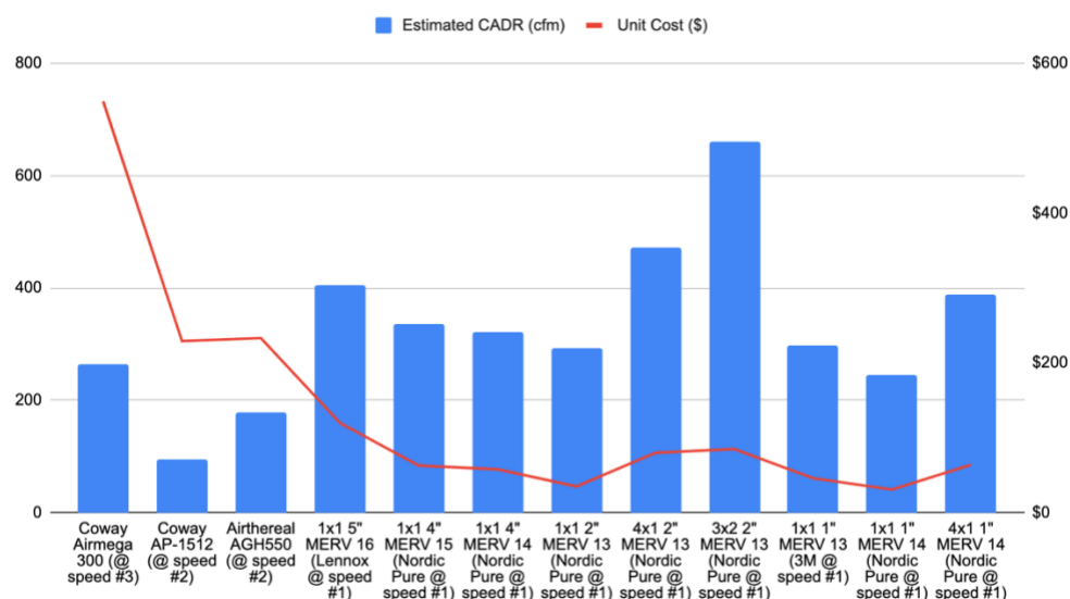
78 79 80 81 Figure 1: comparison of est. CADR and cost of HEPA purifiers and DIY box fan-filters 82 e.g., 3x2 means three filters were used with two box fans 83
