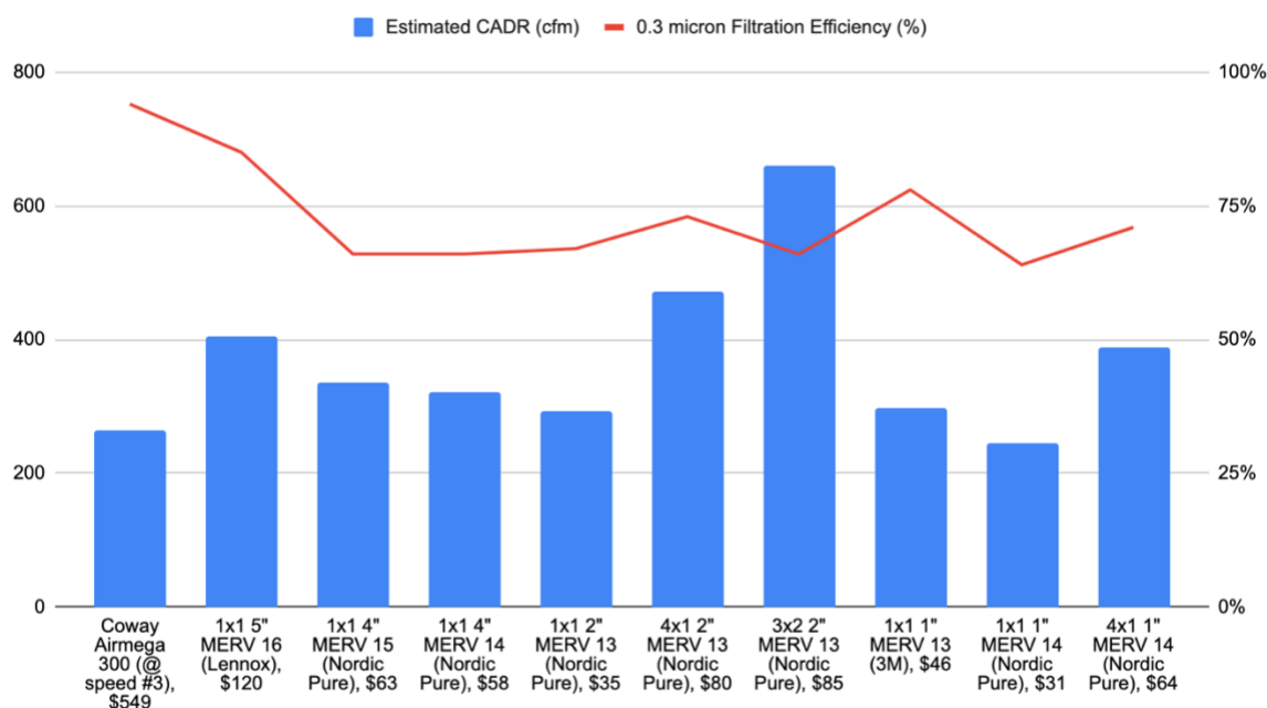
235 Figure 3: Estimated CADR (cfm) for DIY Air Purifiers (filters x fans) @ speed #1 e.g., 3x2 236 means three filters were used with 2 box fans
