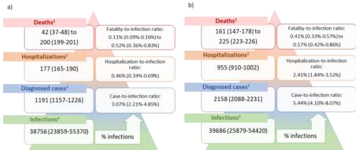
Appendix Figure 2. South African age-standardized SARS-CoV-2 infection, diagnosis, hospitalization and deaths per 100,000 population during wave 3 in the a) rural and b) urban community, March – November, 2021, South Africa
