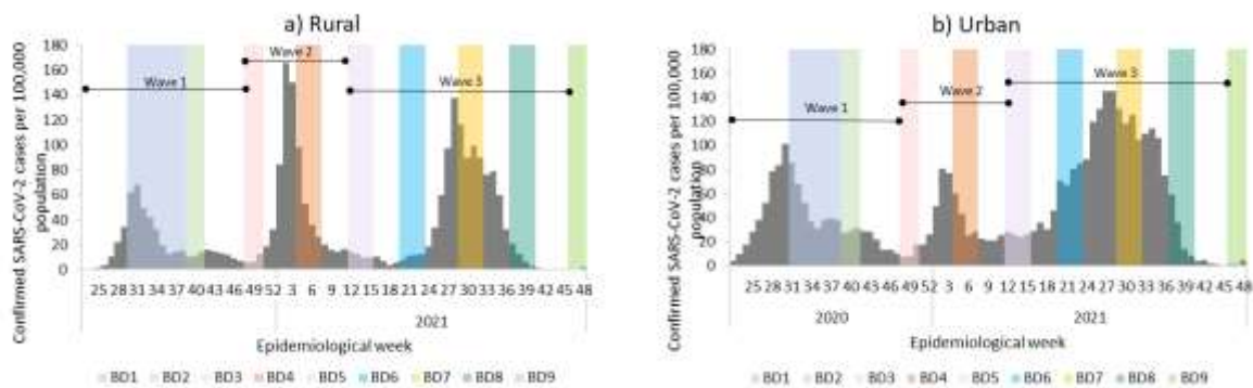
Appendix Figure 1. Timing of blood collection and district SARS-CoV-2 weekly incidence 1 in a) rural community and b) urban community, March 2020 – November 2021, South Africa.
