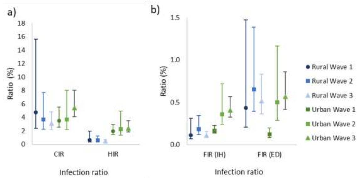
Appendix Figure 3. SARS-CoV-2 a) case-to-infection (CIR), hospitalization-to-infection (HIR) and b) in-hospital (IH) fatality-to-infection (FIR) and excess (ED) fatality-to-infection (FIR) ratios in a rural and urban community during the first, second and third wave of infections, March 2020 - November 2021, South Africa.
