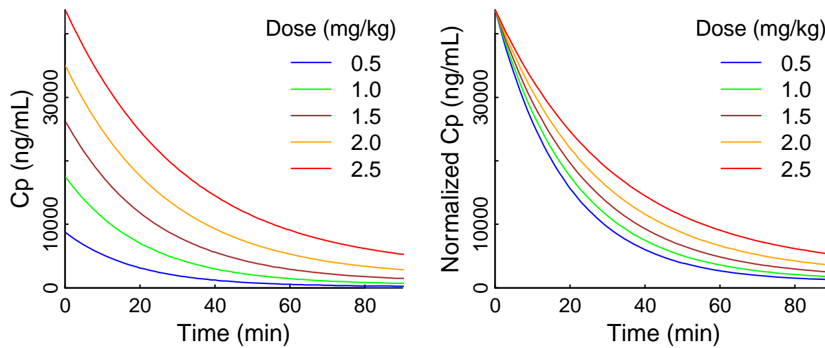
Figure 2: Simulated TSC concentration profiles
