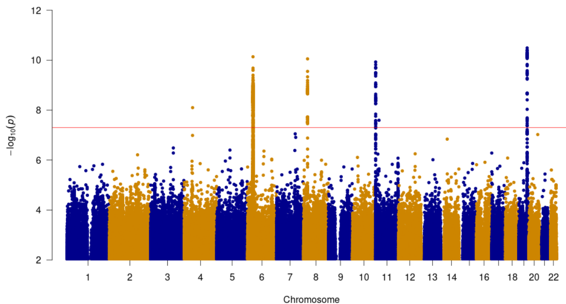
Figure 2 Manhattan plot for genome-wide association study of sputum production. The red line indicates genome-wide significance.
