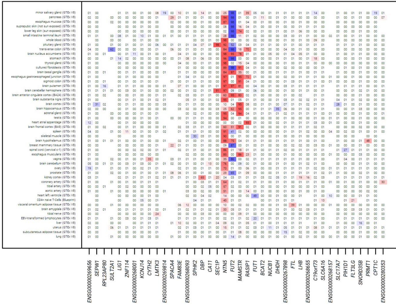
Figure 4 Results for eQTL colocalization for the FUT2 locus using variant rs492602 . The numbers within the grid are the posterior probability of colocalization (H4), with results aligned to the risk allele G for the rs492602 variant. Missing numbers indicate no data was available for the respective gene and tissue.
