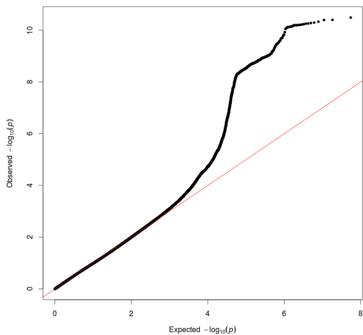
Figure 1 Quantile-quantile (QQ) plot for results of genome-wide association study of sputum production. Variants with imputation quality INFO <0.5 and minor allele count (MAC) <20 were excluded. The genomic control inflation factor, lambda, was 1.026.
