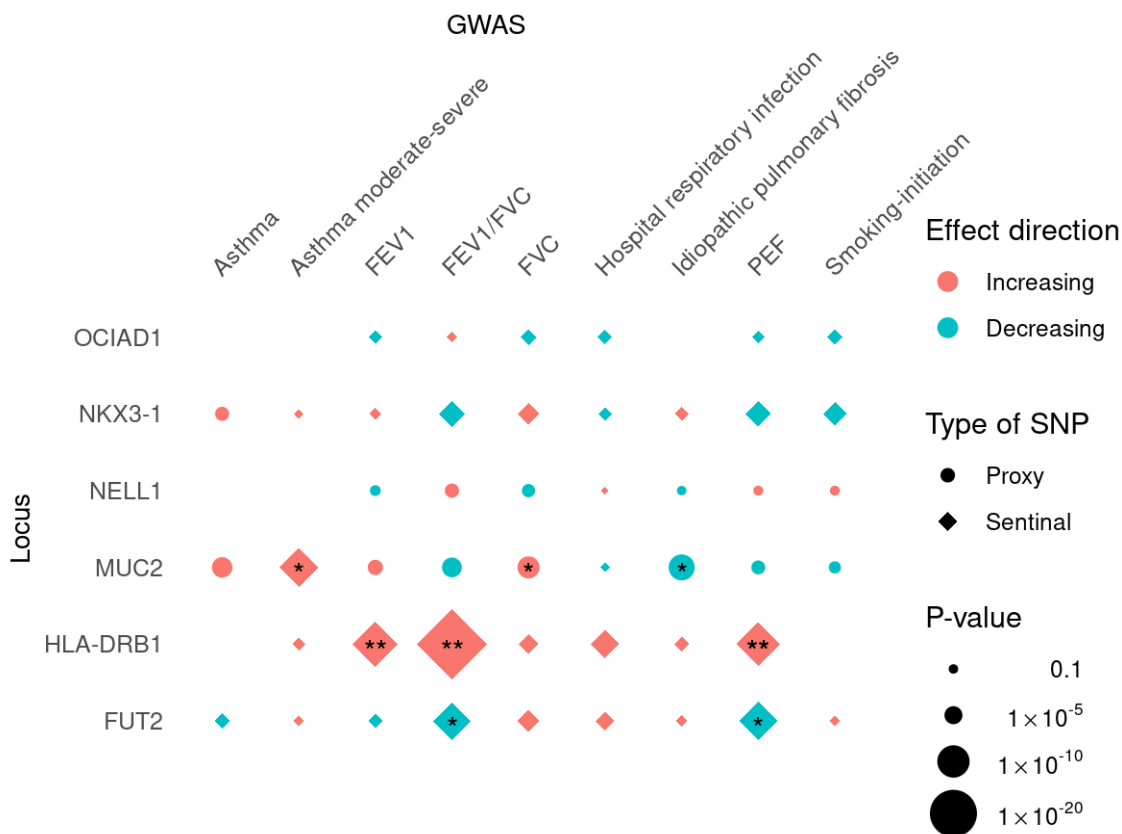
Figure 3 Results for association of sentinel variant risk alleles with respiratory traits. Results are aligned to the risk allele for chronic sputum production, effect direction ‘Increasing’ can be read as increasing risk for binary traits and increasing values in quantitative traits. Smoking age of onset, cigarettes per day and cessation phenotype lookups were omitted as no associations with P < 0.05 found. * P < 6.94 \times 10^{-4} (Bonferroni adjustment for 72 association tests) ** P < 5 \times 10^{-8} .
