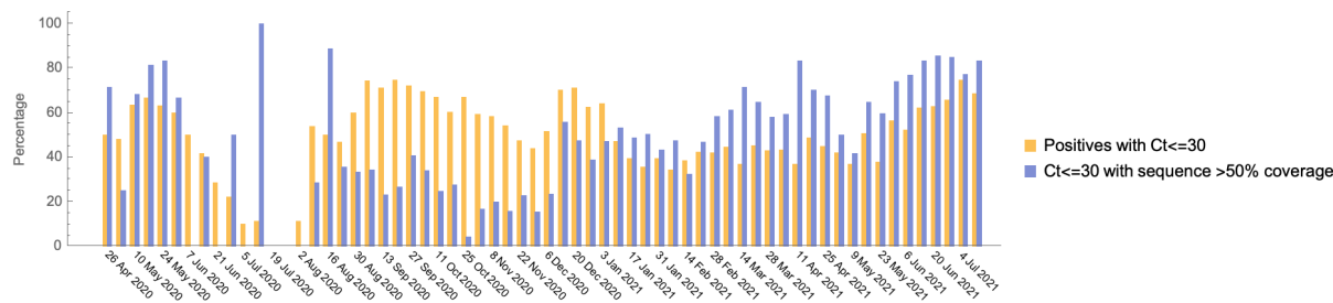
Figure S6: Sample proportions by collection week. The figure shows the percentage of ONS CIS RT PCR positive samples with Ct ≤ 30 (yellow), and the percentage of Ct ≤ 30 samples that have sequence with > 50% genome coverage.
