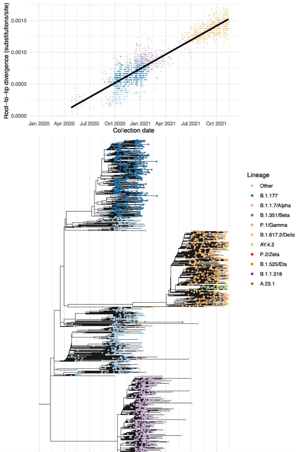
Figure 4. Dated phylogeny and root-to-tip distance of ONS CIS sequences. First, a maximum likelihood phylogeny of ONS sequences with over 95% genome coverage up to and including 13th November 2021 (Fig S3) was generated using RAxML-NG. A. Root to tip distance for samples from the maximum likelihood phylogeny. B. Time tree generated from the maximum likelihood phylogeny using TreeTime [35]. B.1.177, B.1.1.7/Alpha, B.1.617.2/Delta (including AY.4.2) and 'Other' were each randomly subsampled to a maximum of 500 sequences.
