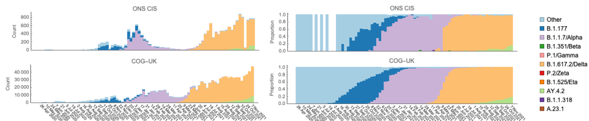
Figure S1. Comparison of lineage dynamics within the ONS CIS and among all COG-UK sequences. Top row: Number of sequenced samples and relative prevalence among ONS CIS sequences. Bottom row: Number of sequenced samples and relative incidence among COG-UK pillar 2 sequences [51], but excluding ONS sequences. All samples are grouped by the week in which they were collected, with the date giving the first day of the collection week (every other week labelled for clarity).
