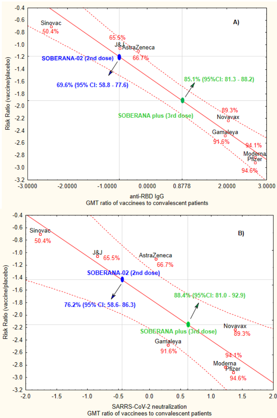
Figure 3. Prediction of clinical efficacy from correlation between antibody responses and efficacy rate
