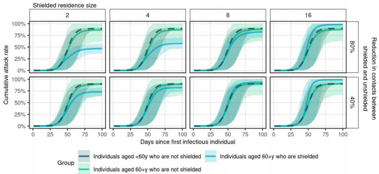
Figure 2. Cumulative infection risk by shielded status over time, since SARS-CoV-2 introduction in the IDP camp. Estimates are stratified by shielded residence size (in facet columns) and reduction in contacts between shielded and unshielded individuals (in facet rows). In each scenario, lines represent the median attack rate across 1000 model runs at each timepoint, whereas corresponding 95% uncertainty intervals are shown by shaded areas of the same colour. Estimates for (unshielded) low-risk individuals are shown in dark-green and a dashed line. Unshielded high-risk individuals are shown in light-green, while shielded high-risk individuals are shown in blue. In all scenarios shown, R_0 was 2.5, 0% of the population were immune at the start of the simulation, and 80% of the high-risk population was shielded.
