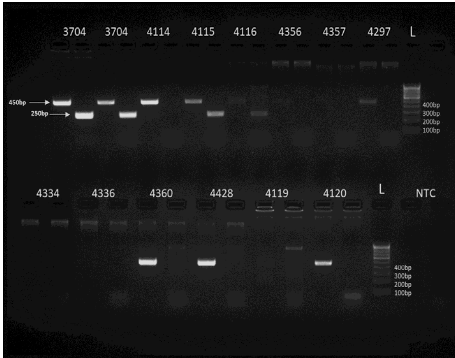
Figure 1: Simplex PCR based assay for the detection of Omicron (B.1.519.2): Primer set 1 resulted in to 250bp bands specific to Omicron. Primer set 2 resulted in to 450bp bands specific all SARS-CoV-2 variants. Numbering on well represents sample numbers for example. L is annotated for ladder (100bp). NTC is non-templet control. Bands other than 450bp and/or 250bp band may be ignored as, it may be nonspecific amplification.
