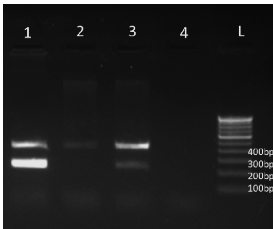
Figure 2: Duplex PCR assay results distinguishing Omicron from other SARS-CoV-2 variants on an agarose gel electrophoresis. Lane 1 & 3: presence of 250 bp band conform the presence
