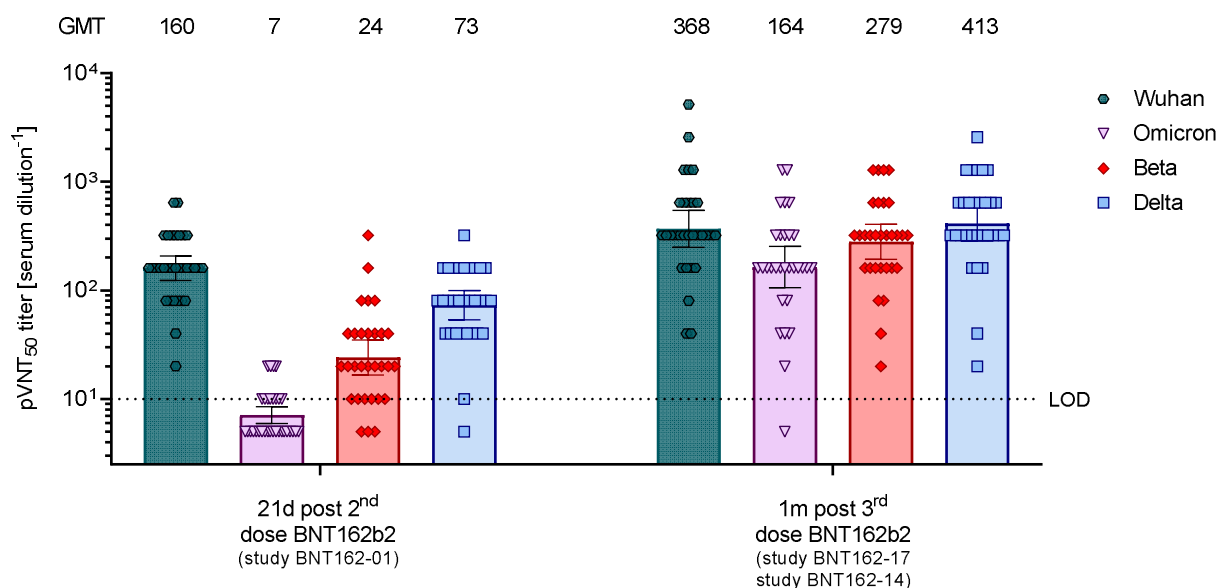
Fig. 1. 50% pseudovirus neutralization titers (pVNT 50 ) of sera from vaccine recipients collected after two or three doses of BNT162b2 against VSV-SARS-CoV-2-S pseudovirus bearing the Wuhan, Omicron, Beta or Delta variant spike protein. N=32 sera from participants in study BNT162-01 drawn at 21 days after dose 2, and n=30 sera from participants in the BNT162-14 (n=11) and BNT162-17 trials (n=19) drawn at 1 month after dose 3 were tested. Each serum was tested in duplicate and geometric mean 50% pseudovirus neutralizing titers (GMTs) were plotted. For values below the limit of detection (LOD), LOD/2 values were plotted. Group GMTs (values) and 95% confidence intervals are indicated.
