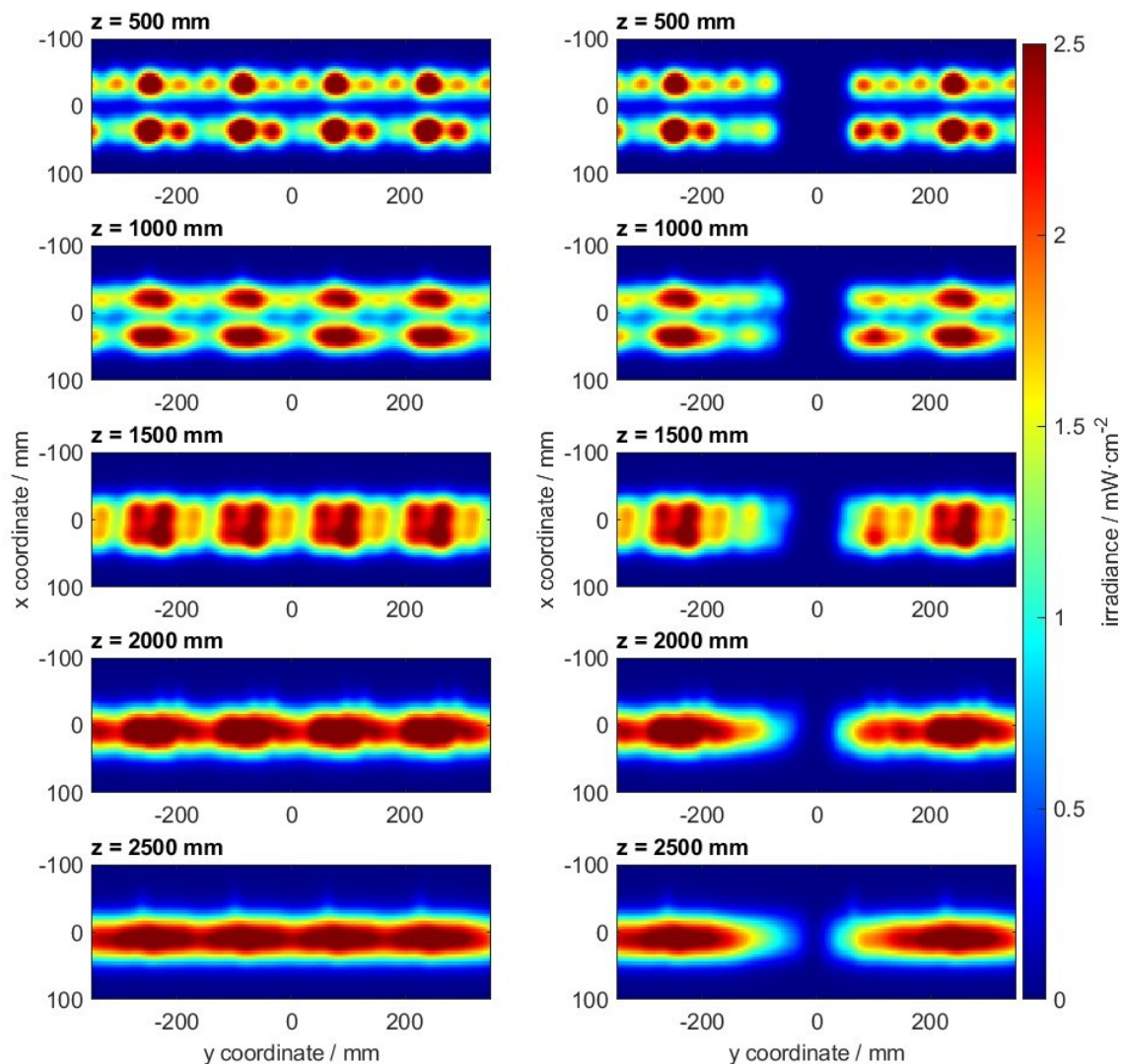
Figure 3: Continuous UV-C curtain simulated mathematically using the measured data of one module (left); the same system with one module in the centre is switched off, simulating a locally engaged safety switch (right).
