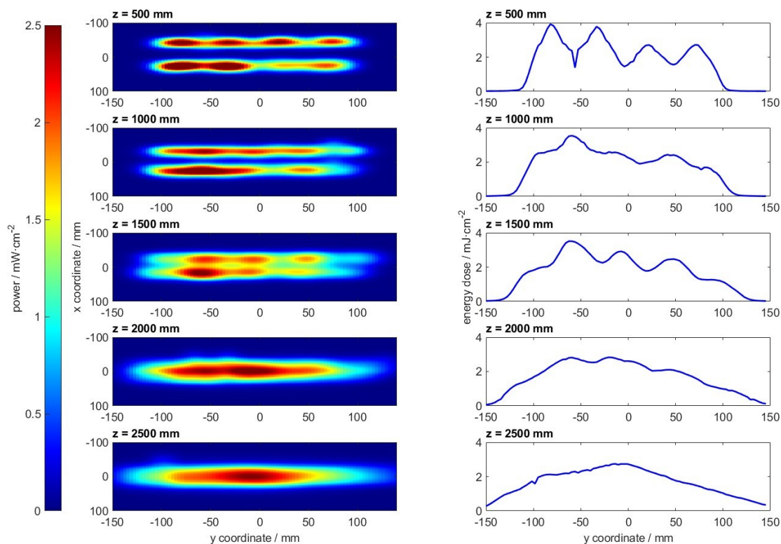
Figure 2: Irradiance map of one optical module in different distances to the source (left) and the corresponding integrated energy dose (right) for a particle passing the light curtain with a speed of 0.1 \text{ m s}^{-1} .
