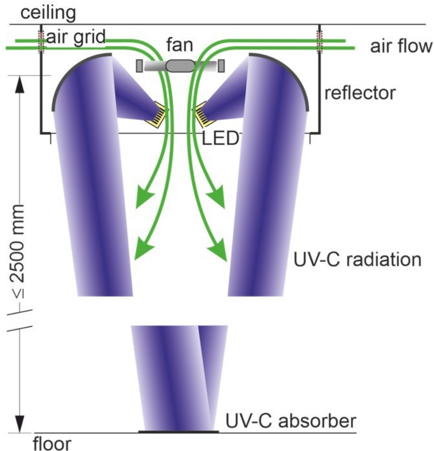
Figure 1: Schematic drawing of the overall system layout. A ceiling mounted housing encloses the mirror based optics and the air duct system.
