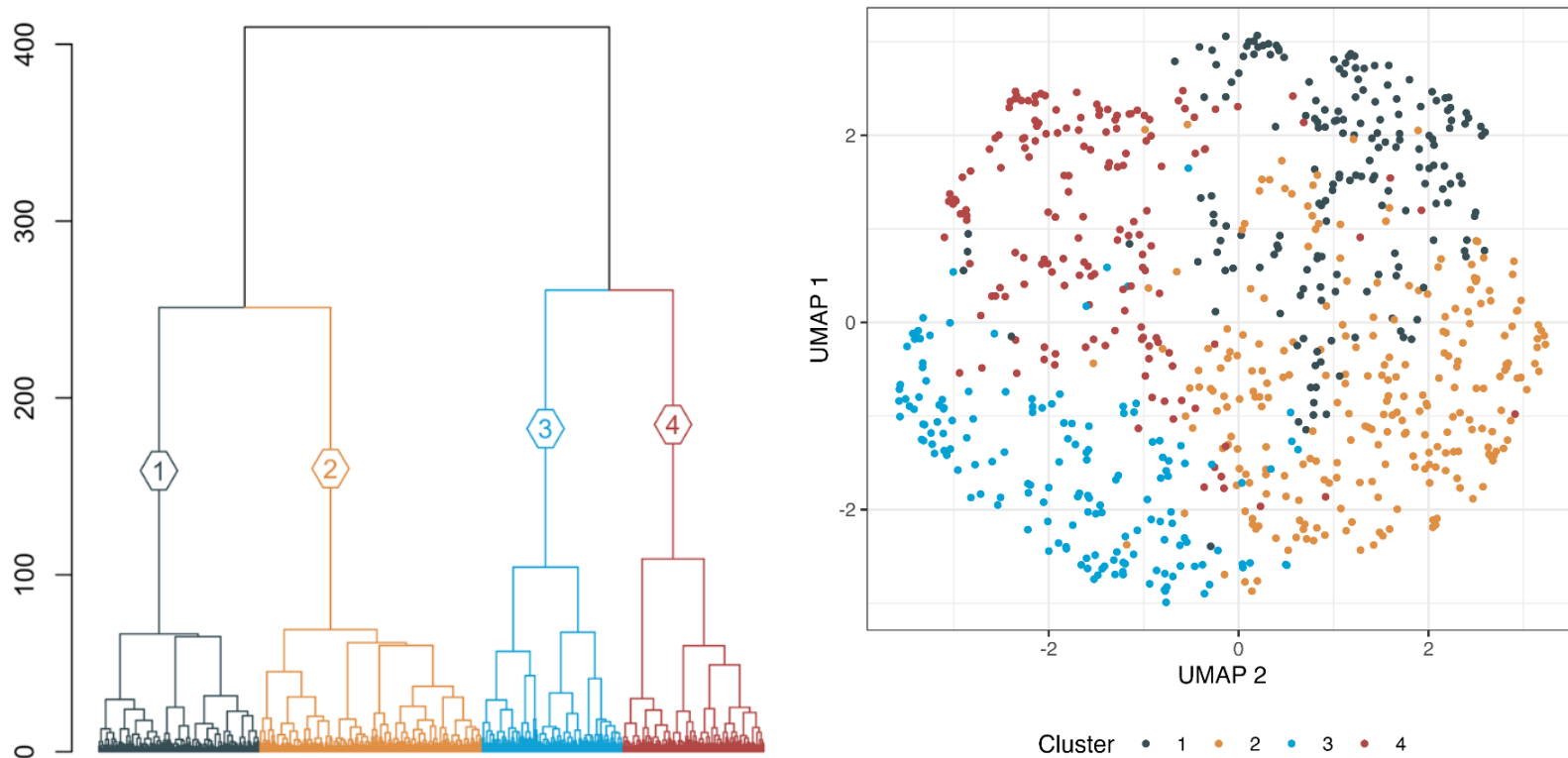
Figure 1. Hierarchical clustering, dendrogram (left). UMAP showing density-based clustering and dimensionality reduction (right).
