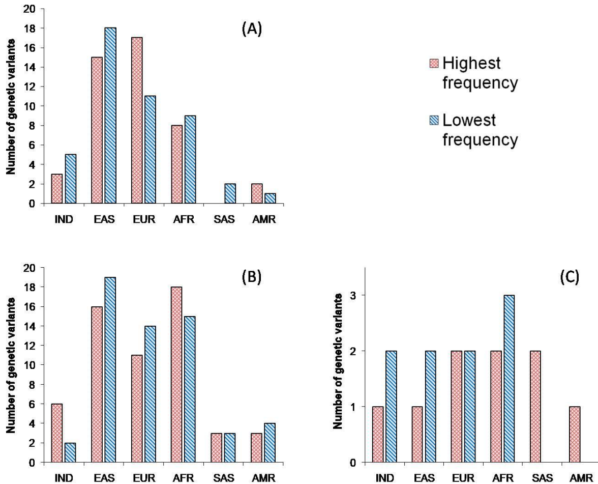
151 Figure 1 Comparison of populations based on the number of variants with highest / lowest risk 152 allele frequency related to (A) Susceptibility to COVID-19, (B) COVID-19 severity, and (C) 153 COVID-19 related mortality or fatal outcomes. IND – India, EUR – Europe, AMR
