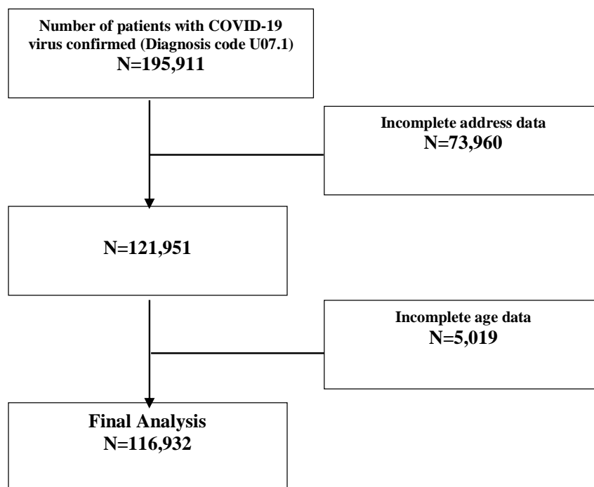
Figure 1. Subjects selection chart
