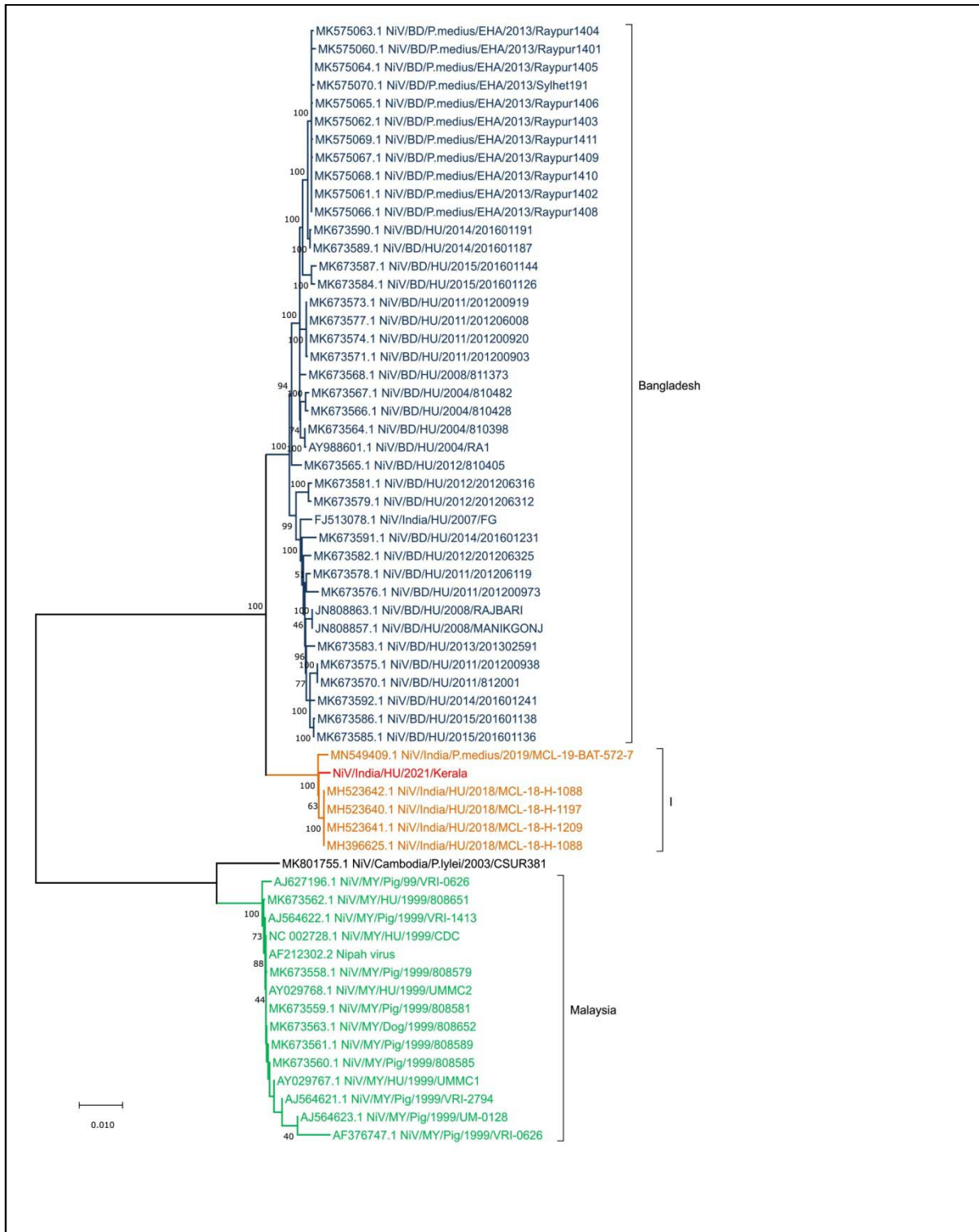
411 Figure 2: Neighbor Joining tree of Nipah virus full genome obtained from the samples of index case 412 in Kerala outbreak 2021
