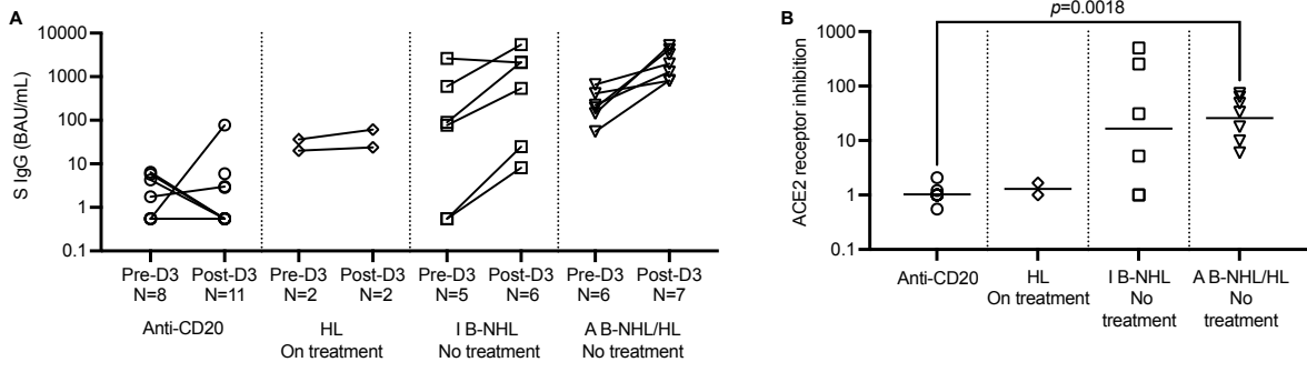
Figure 6. Antibody and pseudoneutralization responses to third vaccine dose
