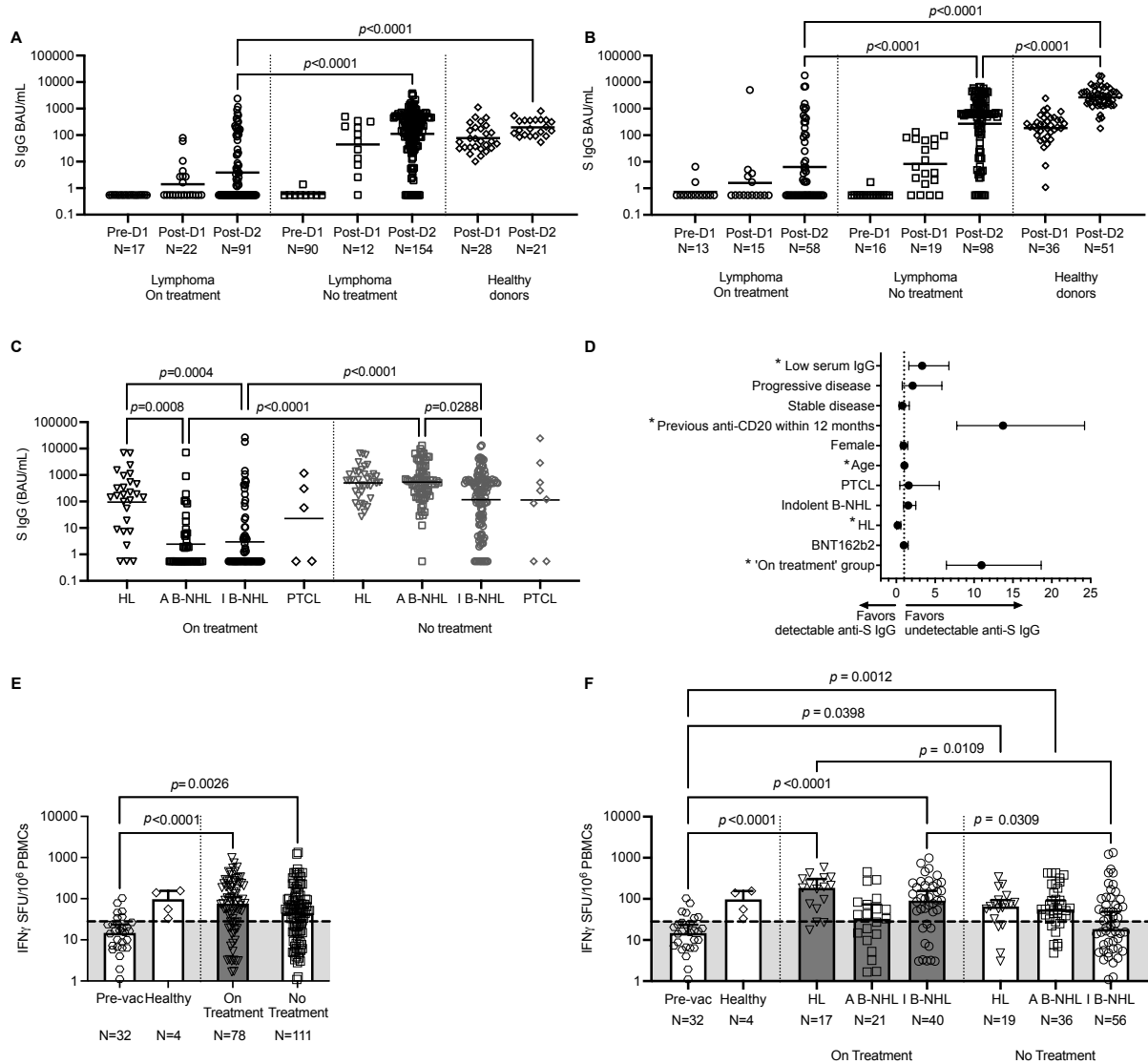
Figure 2. Antibody responses but not cellular responses to SARS-CoV-2 vaccination are impaired by systemic therapy
