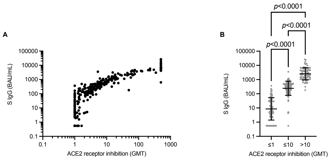
Figure 5. Anti-S level correlates with ACE2 receptor inhibition against WT SARS-CoV-2
