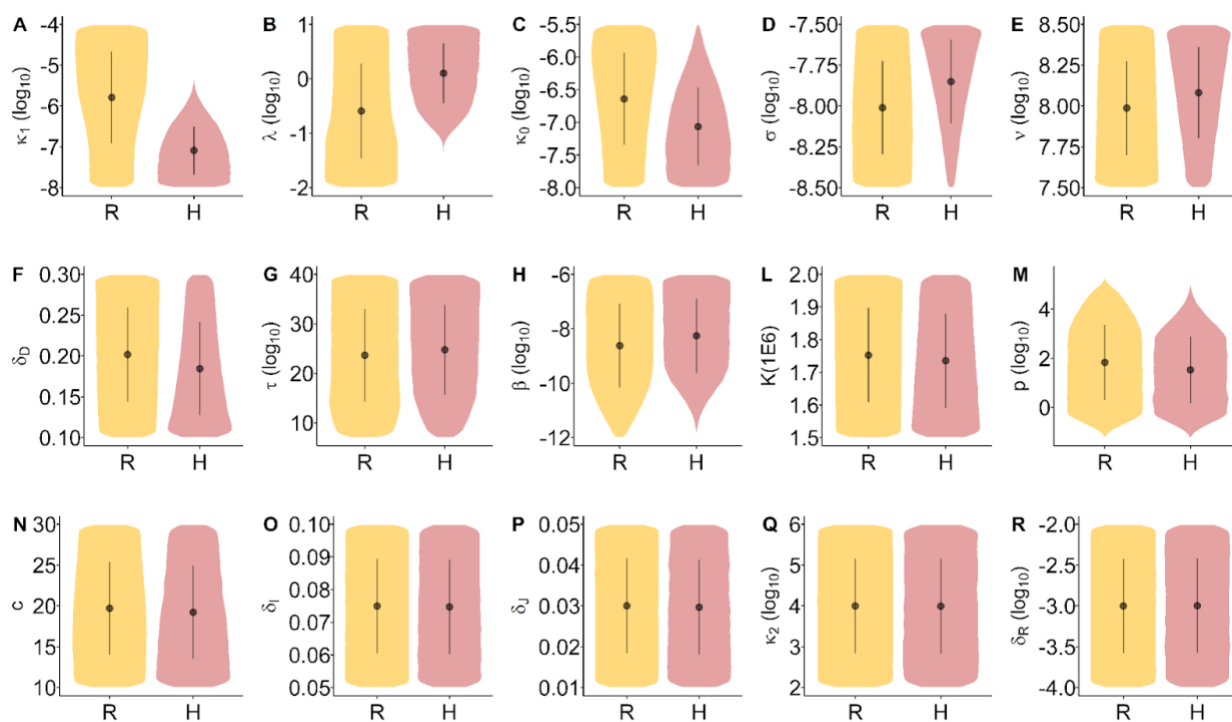
Figure 4. Distribution of the model parameters by inflammation trajectory groups.
