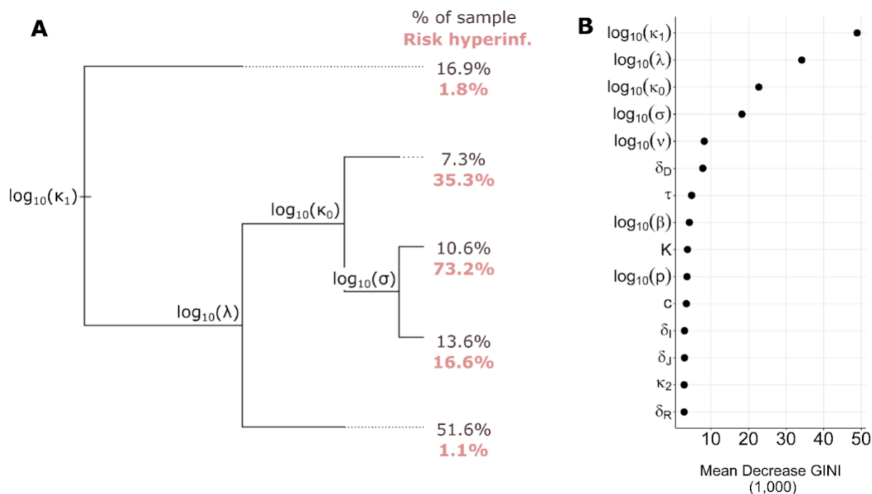
Figure 5. Regression tree analysis results. (A) Single optimal tree for the prediction of hyperinflammation from model parameters. The tree reads from left to right. At each labeled node, simulations either go up if the value for the associated parameter is higher than a threshold determined by the procedure (threshold not shown, see Supplementary Figure S7), or down otherwise. Branch length represents the amount of classification error explained by the node. At each terminal node, the percentage of simulations as well as the risk of hyperinflammation within members of the node are reported. (B): Parameter importance based on the GINI index. A greater mean GINI decrease indicates a parameter that is more discriminatory.
