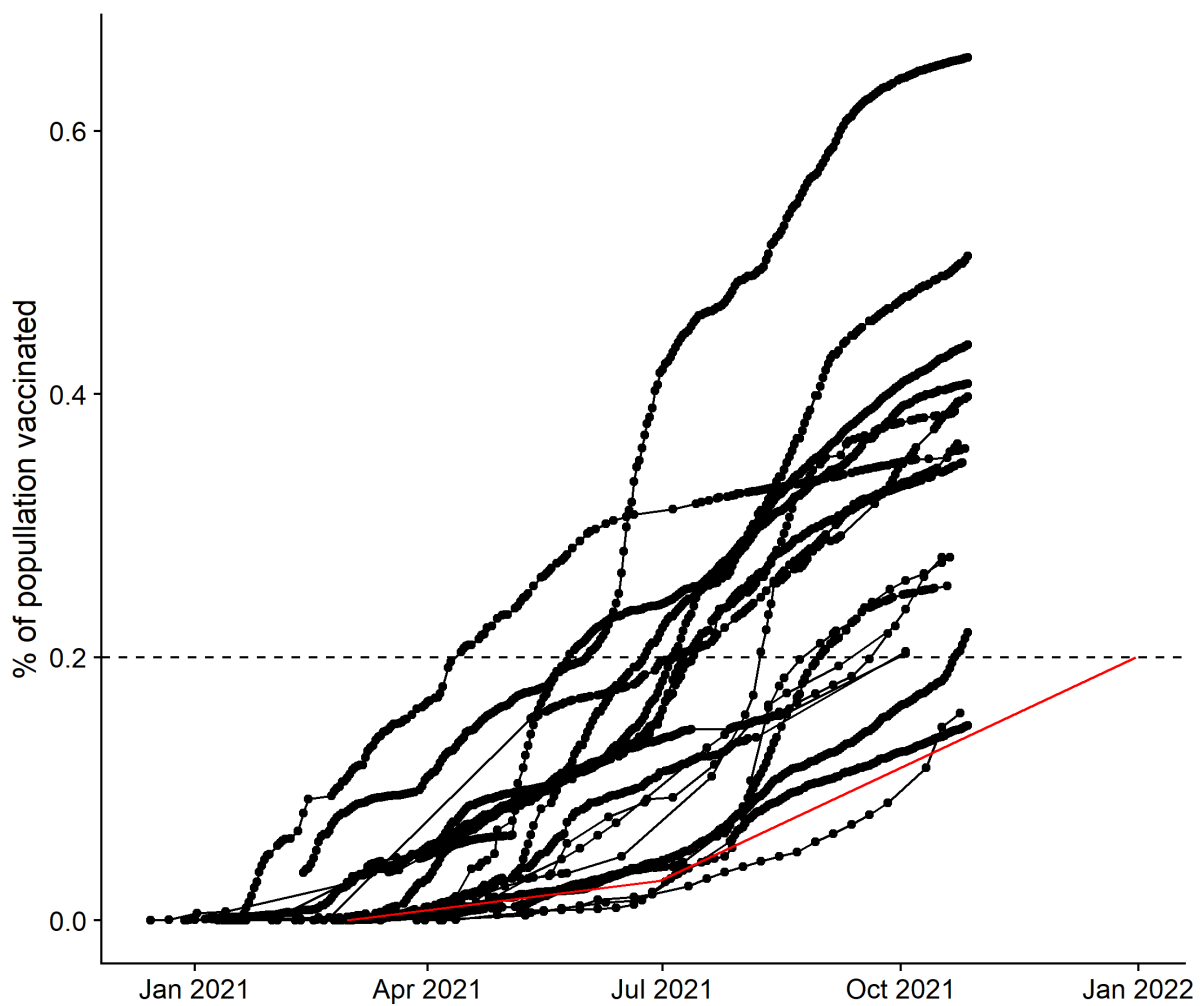
Caption: Each black dotted line represents a country; the red line represents the vaccine rollout strategy investigated in this study. Compared to the rest of the world, LMICs within the WHO European Region are relatively well off. We chose the slowest adaptor within the Region to resemble the slow vaccine row-out conditions that LMICs elsewhere in the world may face.
