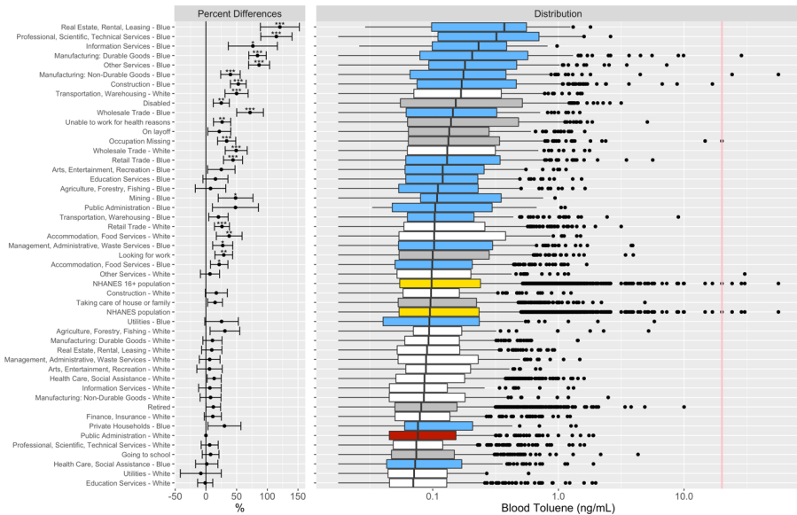
Figure S6. Box plot of distribution of toluene in blood. The “NHANES Population” consists of participants in 1999-2014. The “NHANES 16+ Population” consists of participants in 1999-2014 and are 16 years old or older. Percent differences are derived from fully adjusted models, which were adjusted for age, sex, race/ethnicity, poverty income ratio, study period, and serum cotinine (biomarker of smoking). Reference group for the occupational groups is comprised of white collars from Public Administration. Number of asterisks indicate statistical significance of the percent differences: * (p-value \in (0.01, 0.05]), ** (p-value \in (0.001, 0.01]), and *** (p-value \leq 0.001). The p-values corrected for multiple comparison with the Benjamini and Hochberg FDR procedure of 5%.
