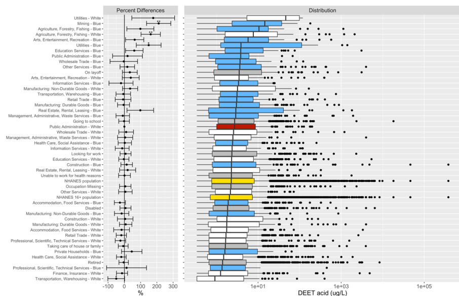
Figure S9. Box plot of distribution of DEET acid in urine. The “NHANES Population” consists of participants in 1999-2014. The “NHANES 16+ Population” consists of participants in 1999-2014 and are 16 years old or older. Percent differences are derived from fully adjusted models, which were adjusted for age, sex, race/ethnicity, poverty income ratio, study period, and serum cotinine (biomarker of smoking). Reference group for the occupational groups is comprised of white collars from Public Administration. Number of asterisks indicate statistical significance of the percent differences: * (p-value \in (0.01, 0.05]), ** (p-value \in (0.001, 0.01]), and *** (p-value \leq 0.001). The p-values corrected for multiple comparison with the Benjamini and Hochberg FDR procedure of 5%.
