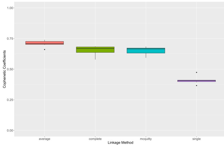
Figure S3. Boxplot of cophenetic correlation coefficients by linkage methods for clustering the occupational groups based on chemical exposure profiles. A cophenetic coefficient is calculated for each stepwise regression models with log10-transformed chemical biomarker levels as the outcome variable and the main predictor as the occupational groups. Covariates include age (continuous), sex (categorical), race (categorical), poverty income ratio (continuous), NHANES cycle (continuous), and smoking with serum cotinine levels (continuous).
