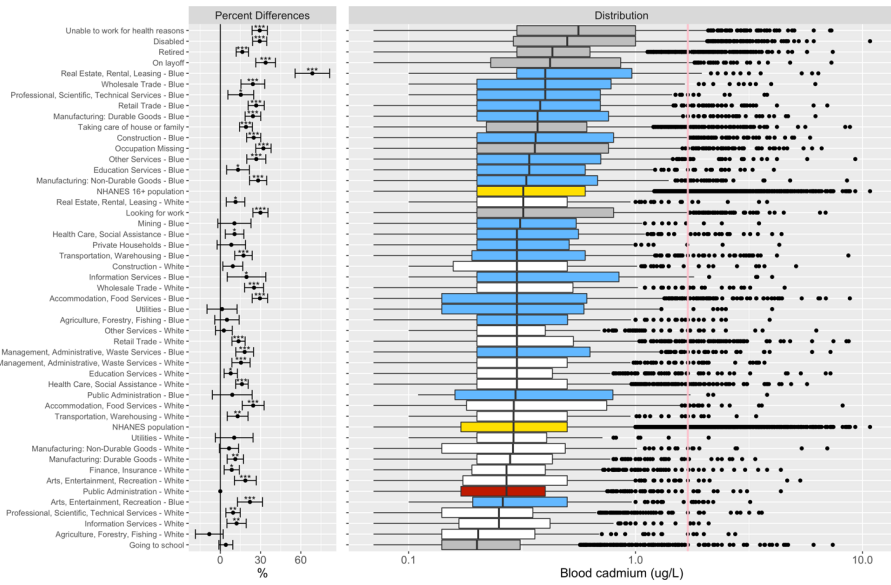
Figure S4. Box plot of distribution of blood cadmium. The “NHANES Population” consists of participants in 1999-2014. The “NHANES 16+ Population” consists of participants in 1999-2014 and are 16 years old or older. Percent differences are derived from fully adjusted models, which were adjusted for age, sex, race/ethnicity, poverty income ratio, study period, and serum cotinine (biomarker of smoking). Reference group for the occupational groups is comprised of white collars from Public Administration. Number of asterisks indicate statistical significance of the percent differences: * (p-value \in (0.01, 0.05]), ** (p-value \in (0.001, 0.01]), and *** (p-value \leq 0.001). The p-values corrected for multiple comparison with the Benjamini and Hochberg FDR procedure of 5%.
