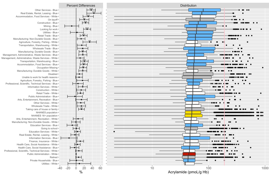
Figure S10. Box plot of distribution of acrylamide in urine. The “NHANES Population” consists of participants in 1999-2014. The “NHANES 16+ Population” consists of participants in 1999-2014 and are 16 years old or older. Percent differences are derived from fully adjusted models, which were adjusted for age, sex, race/ethnicity, poverty income ratio, study period, and serum cotinine (biomarker of smoking). Reference group for the occupational groups is comprised of white collars from Public Administration. Number of asterisks indicate statistical significance of the percent differences: * (p-value \in (0.01, 0.05]), ** (p-value \in (0.001, 0.01]), and *** (p-value \leq 0.001). The p-values corrected for multiple comparison with the Benjamini and Hochberg FDR procedure of 5%.
