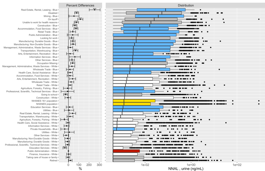
Figure S8. Box plot of distribution of NNAL in urine. The “NHANES Population” consists of participants in 1999-2014. The “NHANES 16+ Population” consists of participants in 1999-2014 and are 16 years old or older. Percent differences are derived from fully adjusted models, which were adjusted for age, sex, race/ethnicity, poverty income ratio, and study period. Reference group for the occupational groups is comprised of white collars from Public Administration. Number of asterisks indicate statistical significance of the percent differences: * (p-value \in (0.01, 0.05]), ** (p-value \in (0.001, 0.01]), and *** (p-value \leq 0.001). The p-values corrected for multiple comparison with the Benjamini and Hochberg FDR procedure of 5%.
