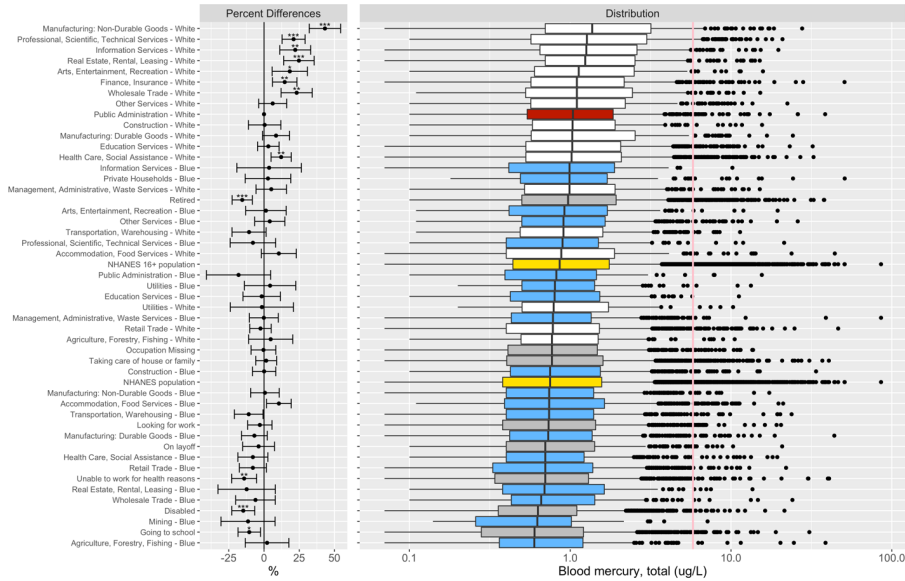
Figure S5. Box plot of distribution of total mercury in blood. The “NHANES Population” consists of participants in 1999-2014. The “NHANES 16+ Population” consists of participants in 1999-2014 and are 16 years old or older. Percent differences are derived from fully adjusted models, which were adjusted for age, sex, race/ethnicity, poverty income ratio, study period, and serum cotinine (biomarker of smoking). Reference group for the occupational groups is comprised of white collars from Public Administration. Number of asterisks indicate statistical significance of the percent differences: * (p-value \in (0.01, 0.05]), ** (p-value \in (0.001, 0.01]), and *** (p-value \leq 0.001). The p-values corrected for multiple comparison with the Benjamini and Hochberg FDR procedure of 5%.
