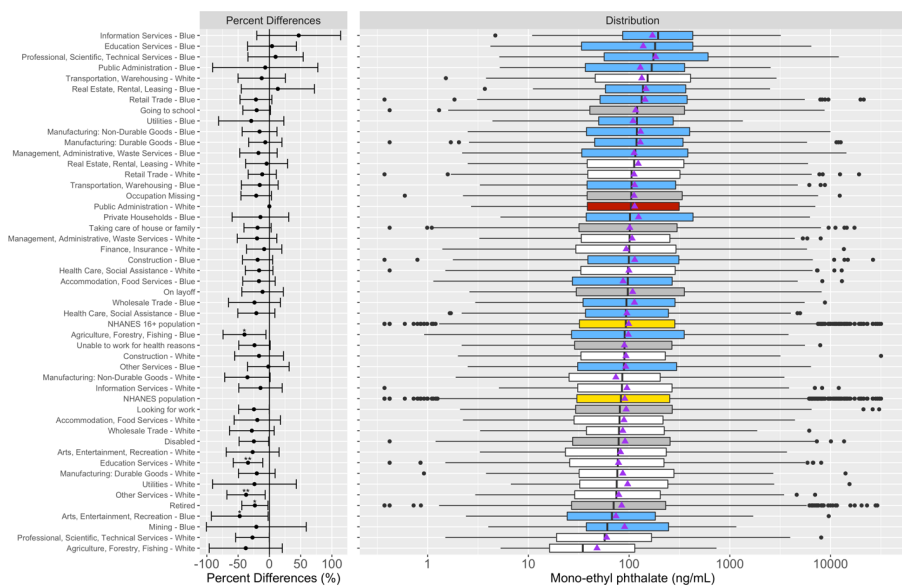
Figure S11. Box plot of distribution of mono-ethyl phthalate in urine. The “NHANES Population” consists of participants in 1999-2014. The “NHANES 16+ Population” consists of participants in 1999-2014 and are 16 years old or older. Percent differences are derived from fully adjusted models, which were adjusted for age, sex, race/ethnicity, poverty income ratio, study period, and serum cotinine (biomarker of smoking). Reference group for the occupational groups is comprised of white collars from Public Administration. Number of asterisks indicate statistical significance of the percent differences: * (p-value \in (0.01, 0.05]), ** (p-value \in (0.001, 0.01]), and *** (p-value \leq 0.001). The p-values corrected for multiple comparison with the Benjamini and Hochberg FDR procedure of 5%.
