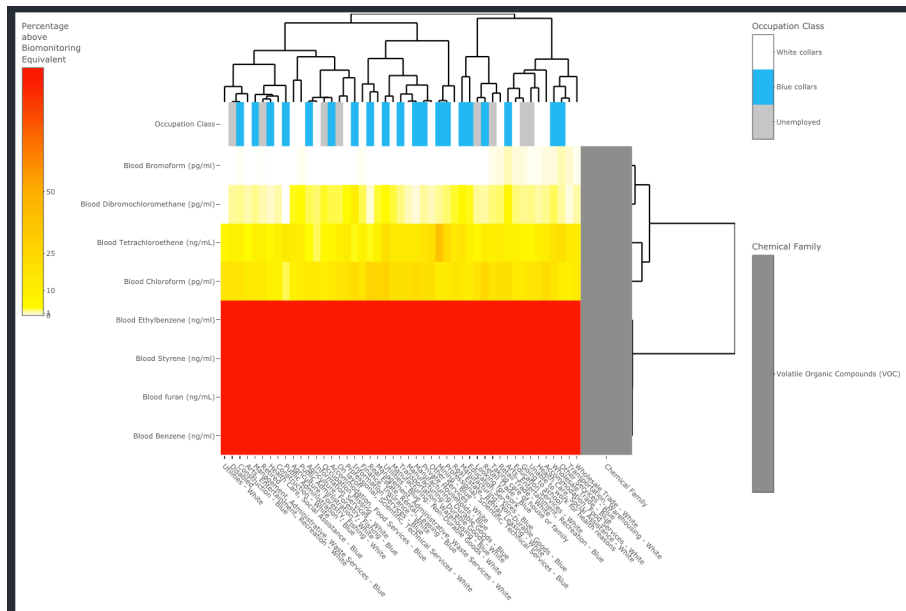
Figure S13. Heatmap of percentages of workers with biomarker levels exceeding biomonitoring equivalents for cancer effects via inhalation. The calculations for the biomonitoring equivalents are based on a 1/10,000 extra risk for cancer.
