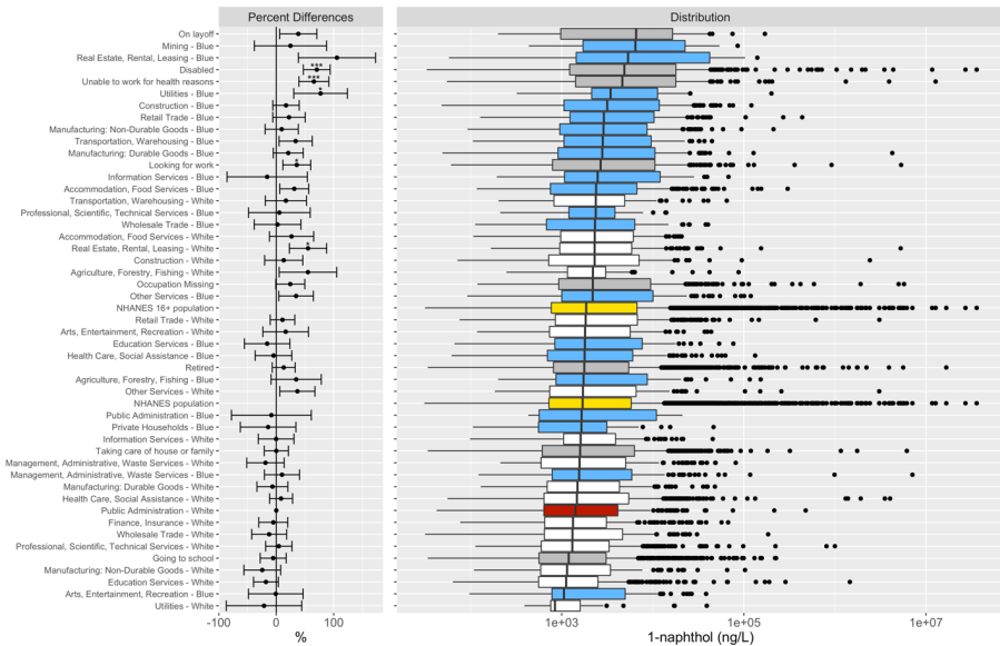
Figure S7. Box plot of distribution of 1-naphthol in blood. The “NHANES Population” consists of participants in 1999-2014. The “NHANES 16+ Population” consists of participants in 1999-2014 and are 16 years old or older. Percent differences are derived from fully adjusted models, which were adjusted for age, sex, race/ethnicity, poverty income ratio, study period, and serum cotinine (biomarker of smoking). Reference group for the occupational groups is comprised of white collars from Public Administration. Number of asterisks indicate statistical significance of the percent differences: * (p-value \in (0.01, 0.05]), ** (p-value \in (0.001, 0.01]), and *** (p-value \leq 0.001). The p-values corrected for multiple comparison with the Benjamini and Hochberg FDR procedure of 5%.
