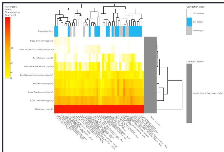
Figure S14. Heatmap of percentages of workers with biomarker levels exceeding biomonitoring equivalents for cancer effects via ingestion. The calculations for the biomonitoring equivalents are based on a 1/10,000 extra risk for cancer.
