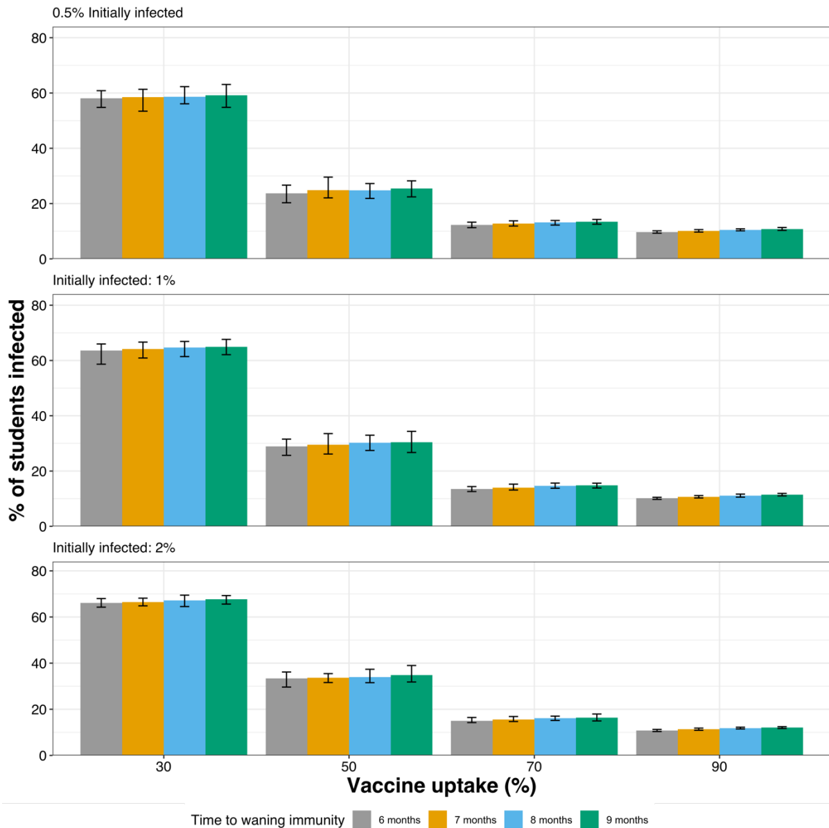
Figure S9. The cumulative percentage of university students infected with SARS-CoV-2 in the Autumn term of 2021 as predicted under different scenarios of waning immunity, vaccine uptake, initially infected students and with 20% students taking part in asymptomatic testing. Each scenario is repeated 50 times, the mean and range are given. The results shown do not include those who were infected but whose immunity has waned by the end of term. Importation from the community was assumed to occur at a time-varying seasonal rate with maximum value of 1e-3 .
