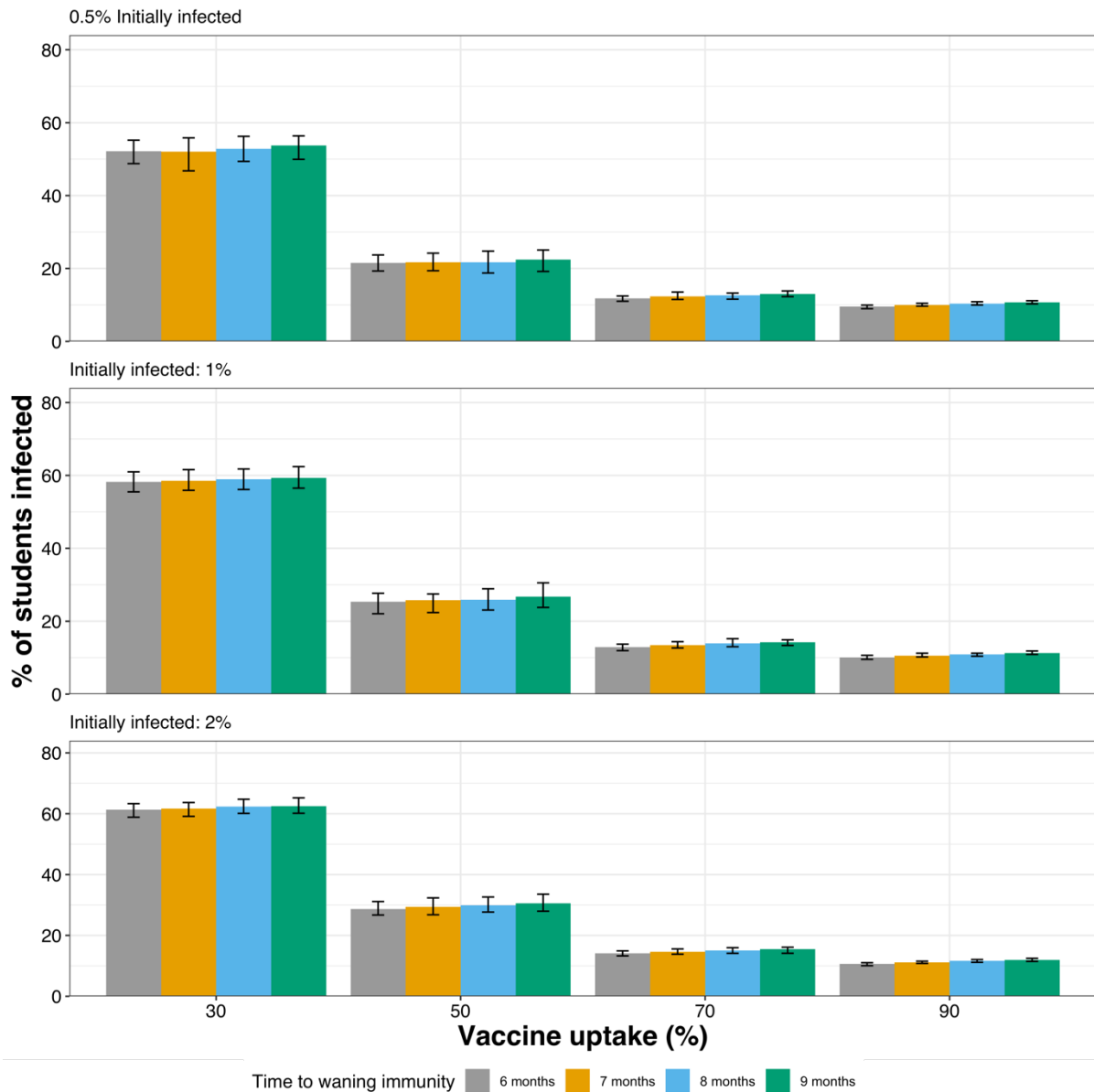
Figure S10. The cumulative percentage of university students infected with SARS-CoV-2 in the Autumn term of 2021 as predicted under different scenarios of waning immunity, vaccine uptake, initially infected students and with 50% students taking part in asymptomatic testing. Each scenario is repeated 50 times, the mean and range are given. The results shown do not include those who were infected but whose immunity has waned by the end of term. Importation from the community was assumed to occur at a time-varying seasonal rate with maximum value of 1e-3 .
