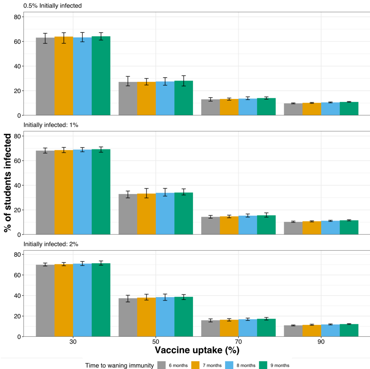
Figure S8. The cumulative percentage of university students infected with SARS-CoV-2 in the Autumn term of 2021 as predicted under different scenarios of waning immunity, vaccine uptake, initially infected students and with no asymptomatic testing. Each scenario is repeated 50 times, the mean and range are given. The results shown do not include those who were infected but whose immunity has waned by the end of term. Importation from the community was assumed to occur at a time-varying seasonal rate with maximum value of 1e-3 .
