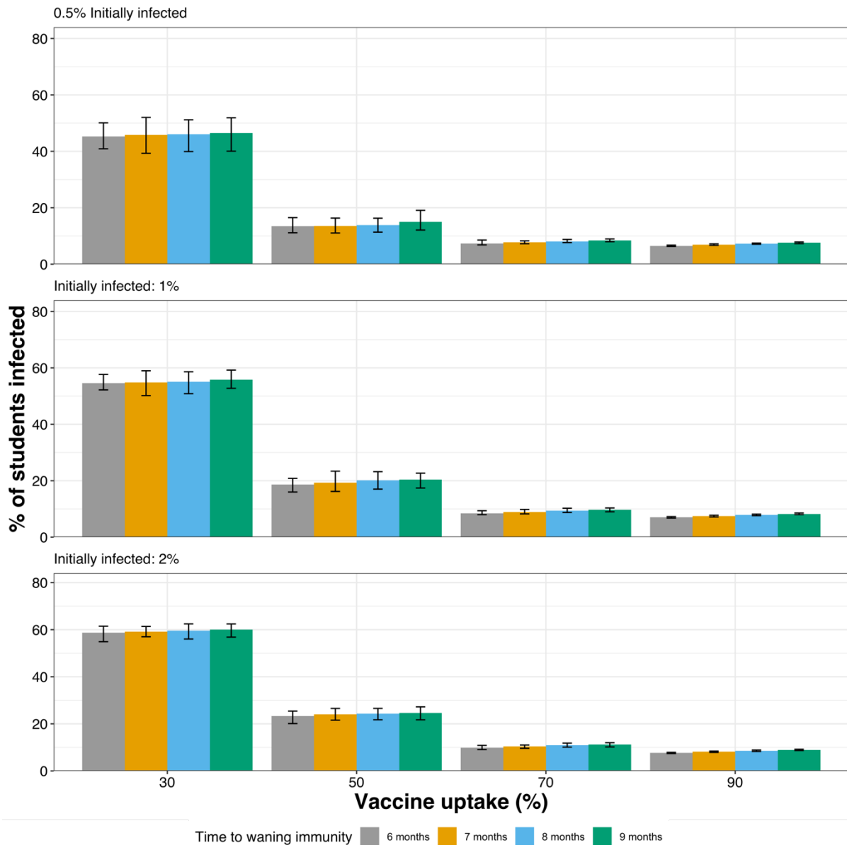
Figure S3. The cumulative percentage of university students infected with SARS-CoV-2 in the Autumn term of 2021 as predicted under different scenarios of waning immunity, vaccine uptake, initially infected students and with 50% students taking part in asymptomatic testing. Each scenario is repeated 50 times, the mean and range are given. The results shown do not include those who were infected but whose immunity has waned by the end of term. It is assumed there is no importation of infection from community.
