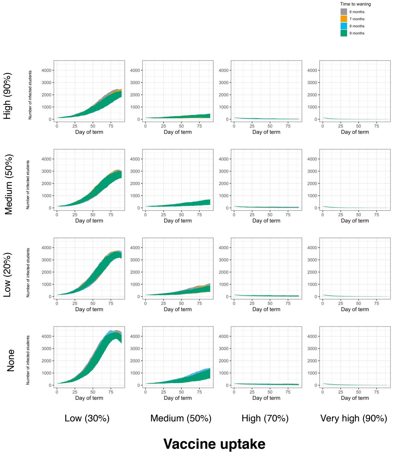
Figure S5. Daily numbers of SARS-CoV-2 infections in a population of students (n=28116) during the autumn term of 2021 as predicted under different scenarios of waning immunity, vaccine uptake, asymptomatic testing and with 0.5% of students initially infected. Each scenario is repeated 50 times and the range is given. It is assumed there is no importation of infection from community.
