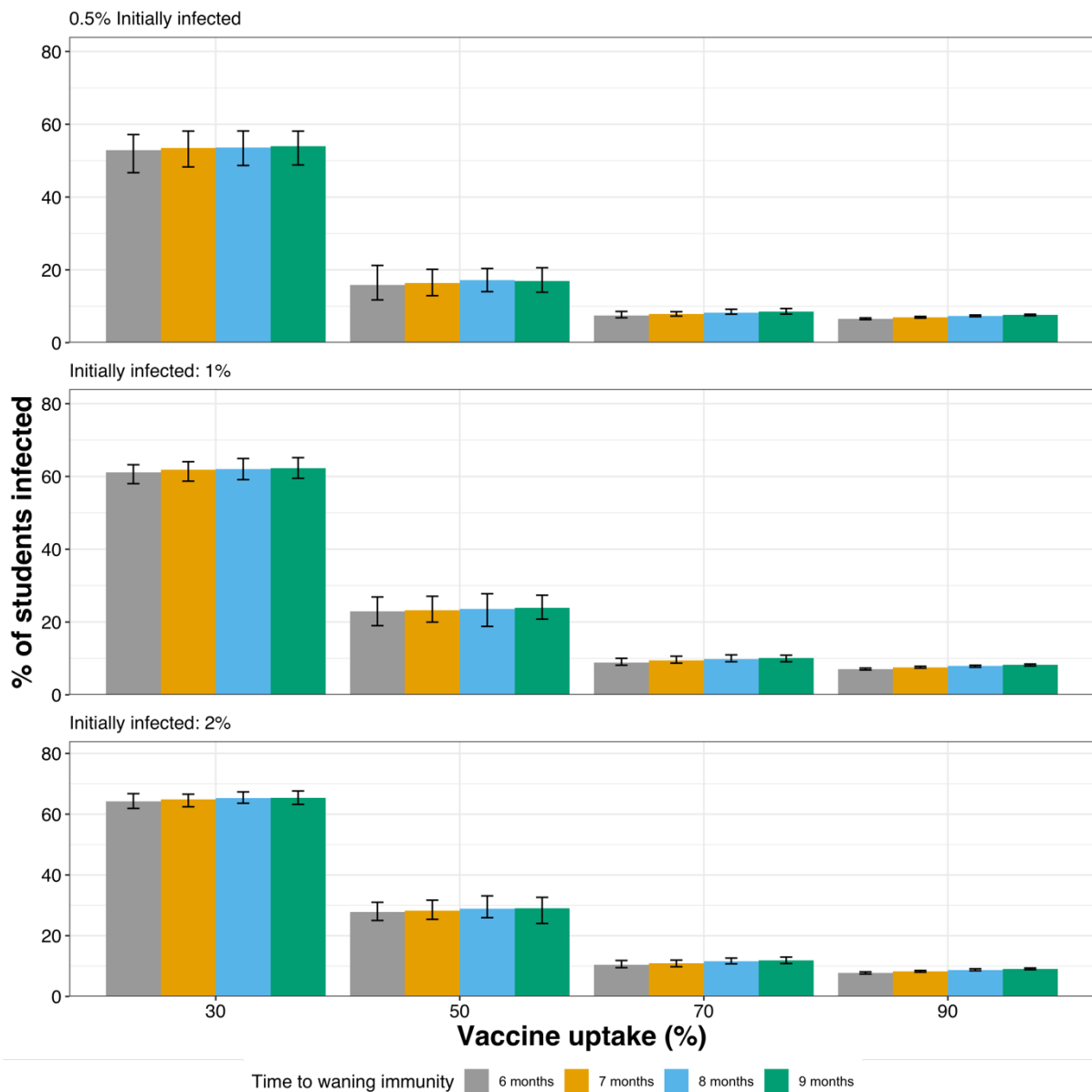
Figure S2. The cumulative percentage of university students infected with SARS-CoV-2 in the Autumn term of 2021 as predicted under different scenarios of waning immunity, vaccine uptake, initially infected students and with 20% students taking part in asymptomatic testing. Each scenario is repeated 50 times, the mean and range are given. The results shown do not include those who were infected but whose immunity has waned by the end of term. It is assumed there is no importation of infection from community.
