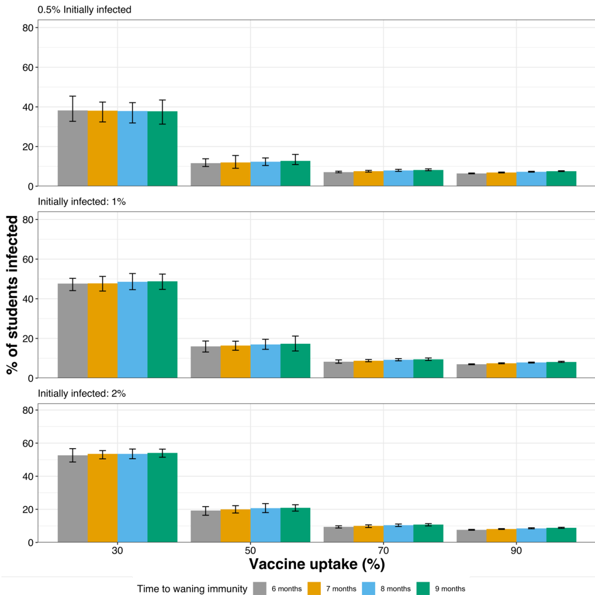
Figure S4. The cumulative percentage of university students infected with SARS-CoV-2 in the Autumn term of 2021 as predicted under different scenarios of waning immunity, vaccine uptake, initially infected students and with 90% students taking part in asymptomatic testing. Each scenario is repeated 50 times, the mean and range are given. The results shown do not include those who were infected but whose immunity has waned by the end of term. It is assumed there is no importation of infection from community.
