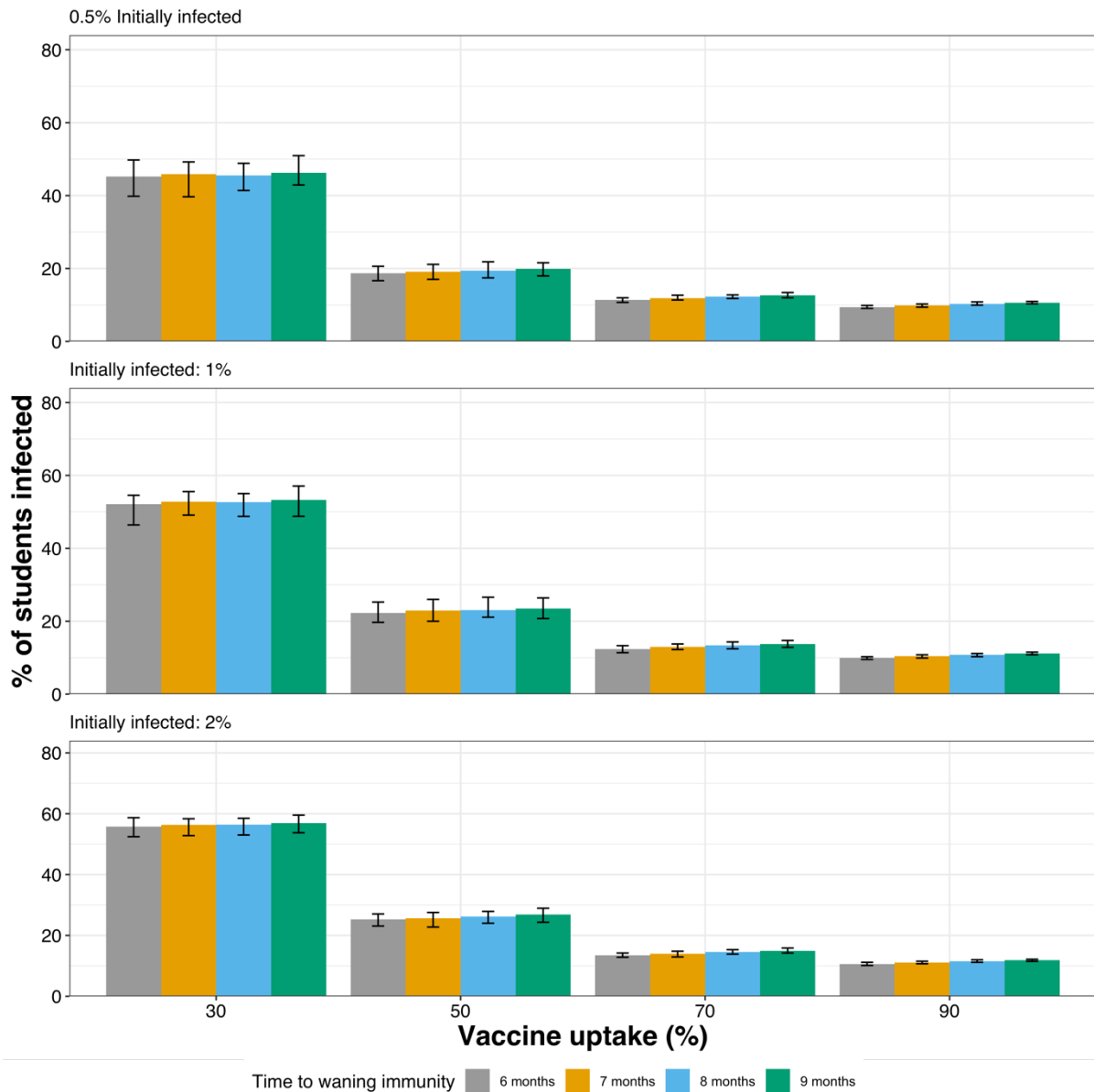
Figure S11. The cumulative percentage of university students infected with SARS-CoV-2 in the Autumn term of 2021 as predicted under different scenarios of waning immunity, vaccine uptake, initially infected students and with 90% students taking part in asymptomatic testing. Each scenario is repeated 50 times, the mean and range are given. The results shown do not include those who were infected but whose immunity has waned by the end of term. Importation from the community was assumed to occur at a time-varying seasonal rate with maximum value of 1e-3 .
