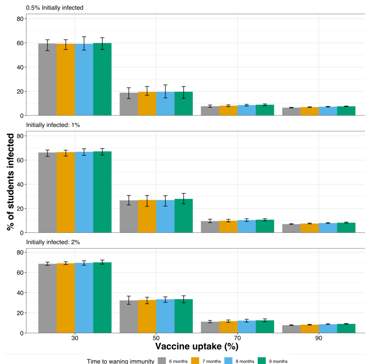
Figure S1. The cumulative percentage of university students infected with SARS-CoV-2 in the Autumn term of 2021 as predicted under different scenarios of waning immunity, vaccine uptake, initially infected students and with no asymptomatic testing. Each scenario is repeated 50 times, the mean and range are given. The results shown do not include those who were infected but whose immunity has waned by the end of term. It is assumed there is no importation of infection from community.
