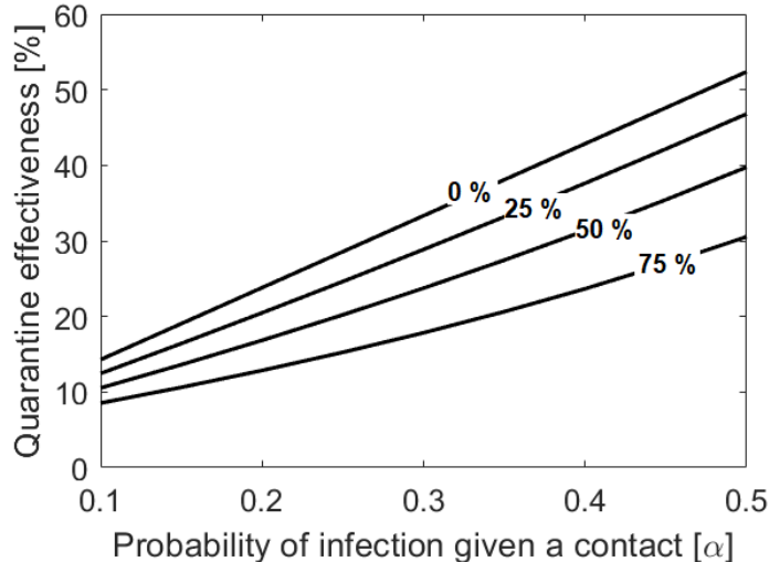
Figure 4: Quarantine effectiveness, defined as the percentage of quarantined individuals that develop an infection, as a function of the probability of infection given a contact ( \alpha ). Different curves represent different vaccination status of the population, where we consider that 0%, 25%, 50% or 75% of the population has been fully vaccinated.
