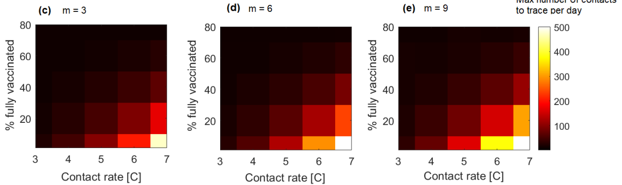
Figure 3: Maximal number of contacts to trace per day as a function of the percentage of fully vaccinated individuals in the population and the contact rate. The number of symptomatic individuals already present in the community when contact tracing is activated ( I_c^* ) is progressively increased from (a) I_c^* = 3 , to (b) I_c^* = 6 , to (c) I_c^* = 9 . In figures (d)-(f) I_c^* = 3 for all simulations, and the number of imported cases m over the time interval considered (i.e., T = 180 days) varies, with (d) m = 3 , (e) m = 6 , and (f) m = 9 . The contact tracing efficiency is kept constant at q = 0.75 .
