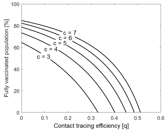
Figure S.1: Analytical approximation of the minimal contact tracing efficiency q^* needed to avoid disease spread, as a function of the vaccination status and for different contact rates. Lines represent equality in Eq. (16), for the contact rates c = \{3, 4, 5, 6, 7\} . Default parameters are given in Table 1.
