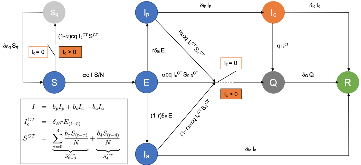
Figure 1: A schematic representation of the flow of individuals among different states in the population as described by equation (9). Susceptible individuals S can become exposed E after having interacted with an infected person, and successively become infectious pre-symptomatic I_p , symptomatic I_c or asymptomatic I_a . Individuals in states represented in blue are not aware of their infectious status and behave normally in the population. Individuals in I_c , represented in orange, can become aware of their status and be contact traced. Once contact tracing is activated (for I_c > 0 , see Eq. (3)) contacts can be moved to quarantine (states in grey), where contacts developing an infection will enter the Q class, and contacts not developing an infection will enter the S_q class. Recovered individuals enter the R status (in green). Delays in outbreak detection are modelled by assuming that contact tracing activates only when I_c > I_c^* , rather than when I_c > 0 (see section 2.4).
