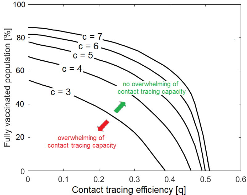
Figure 2: Minimal contact tracing efficiency needed to avoid overwhelming of contact tracing capacity, as a function of the vaccination status of the population and for different contact rates (black curves, with c = \{3, 4, 5, 6, 7\} ), for I_c^* = 0 . The area below each curve represents the parameter space for which contact tracing is overwhelmed, while the area above each curve represents the parameter space for which contact tracing is not overwhelmed. Default parameters used for the simulations are given in Table 1.
