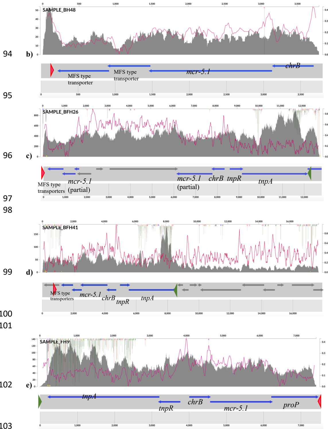
Figure S5: Comparative analysis of contigs that harbor plasmid-mediated mcr-5.1 colistin resistance gene in four different metagenomic samples. Visualizations of the contigs were created using anvio (v7) metagenomics workflow for single profiles 1 . Putative encoding genes are indicated by blue arrows. The gene names were determined based on BLAST search results. The recruited reads are shown as a dark grey histogram with an overlay line (pink) denoting the GC content. Single nucleotide variation is shown on top of the panel with colourful vertical lines. Inverse repeat sequences of Tn3-like transposase sequences (38 bp) are shown with dark pink (IRL: 5' GGGGTCGTCTCAGAAAACGGAAAAAATCGTACGCTAAG 3') and green triangles (IRR: 5'
