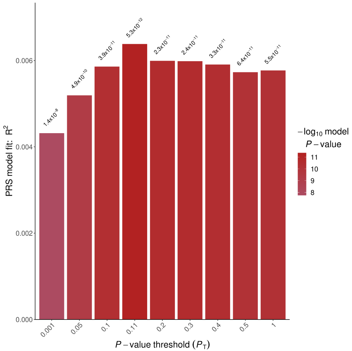
Figure S2: Proportion of variance of alcohol consumption last week explained by PGS ( R^2 ) in the training sample ( N=7,431 ) for different P -value thresholds. P -value threshold = 0.11 generates the best-fit PGS with R^2 = 0.0064 .
