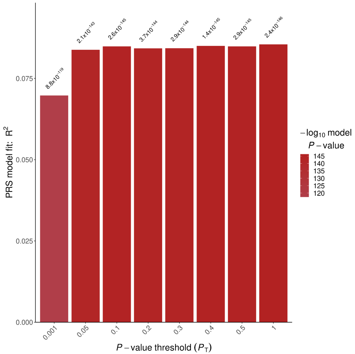
Figure S3: Proportion of variance of BMI explained by PGS ( R^2 ) in the training sample ( N=7,431 ) for different P -value thresholds. P -value threshold = 1 generates the best-fit PGS with R^2 = 0.0855 .
