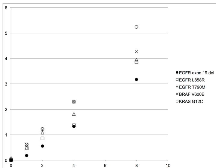
Figure 1. Quantitative ability of DNA module I. Horizontal axis, mutation allele frequency of artificial DNA (%); vertical axis, mutation allele frequency measured with the compact panel (%). Each data point is average of eight samples.
