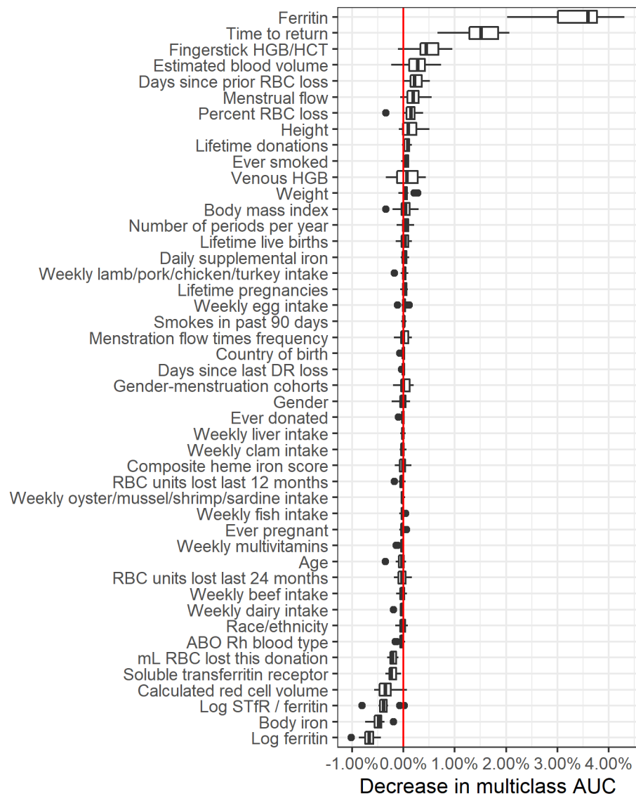
Figure S4: Relative variable importance for the top "extra biomarkers" model.
