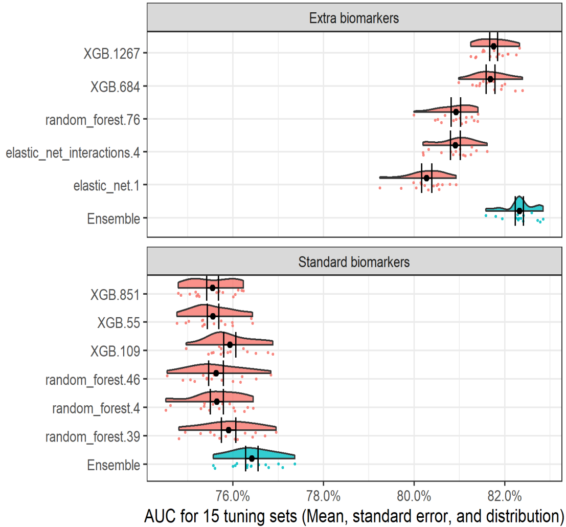
Figure S2: Distribution of multiclass AUC for across the 15 tuning sets for the top ensemble model configurations and the base model configurations that comprised them. For both the ``standard`` and ``extra biomarkers`` versions, the top ensemble was an average of the base models.
