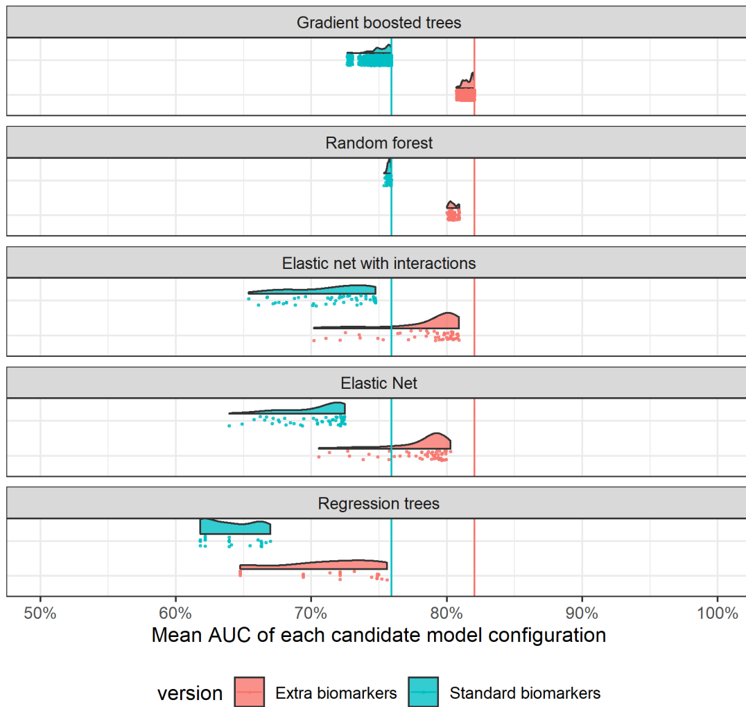
Figure S1: Average multiclass AUC for each evaluated model configuration as assessed using 5-fold cross validation and averaged across 15 tuning sets (excluding ensemble models). Each configuration (model type and hyperparameter set) is plotted as a dot. Distributions for each model type are shown.
