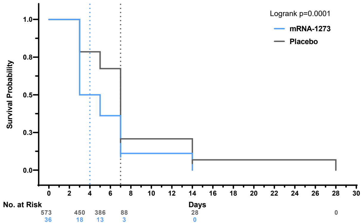
Figure S3. Time to undetectable SARS-CoV-2 viral copies
