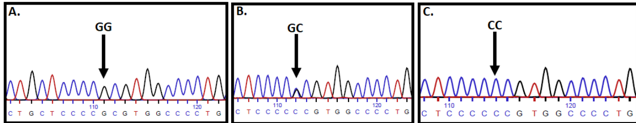
Figure 5: Sanger sequencing displaying TP53 rs1042522 polymorphism indicated by arrow. (A.) Wild type [GG], (B.) Heterozygous [GC], (C.) Variant [CC] sequences.
