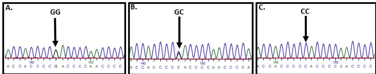
Figure 3: Sanger sequencing displaying TP53 rs1642785 polymorphism indicated by arrow. (A.) Wild type [GG], (B.) Heterozygous [GC], (C.) Variant [CC].
