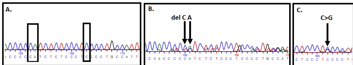
Figure 6: Representative Sanger sequencing displaying (A.) Wild type sequence in 3'UTR, (B.) del CA at chromosome 17:7669567_8 and (C.) C>G at chromosome 17:7669560.
