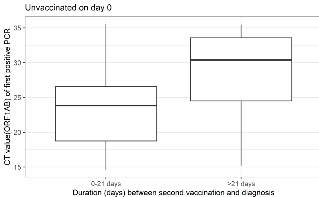
293 Figure 4: Ct-Value (ORF1AB gene) of the first positive PCR by interval between second vaccination 294 and diagnosis during a SARS-CoV-2 Alpha outbreak in a nursing home in Germany, Jan-Mar 2021
